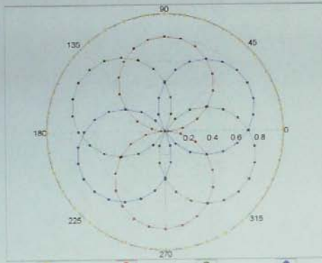
f=600 MHz,TEM
