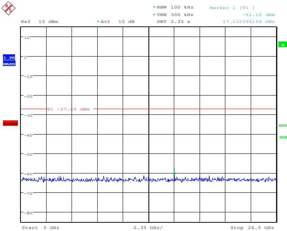
(Plot 4.6.1 B2: Channel 19: 2440MHz @ GFSK)
