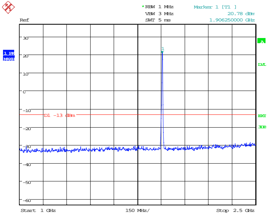
(Plot 4.6.1 C3: Channel 9538: 1907.6MHz @ Traffic WCDMA Band II)
