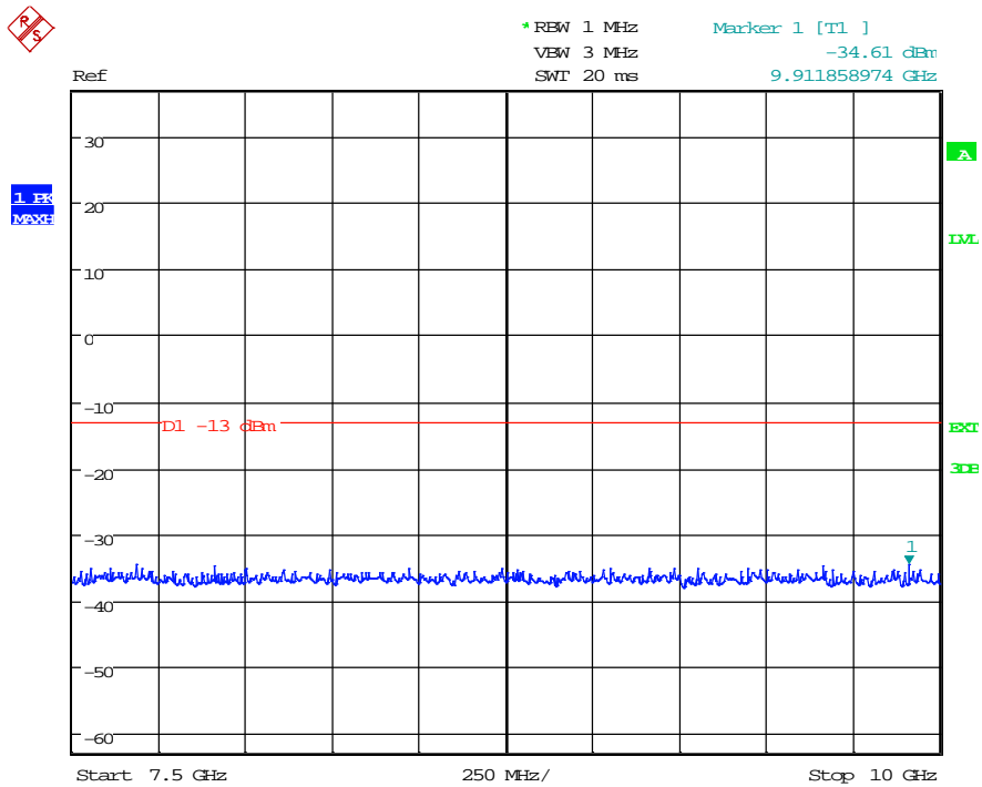
(Plot 4.6.2 B5: Channel 4183: 836.60 MHz @ WCDMA Band V)
