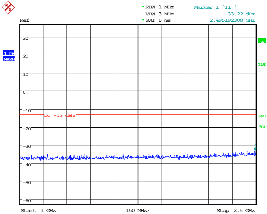
(Plot 4.6.2 A3: Channel 4132: 826.40 MHz @ WCDMA Band V)
