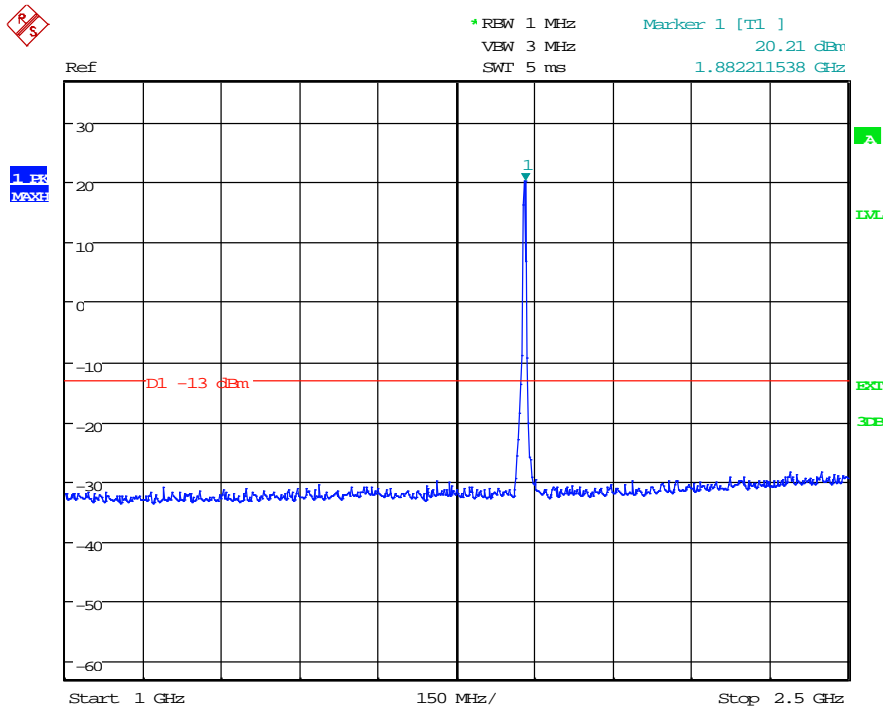
(Plot 4.6.1 B3: Channel 9400: 1880.0MHz @ Traffic WCDMA Band II)
