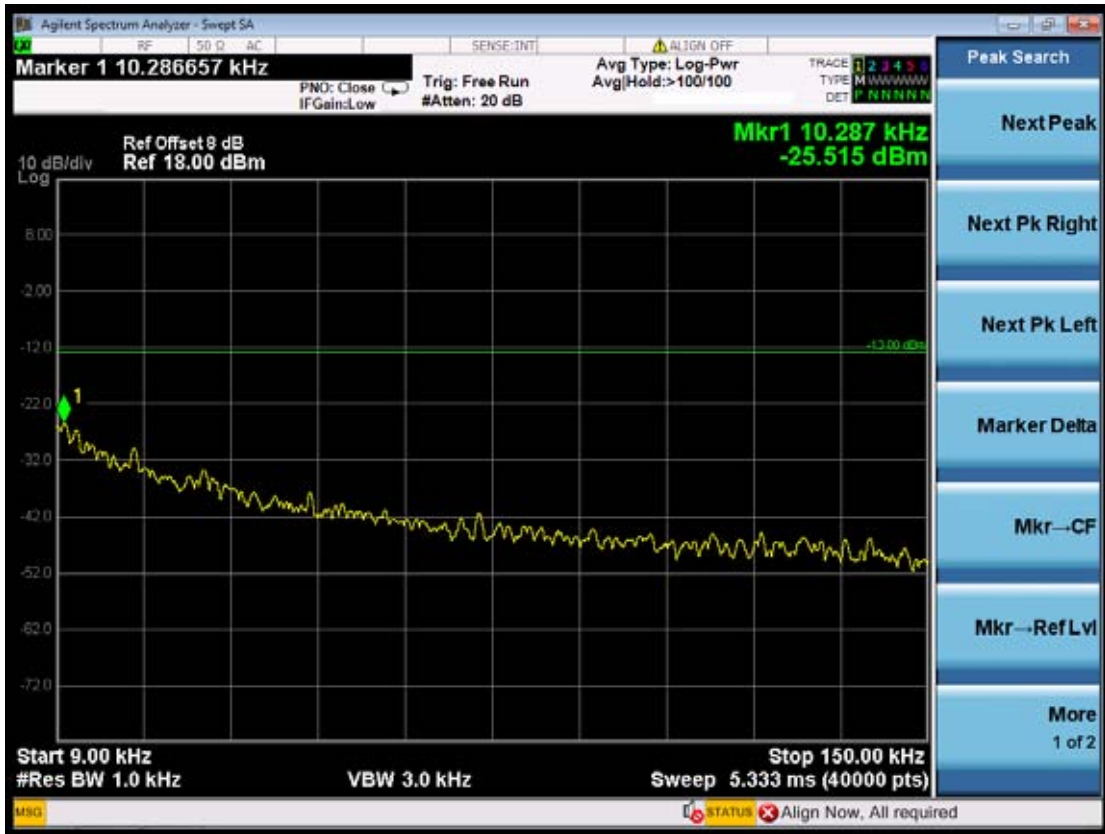
(Plot 4.6.1 D1: Idle WCDMA Band II)
