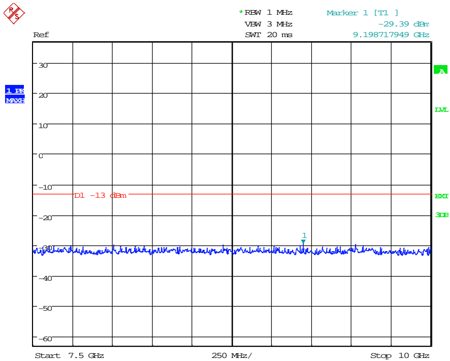
(Plot 4.6.1 A5: Channel 9262: 1852.4MHz @ Traffic WCDMA Band II)
