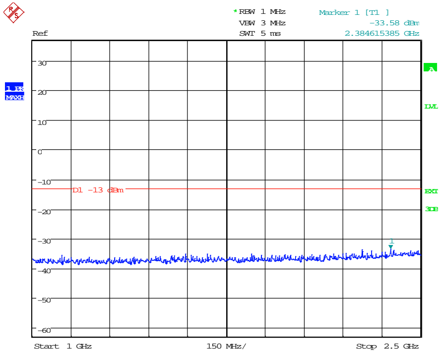
(Plot 4.6.2 B3: Channel 4183: 836.60 MHz @ WCDMA Band V)
