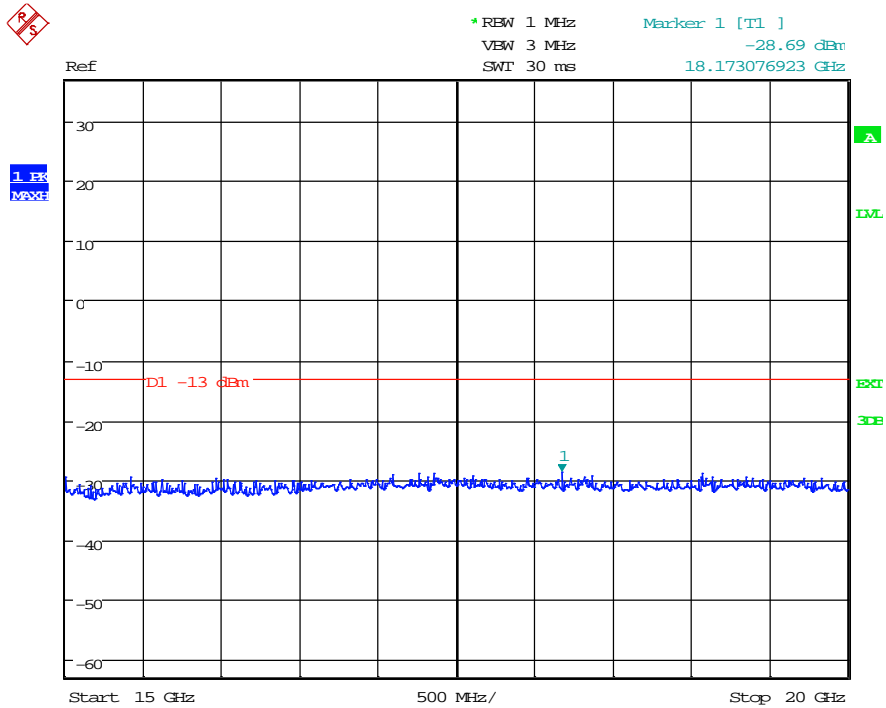
(Plot 4.6.1 C7: Channel 9538: 1907.6MHz @ Traffic WCDMA Band II)
