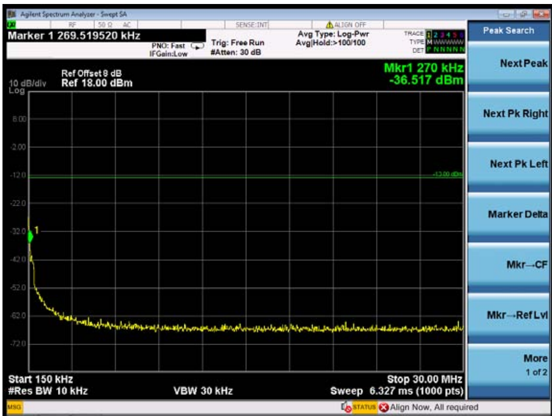
(Plot 4.6.2 D2: Idle @ WCDMA Band V)
