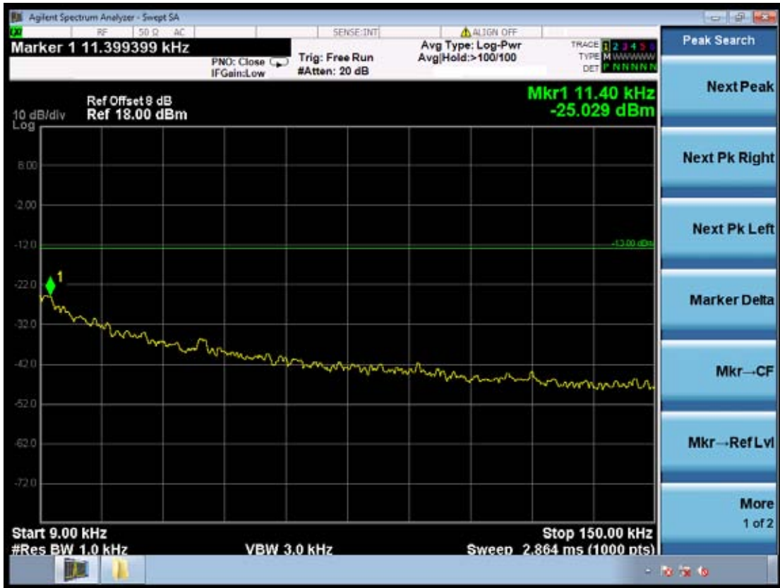
(Plot 4.6.2 D1: Idle @ WCDMA Band V)
