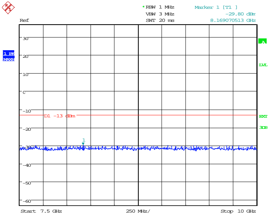
(Plot 4.6.1 C5: Channel 9538: 1907.6MHz @ Traffic WCDMA Band II)
