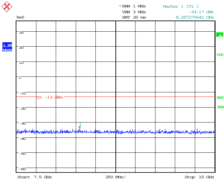
(Plot 4.6.2 C5: Channel 4233: 846.60 MHz @ WCDMA Band V)
