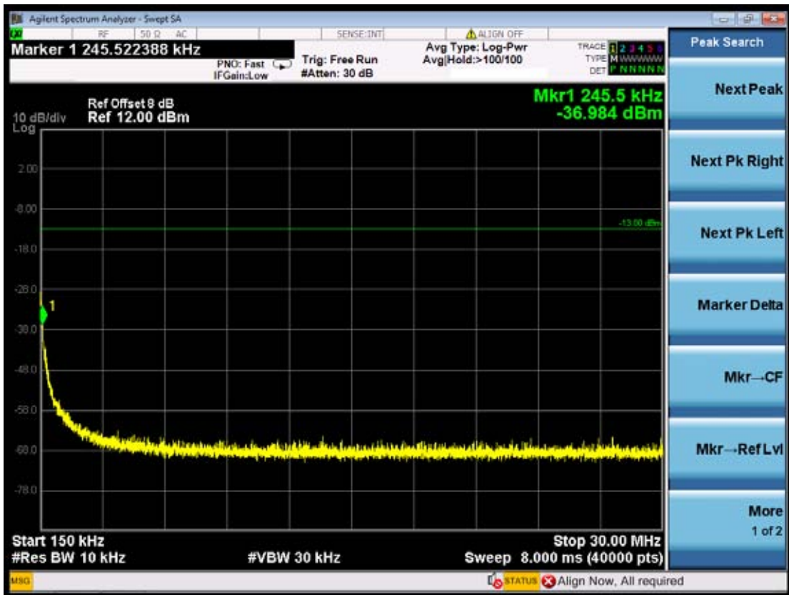
(Plot 4.6.2 A2: Channel 4132: 826.40 MHz @ WCDMA Band V)
