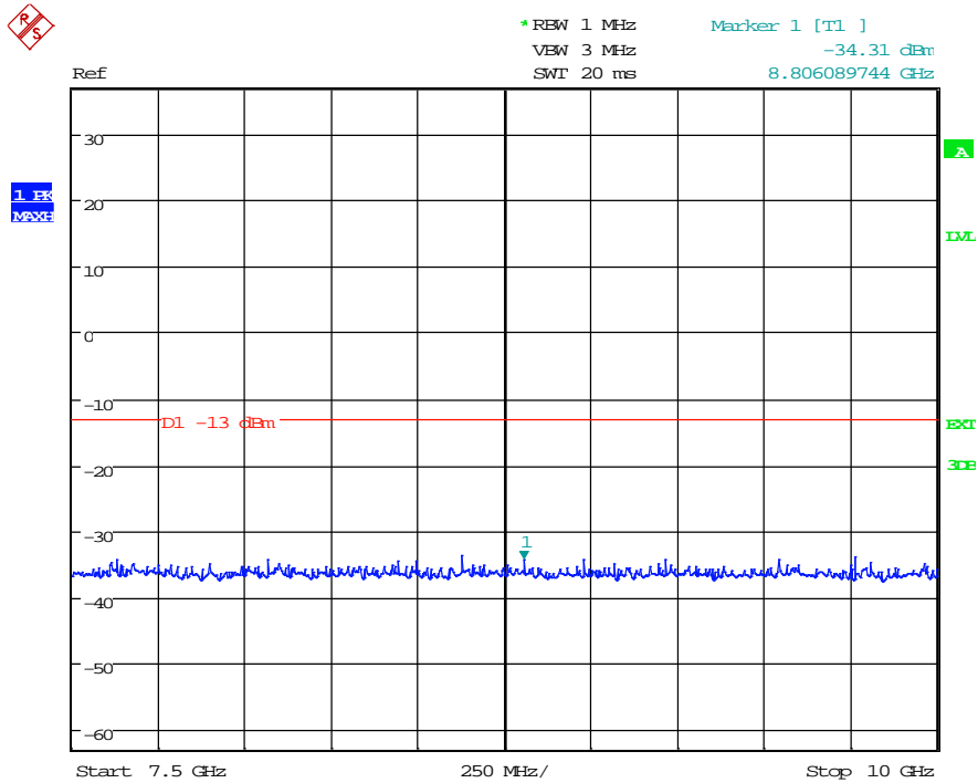
(Plot 4.6.2 A5: Channel 4132: 826.40 MHz @ WCDMA Band V)
