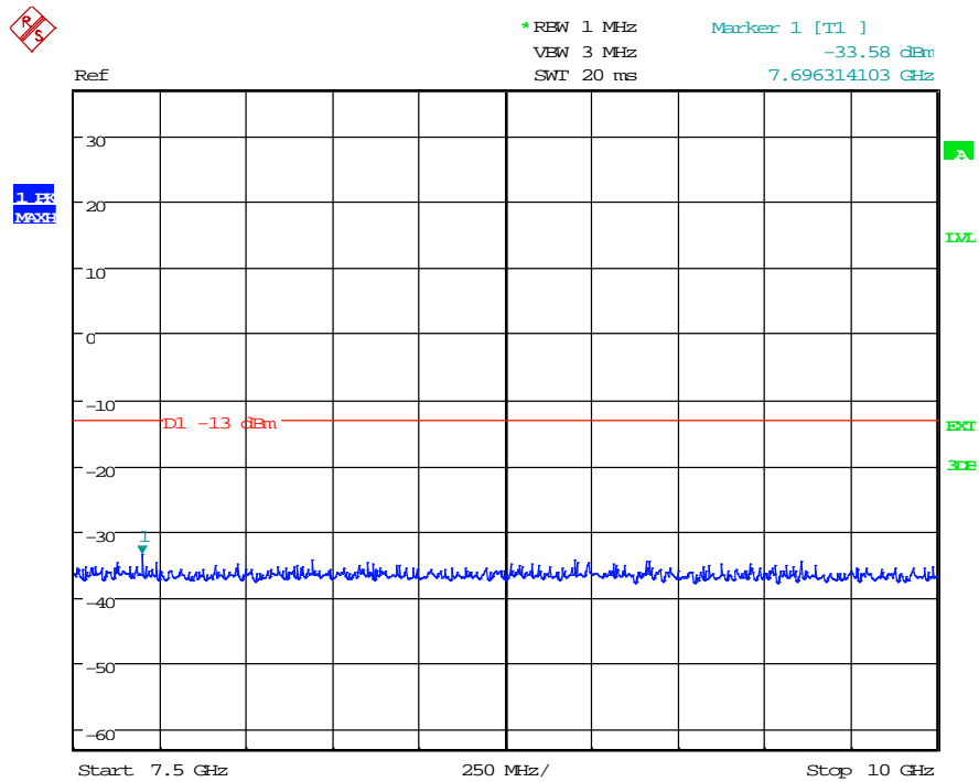
(Plot 4.6.2 D5: Idle @ WCDMA Band V)
