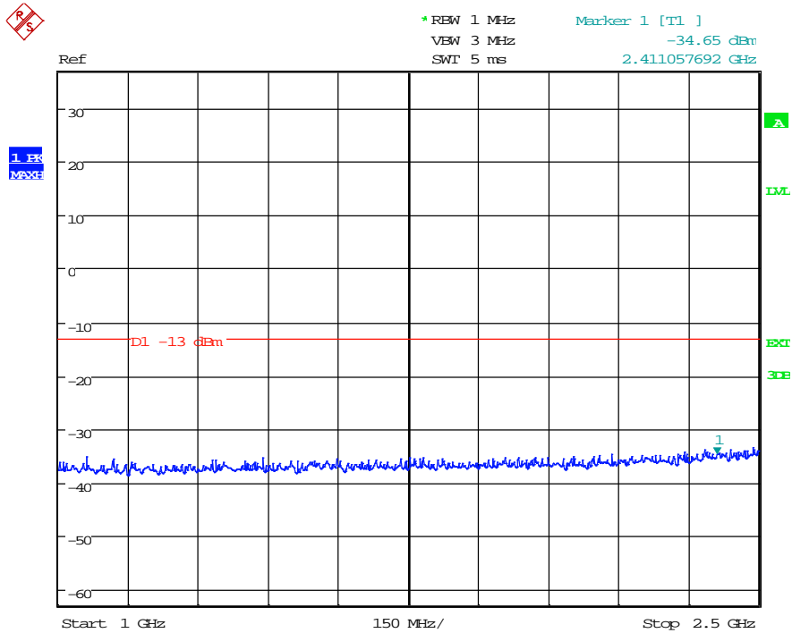
(Plot 4.6.2 C3: Channel 4233: 846.60 MHz @ WCDMA Band V)
