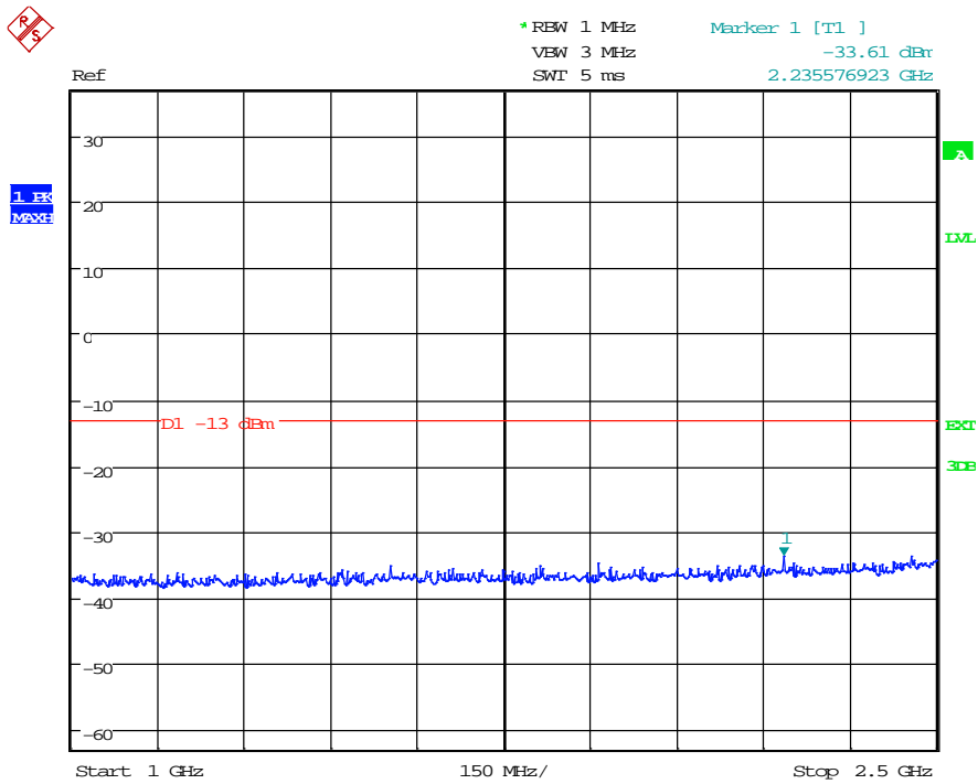
(Plot 4.6.2 D3: Idle @ WCDMA Band V)
