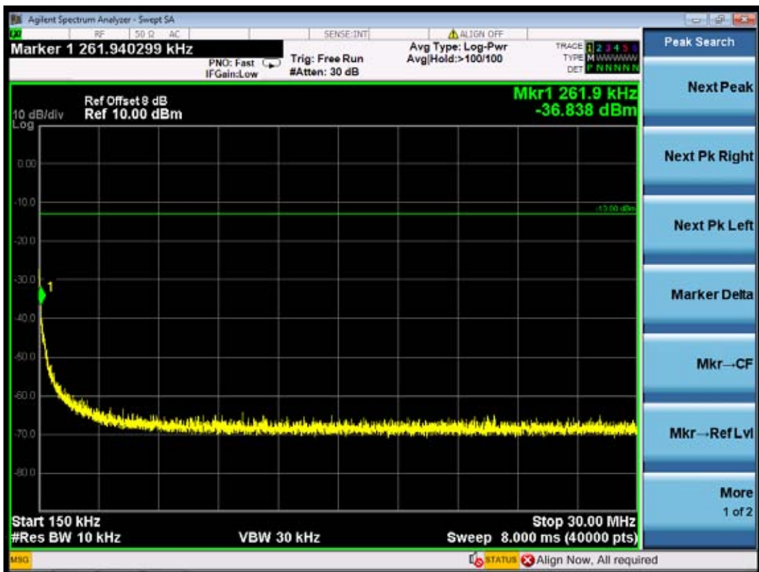
(Plot 4.6.1 C2: Channel 9538: 1907.6MHz @ Traffic WCDMA Band II)
