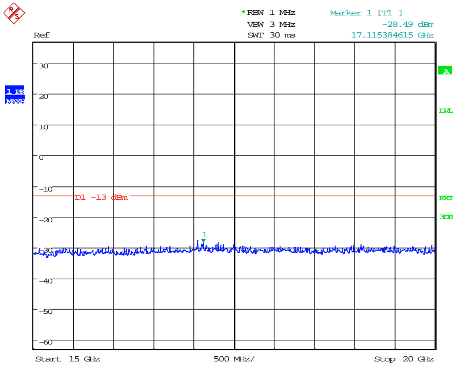
(Plot 4.6.1 A7: Channel 9262: 1852.4MHz @ Traffic WCDMA Band II)
