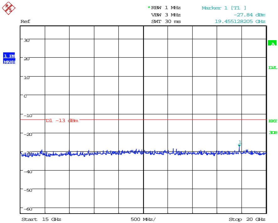
(Plot 4.6.1 B7: Channel 9400: 1880.0MHz @ Traffic WCDMA Band II)
