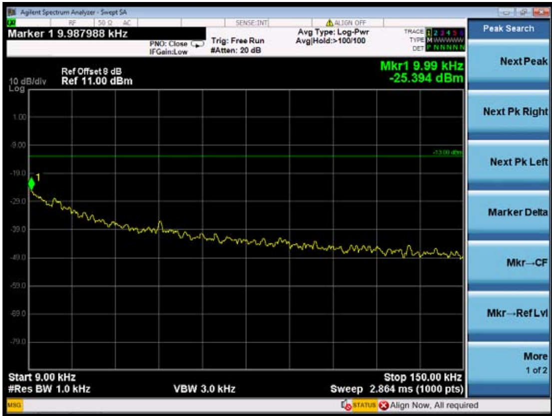
(Plot 4.6.2 A1: Channel 4132: 826.40 MHz @ WCDMA Band V)
