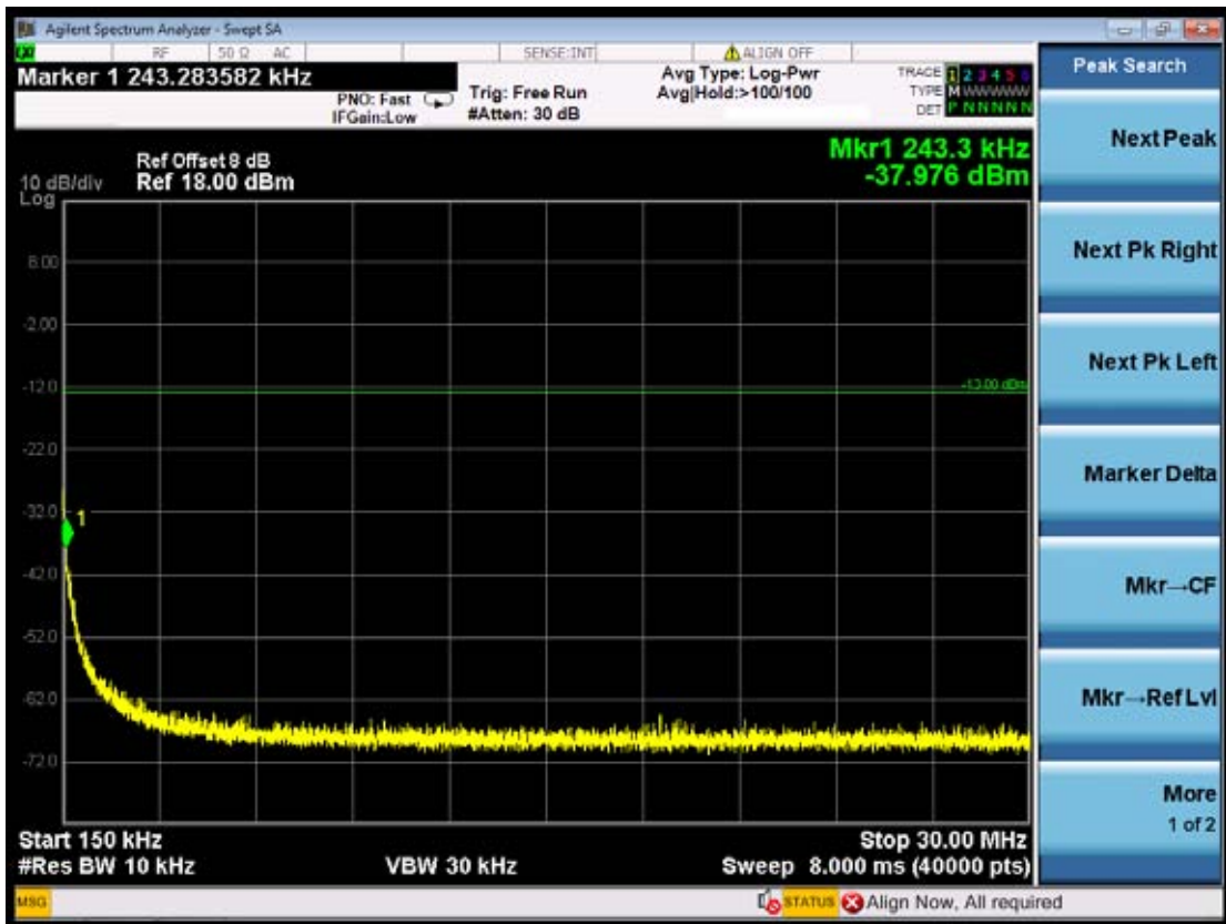
(Plot 4.6.1 D2: Idle WCDMA Band II)
