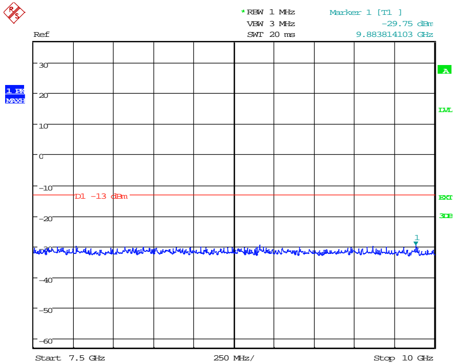
(Plot 4.6.1 B5: Channel 9400: 1880.0MHz @ Traffic WCDMA Band II)
