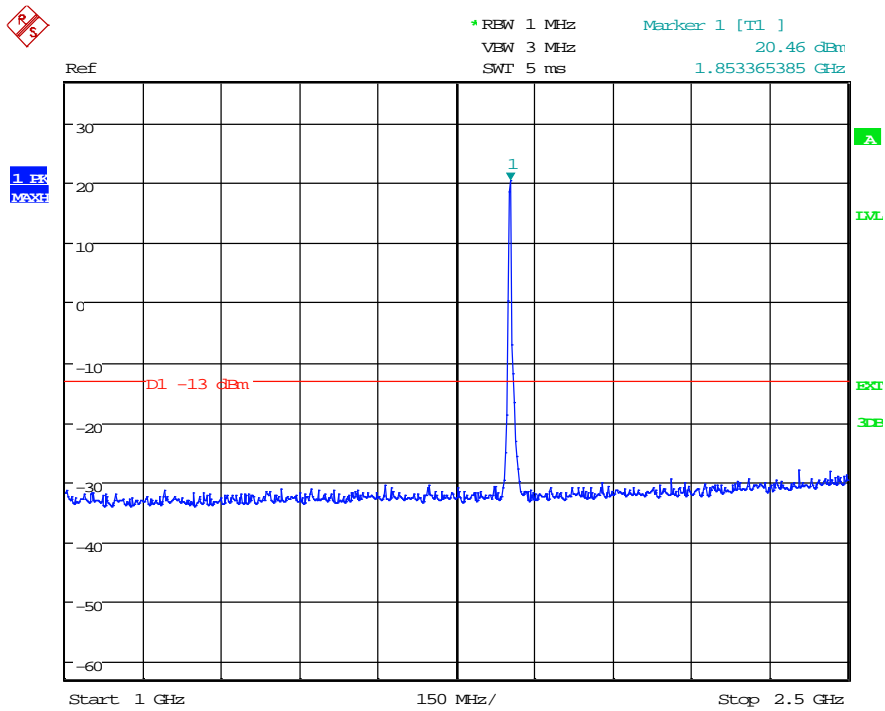
(Plot 4.6.1 A3: Channel 9262: 1852.4MHz @ Traffic WCDMA Band II)
