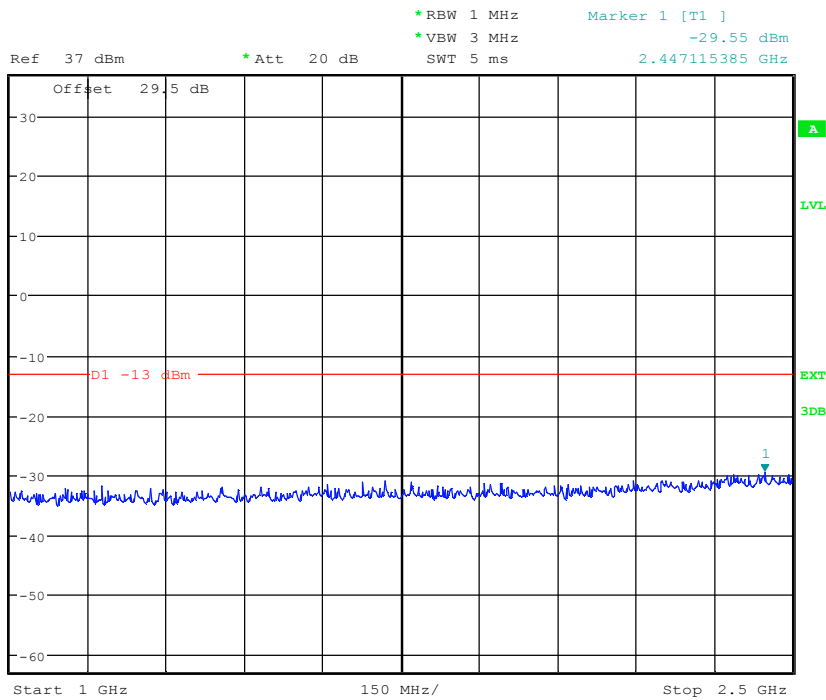
(Plot 4.6.2 D3: Idle @ PCS1900)
