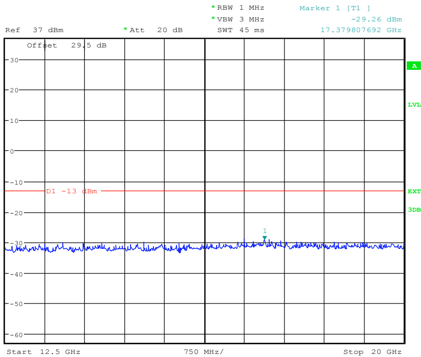
(Plot 4.6.2 B7: Channel 661: 1880.00MHz @ Traffic @ PCS1900)
