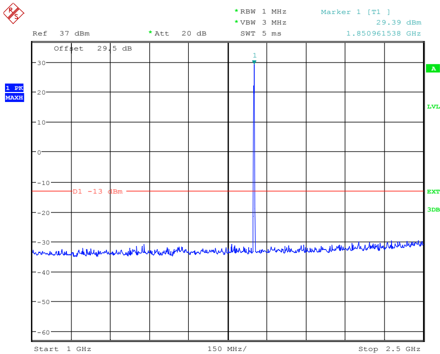
(Plot 4.6.2 A3: Channel 512: 1850.20MHz @ Traffic @ PCS1900)
