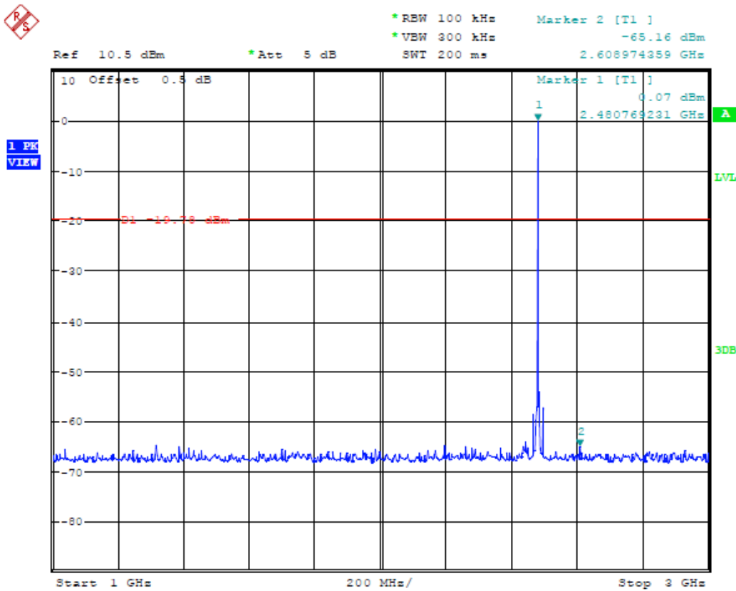
(Plot 4.6.1 C4: Channel 39: 2480MHz @ GFSK)
