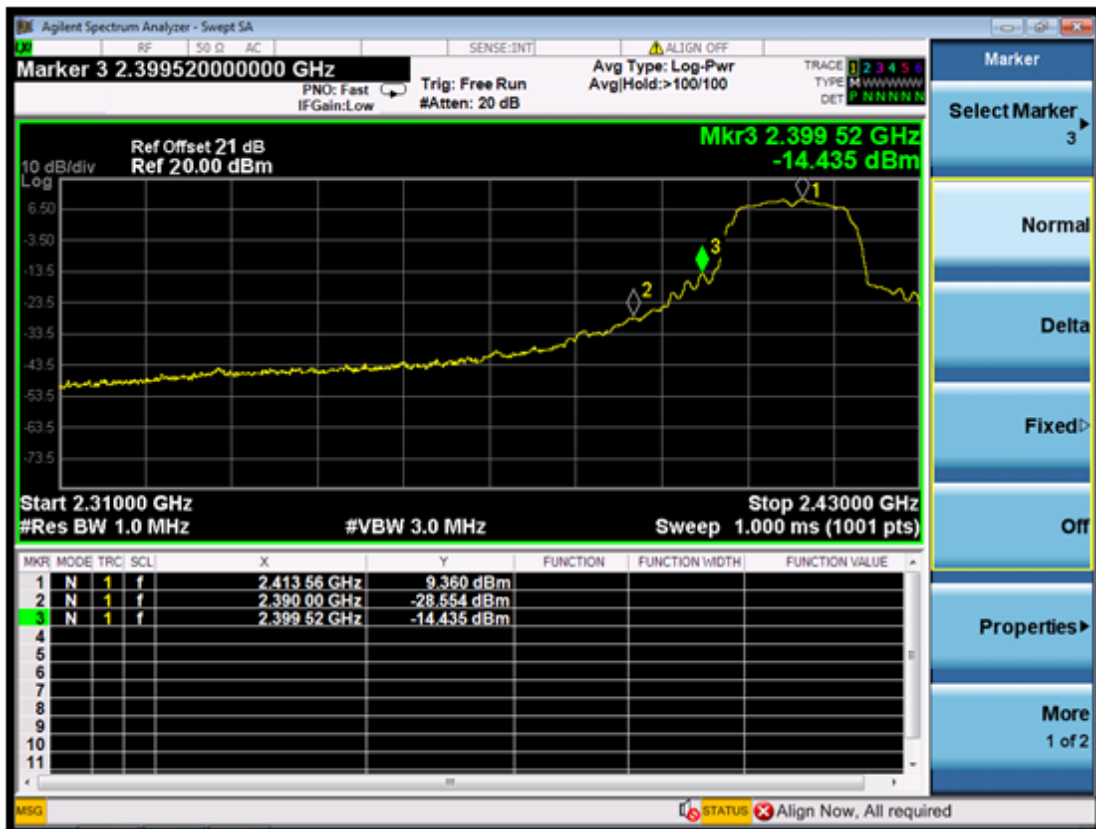
(Plot 4.5.2 A1: Channel 1: 2412MHz @ 802.11g)
