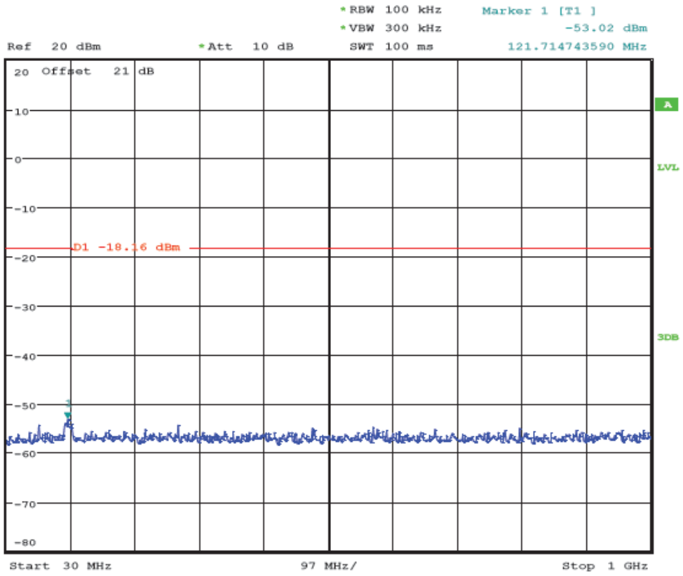
(Plot 4.6.3 B3: Channel 6: 2437MHz @ 802.11n HT20)
