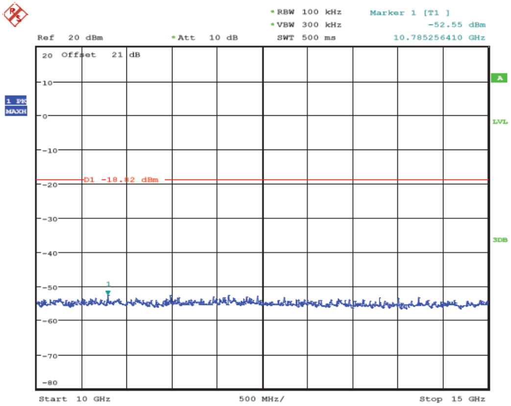
(Plot 4.6.2 A7: Channel 1: 2412MHz @ 802.11g)
