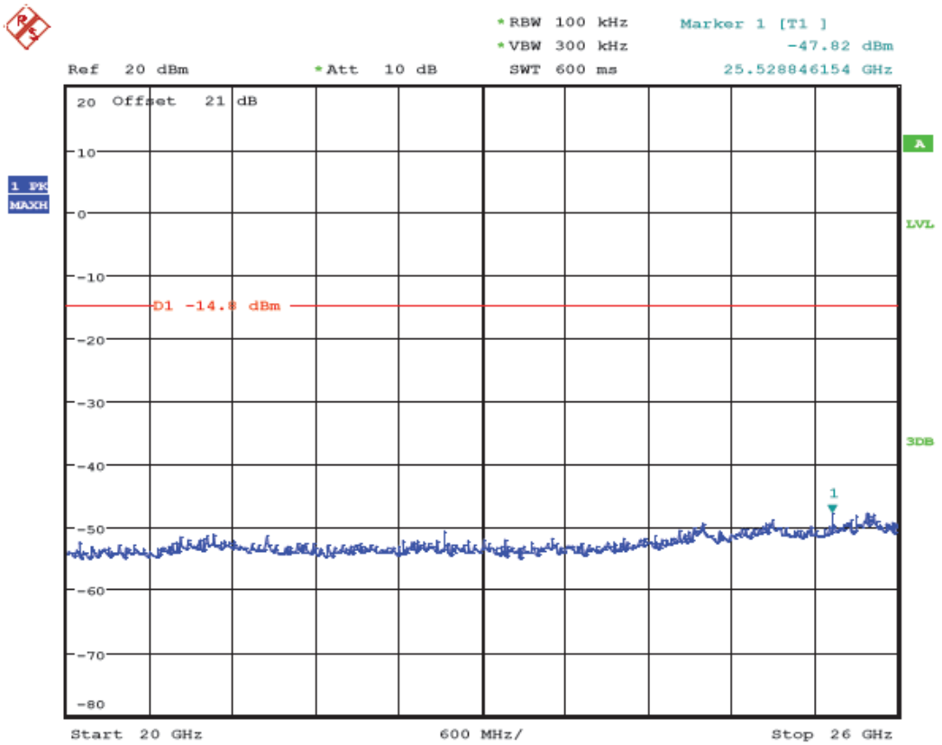
(Plot 4.6.1 A9: Channel 1: 2412MHz @ 802.11b)
