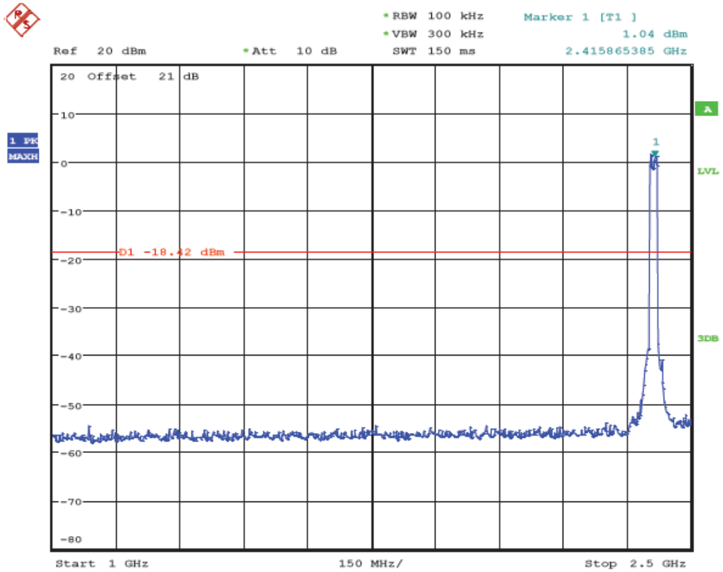
(Plot 4.6.3 A4: Channel 1: 2412MHz @ 802.11n HT20)
