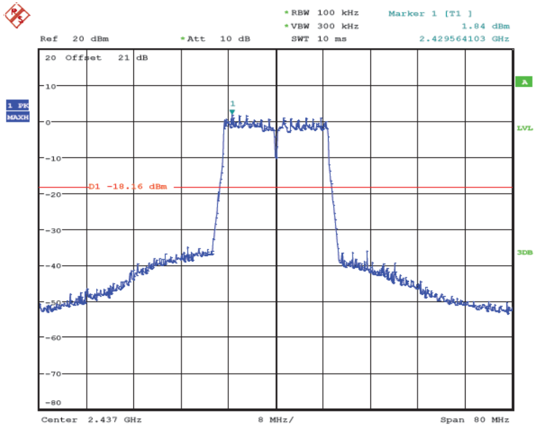
(Plot 4.6.3 B1: Channel 6: 2437MHz @ 802.11n HT20)
