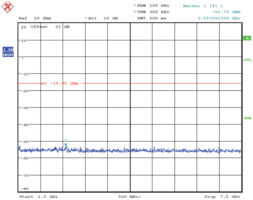
(Plot 4.6.1 B5: Channel 6: 2437MHz @ 802.11b)
