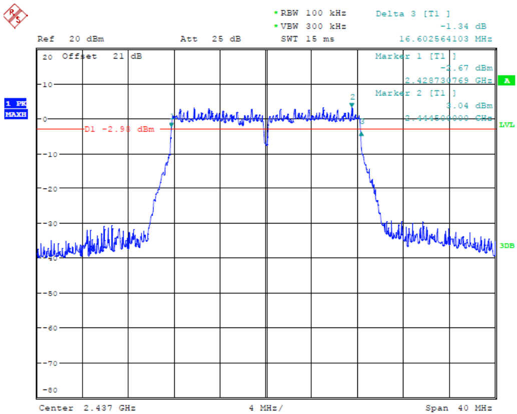
(Plot 4.7.2 B: Channel 6: 2437MHz @ 802.11g)
