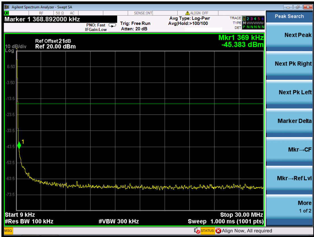
(Plot 4.6.1 A2: Channel 1: 2412MHz @ 802.11b)
