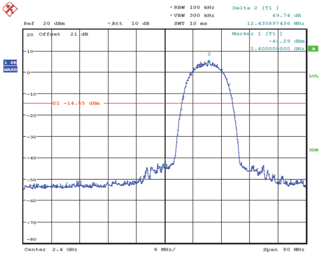
(Plot 6.6.1 D: Channel 1: 2412MHz @ 802.11b)
