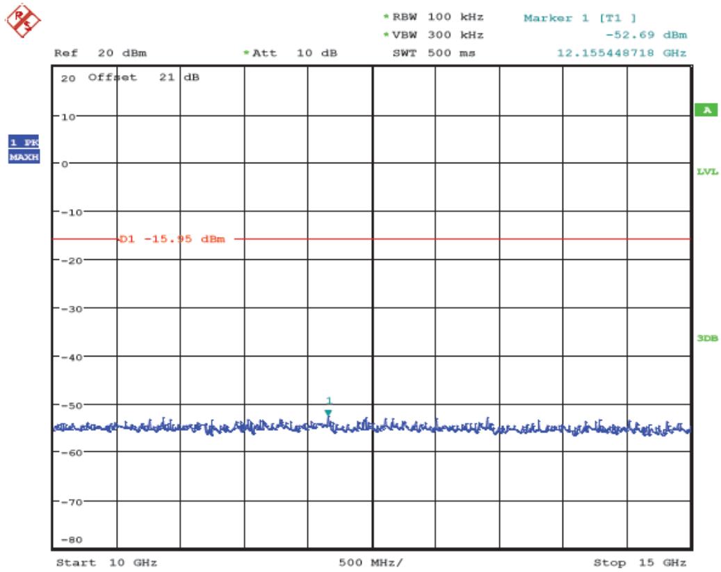
(Plot 4.6.1 B7: Channel 6: 2437MHz @ 802.11b)
