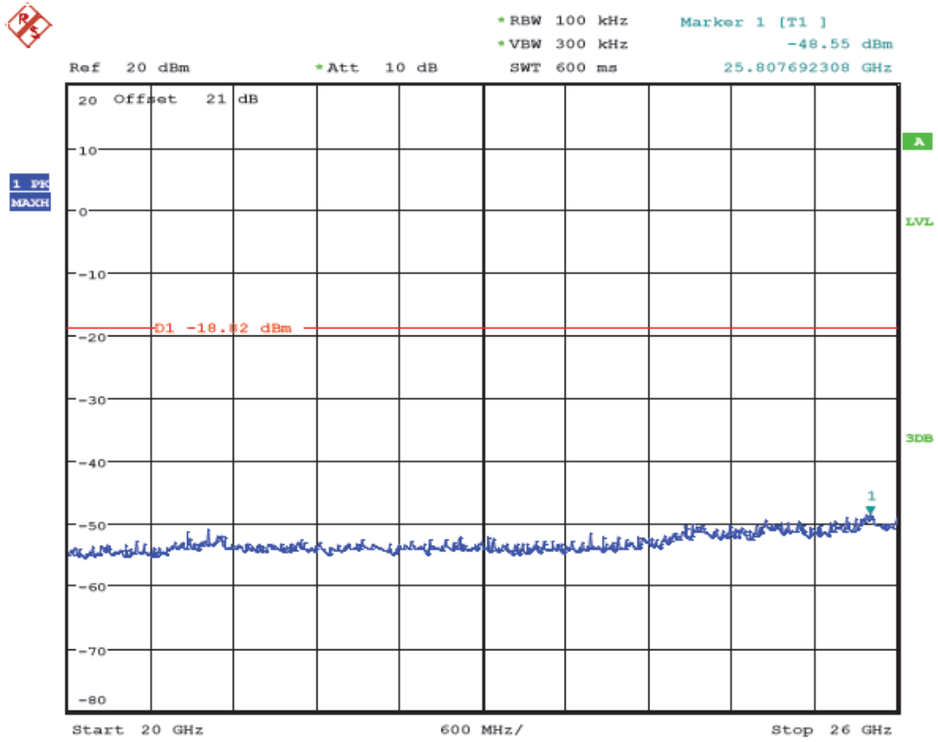
(Plot 4.6.2 A9: Channel 1: 2412MHz @ 802.11g)
