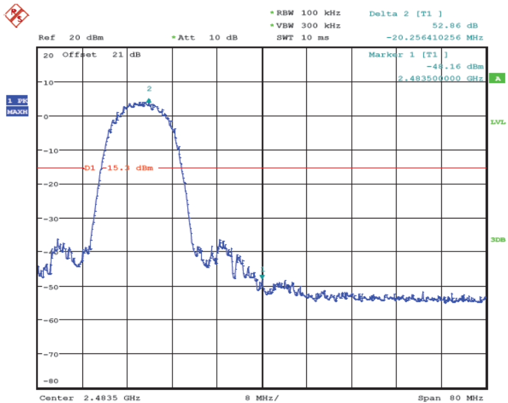
(Plot 6.6.1 E: Channel 11: 2462MHz @ 802.11b)
