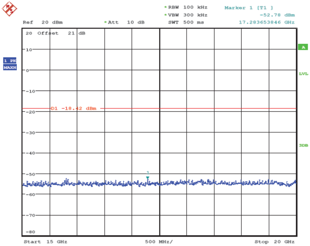
(Plot 4.6.3 A8: Channel 1: 2412MHz @ 802.11n HT20)
