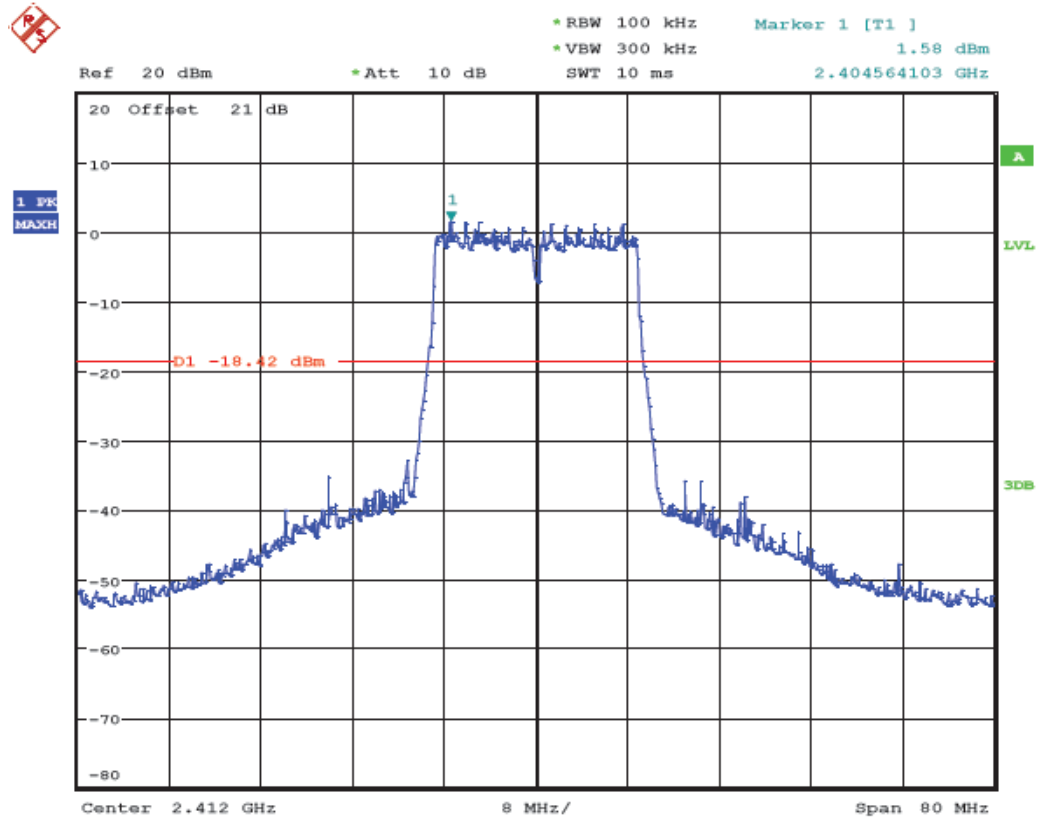
(Plot 4.6.3 A1: Channel 1: 2412MHz @ 802.11n HT20)
