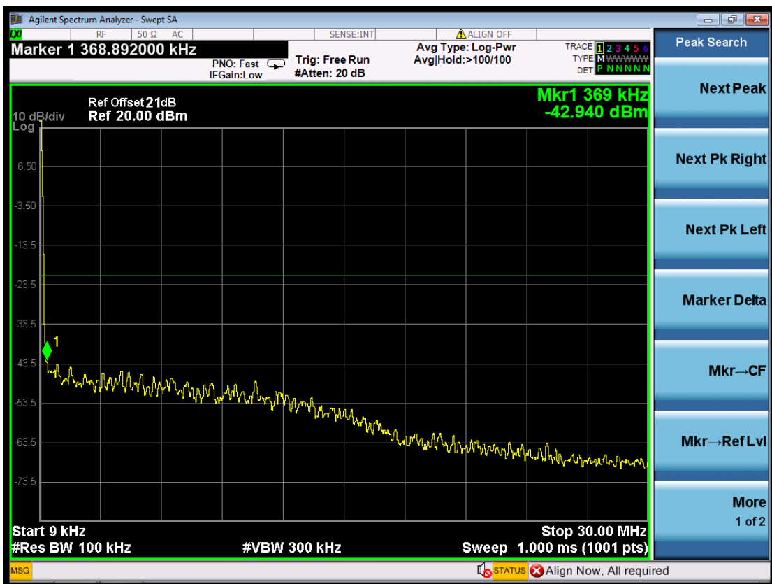
(Plot 4.6.3 B2: Channel 6: 2437MHz @ 802.11n HT20)
