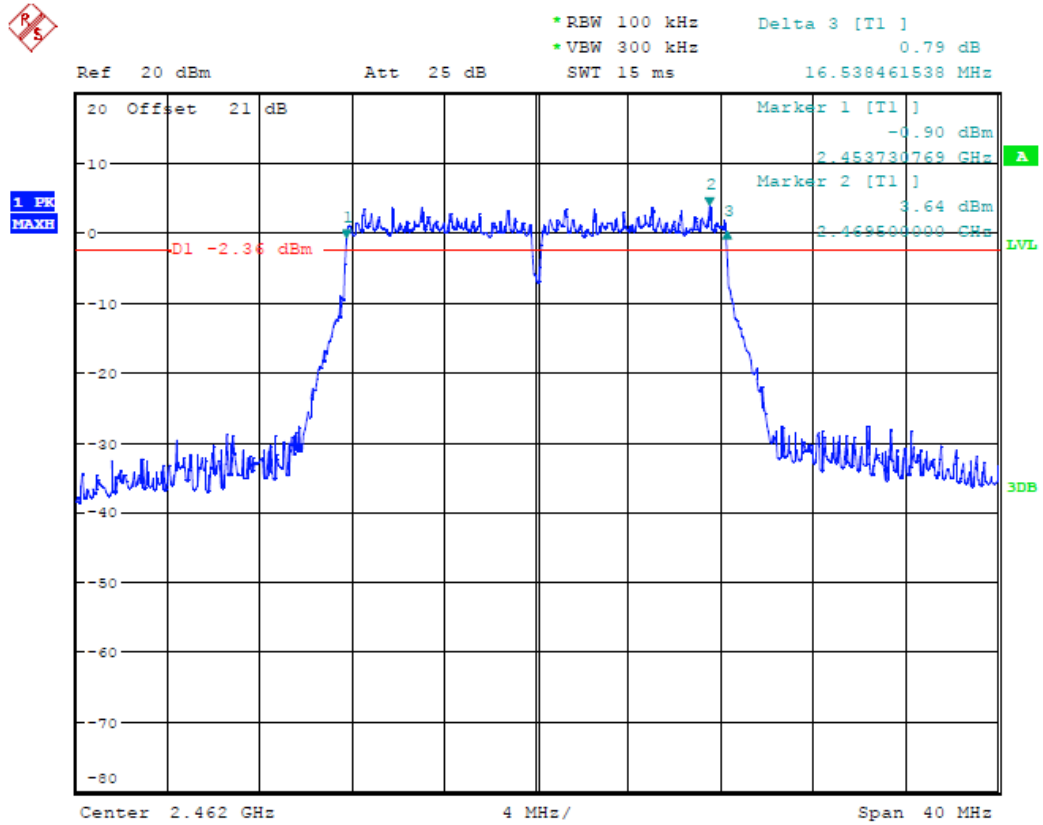
(Plot 4.7.2 C: Channel 11: 2462MHz @ 802.11g)
