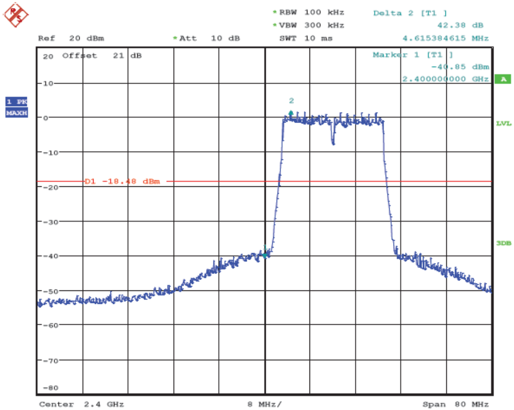
(Plot 4.6.3 D: Channel 1: 2412MHz @ 802.11n HT20)
