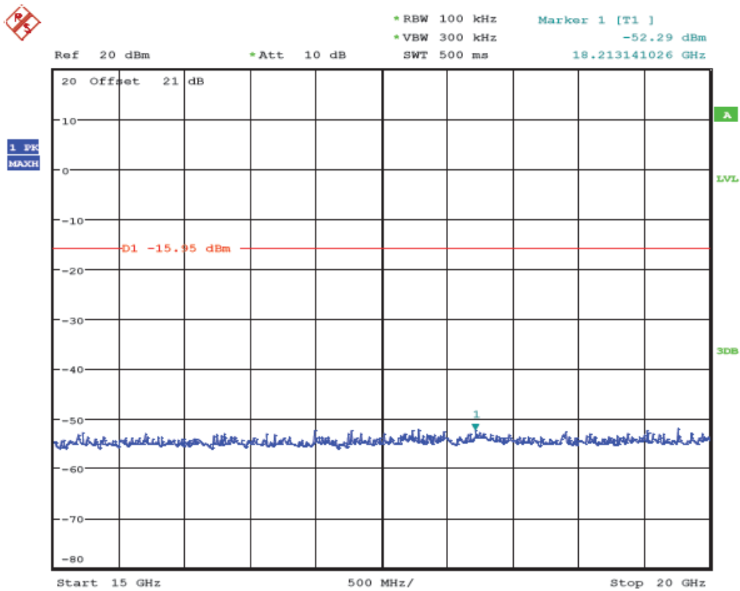
(Plot 4.6.1 B8: Channel 6: 2437MHz @ 802.11b)
