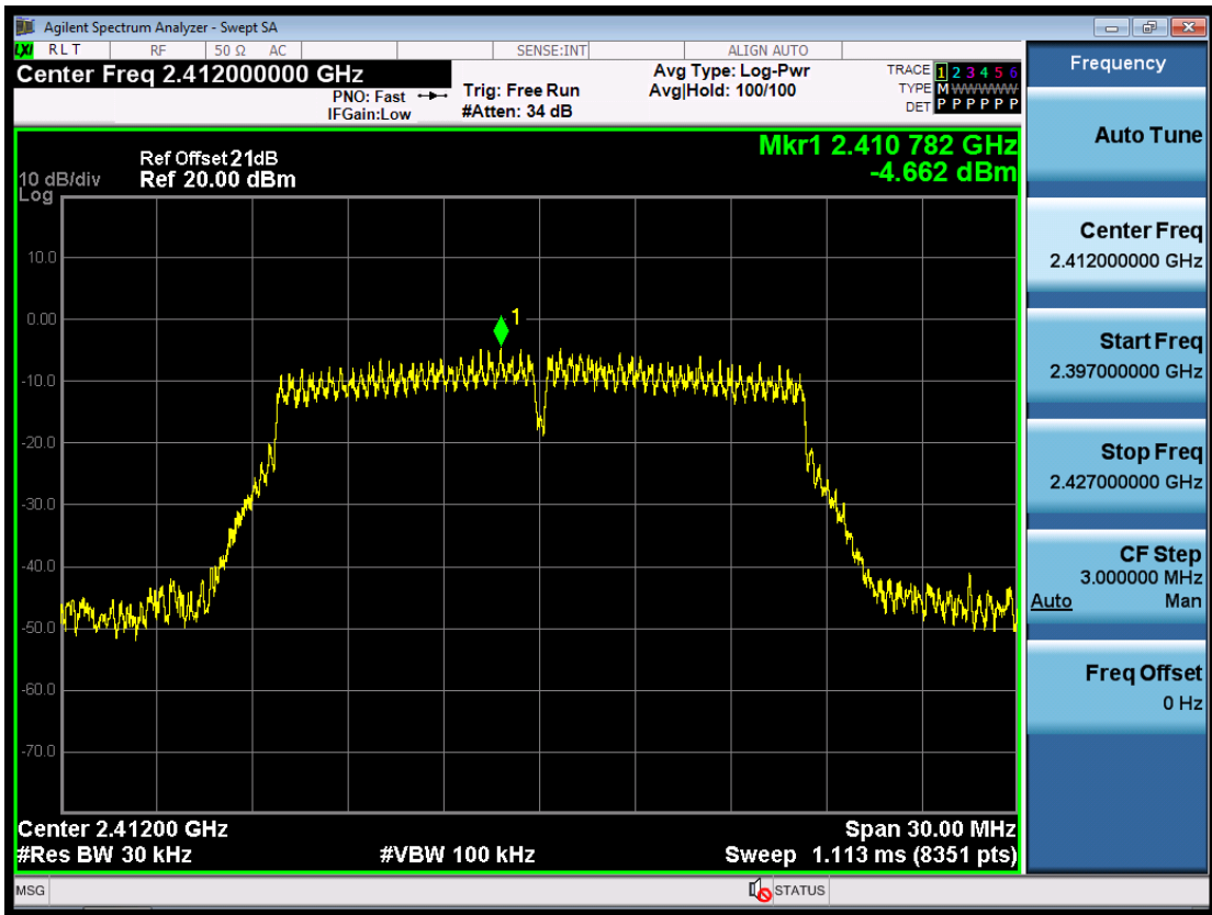
(Plot 4.4.2 A: Channel 1: 2412MHz @ 802.11g)
