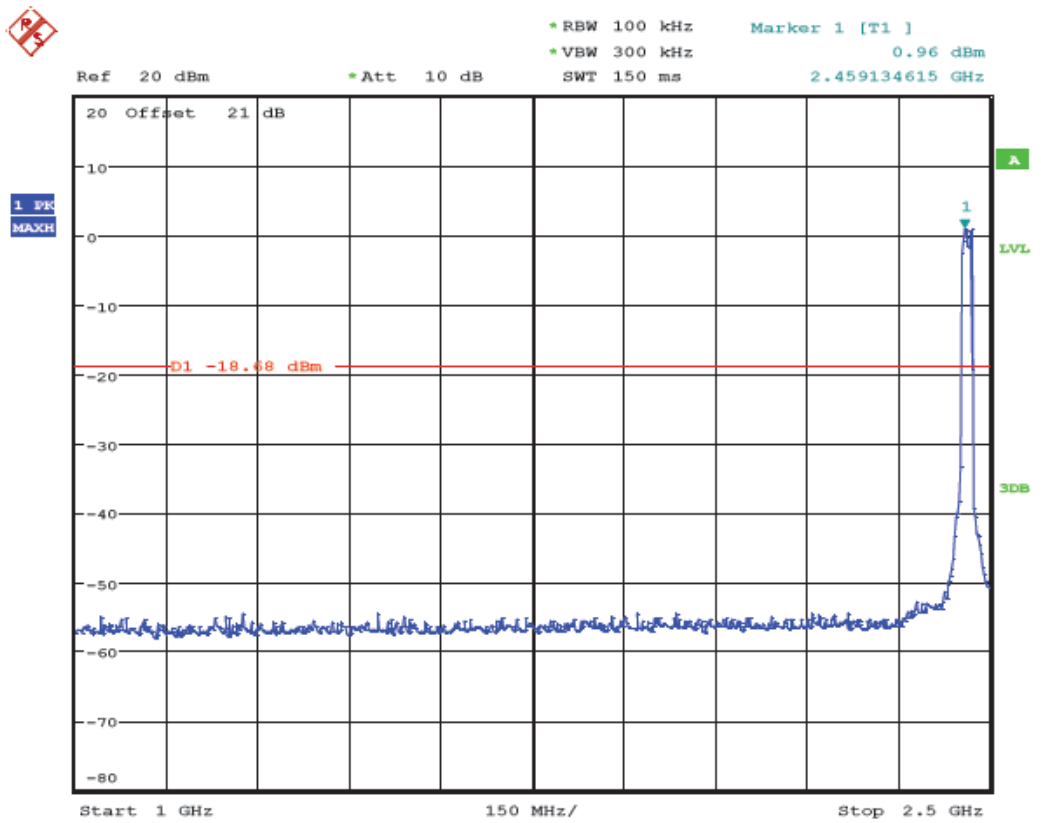
(Plot 4.6.2 C4: Channel 11: 2462MHz @ 802.11g)
