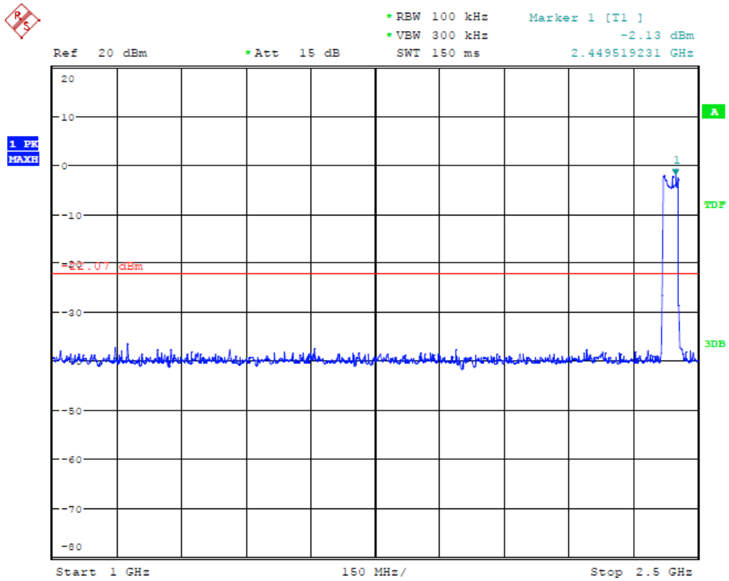
(Plot 4.6.4 B4: Channel 6: 2437MHz @ 802.11n HT40)
