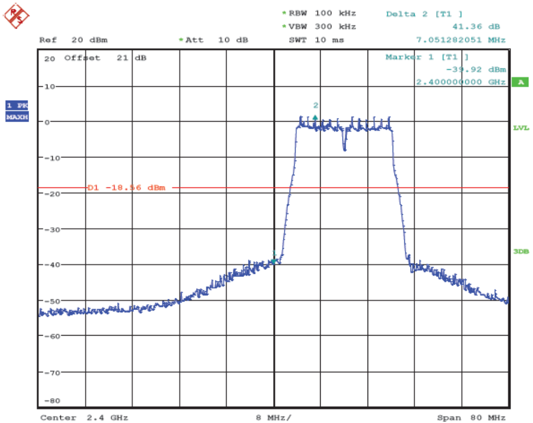
(Plot 4.6.2 D: Channel 1: 2412MHz @ 802.11g)
