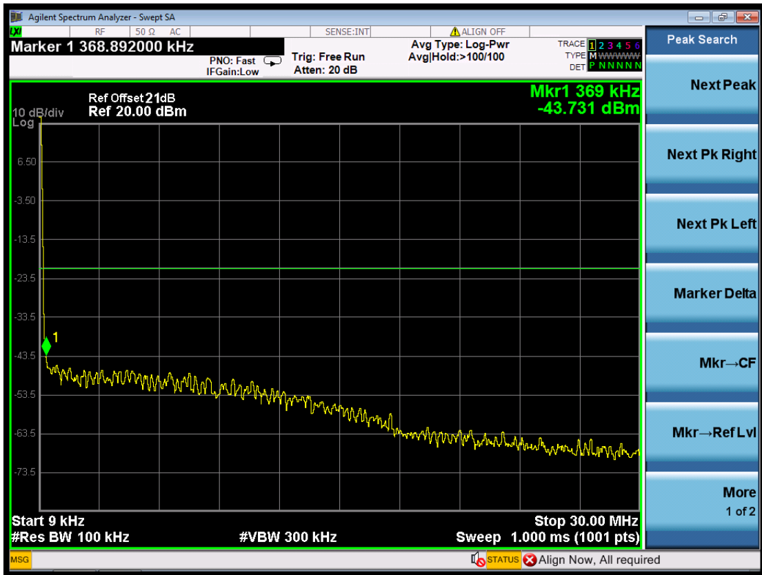
(Plot 4.6.3 A2: Channel 1: 2412MHz @ 802.11n HT20)
