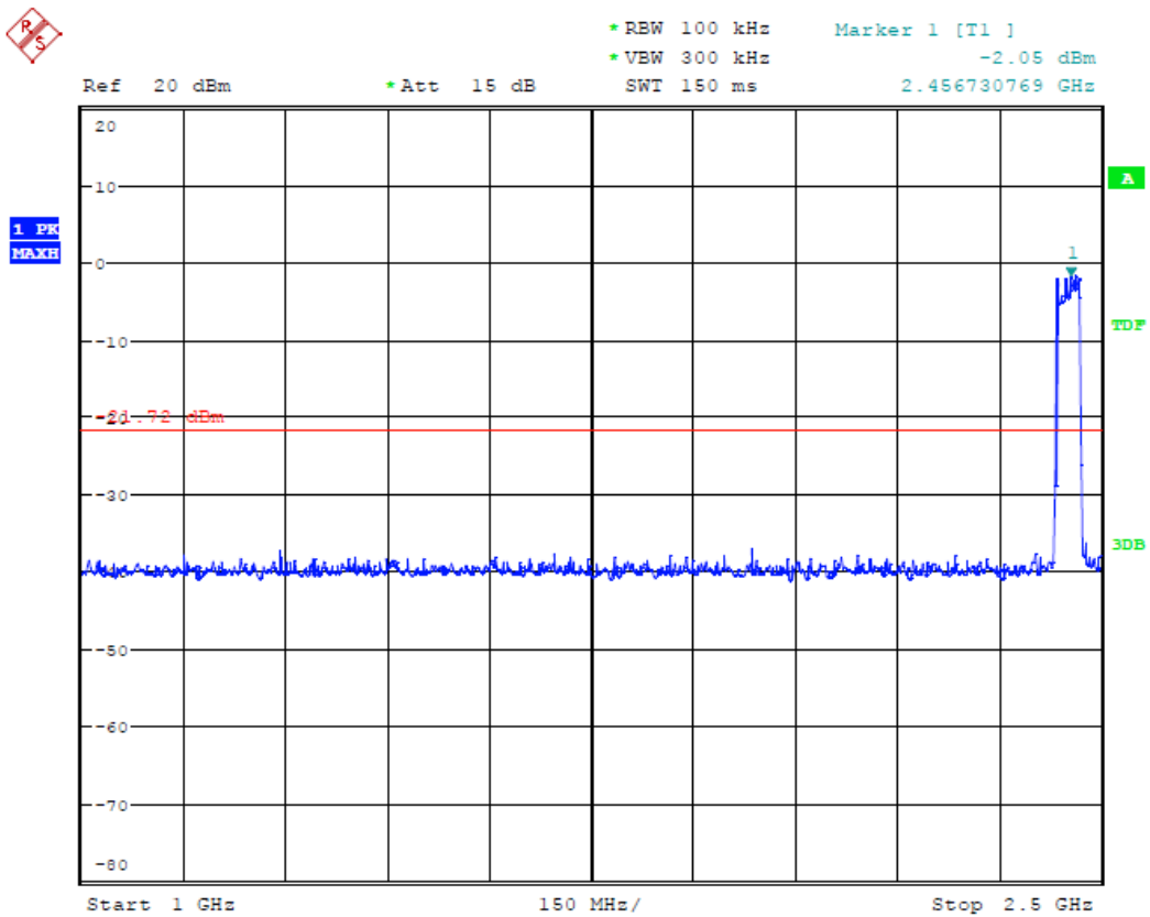
(Plot 4.6.4 C4: Channel 11: 2462MHz @ 802.11n HT40)
