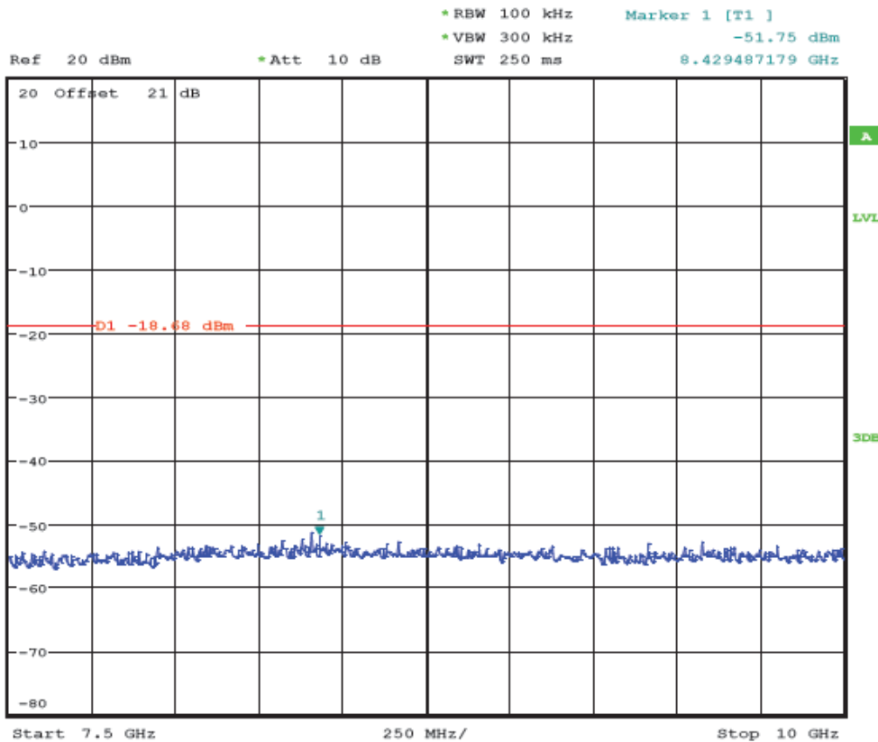
(Plot 4.6.2 C6: Channel 11: 2462MHz @ 802.11g)
