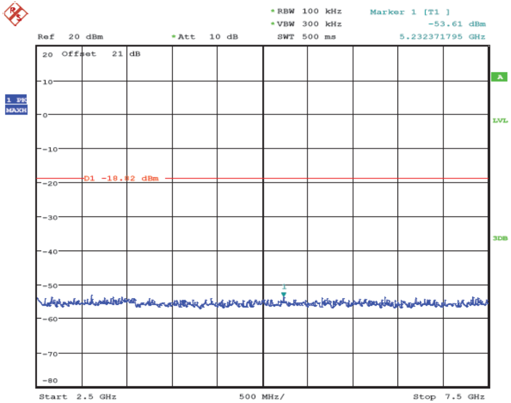
(Plot 4.6.2 A5: Channel 1: 2412MHz @ 802.11g)
