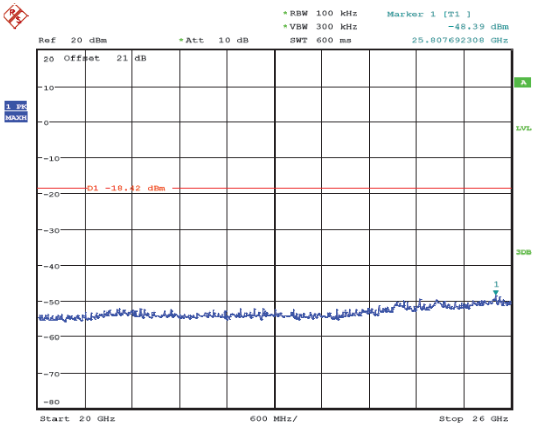
(Plot 4.6.3 A9: Channel 1: 2412MHz @ 802.11n HT20)
