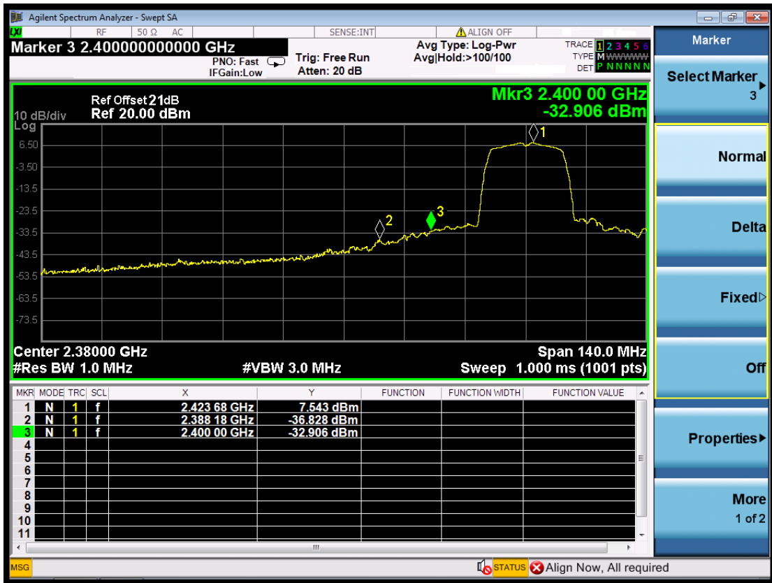
(Plot 4.5.4 A1: Channel 3: 2422MHz @ 802.11n HT40MHz)
