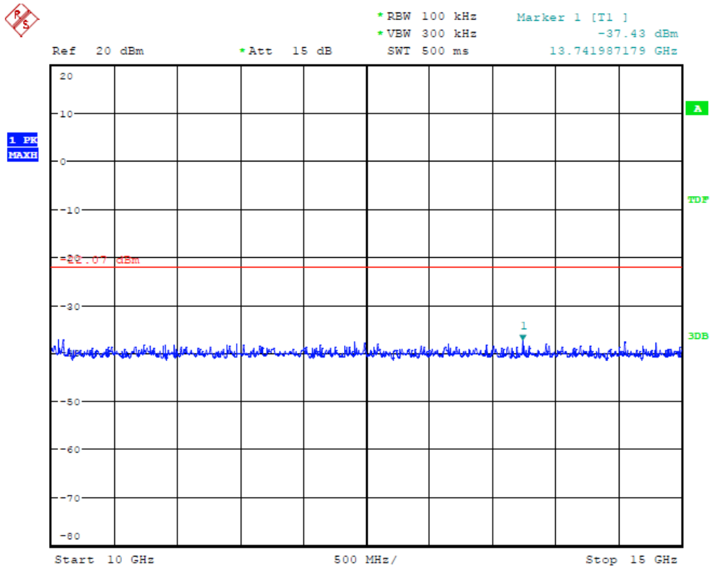
(Plot 4.6.4 A7: Channel 3: 2422MHz @ 802.11n HT40)
