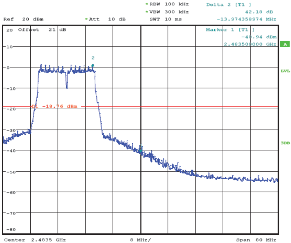
(Plot 4.6.2 E: Channel 11: 2462MHz @ 802.11g)
