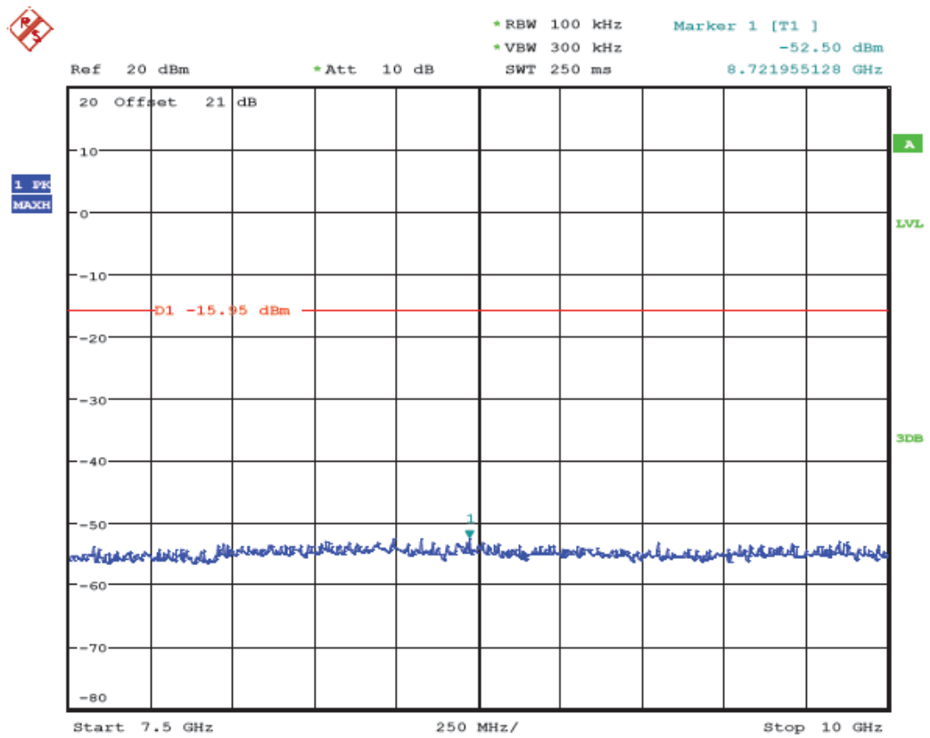
(Plot 4.6.1 B6: Channel 6: 2437MHz @ 802.11b)
