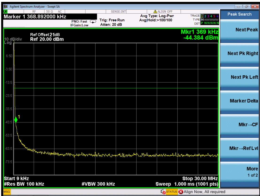
(Plot 4.6.1 B2: Channel 6: 2437MHz @ 802.11b)
