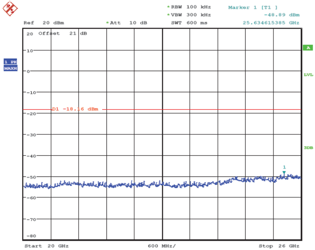
(Plot 4.6.3 B9: Channel 6: 2437MHz @ 802.11n HT20)
