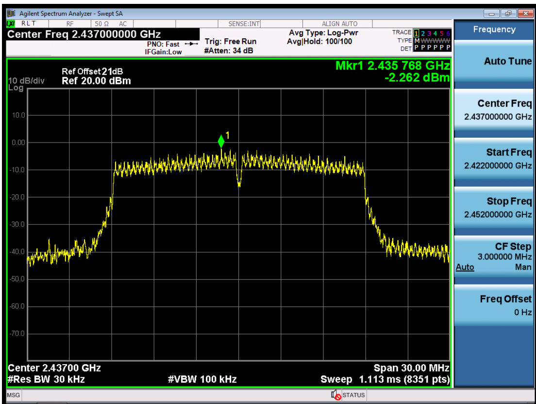
(Plot 4.4.3 B: Channel 6: 2437MHz @ 802.11n HT20)
