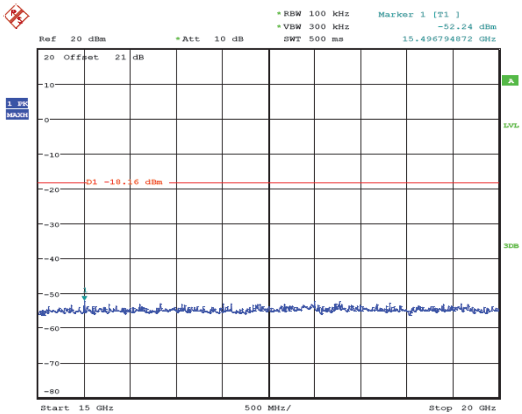
(Plot 4.6.3 B8: Channel 6: 2437MHz @ 802.11n HT20)
