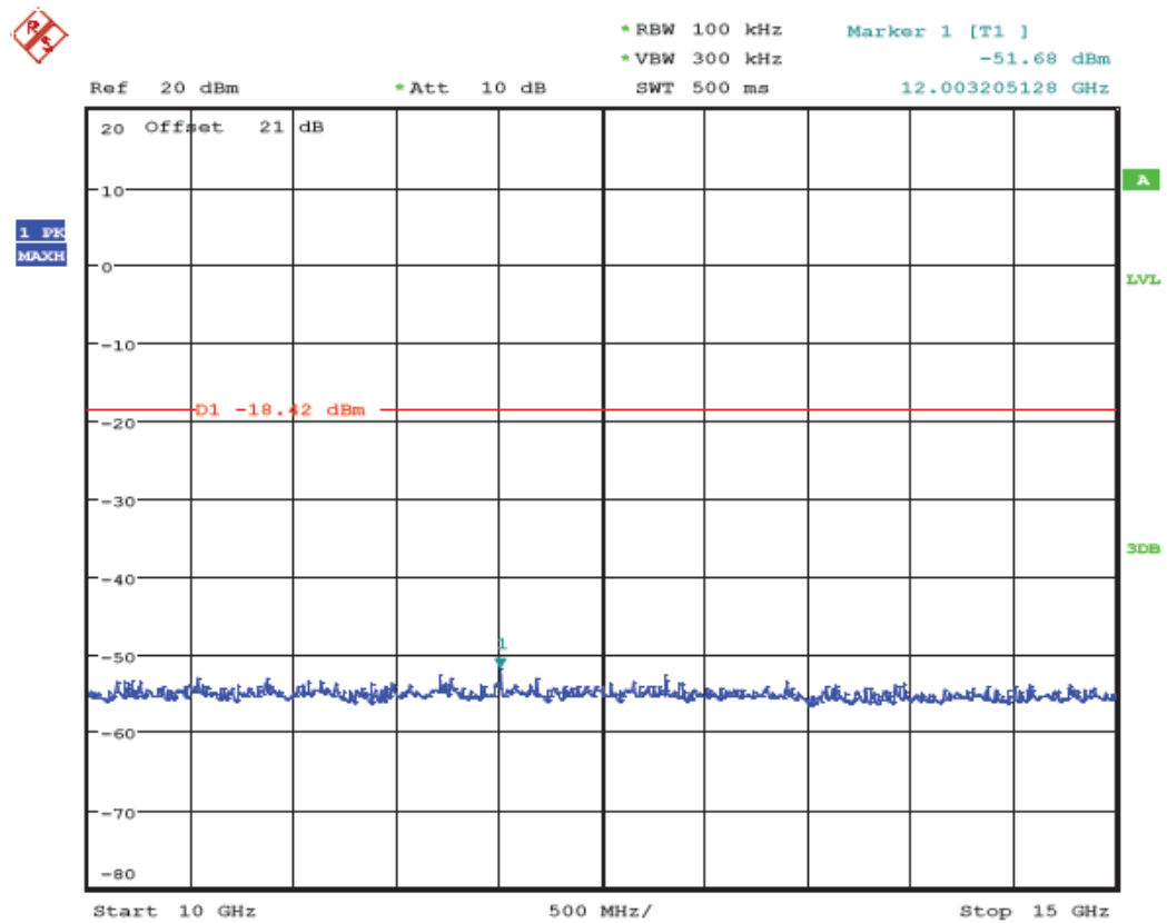
(Plot 4.6.3 A7: Channel 1: 2412MHz @ 802.11n HT20)
