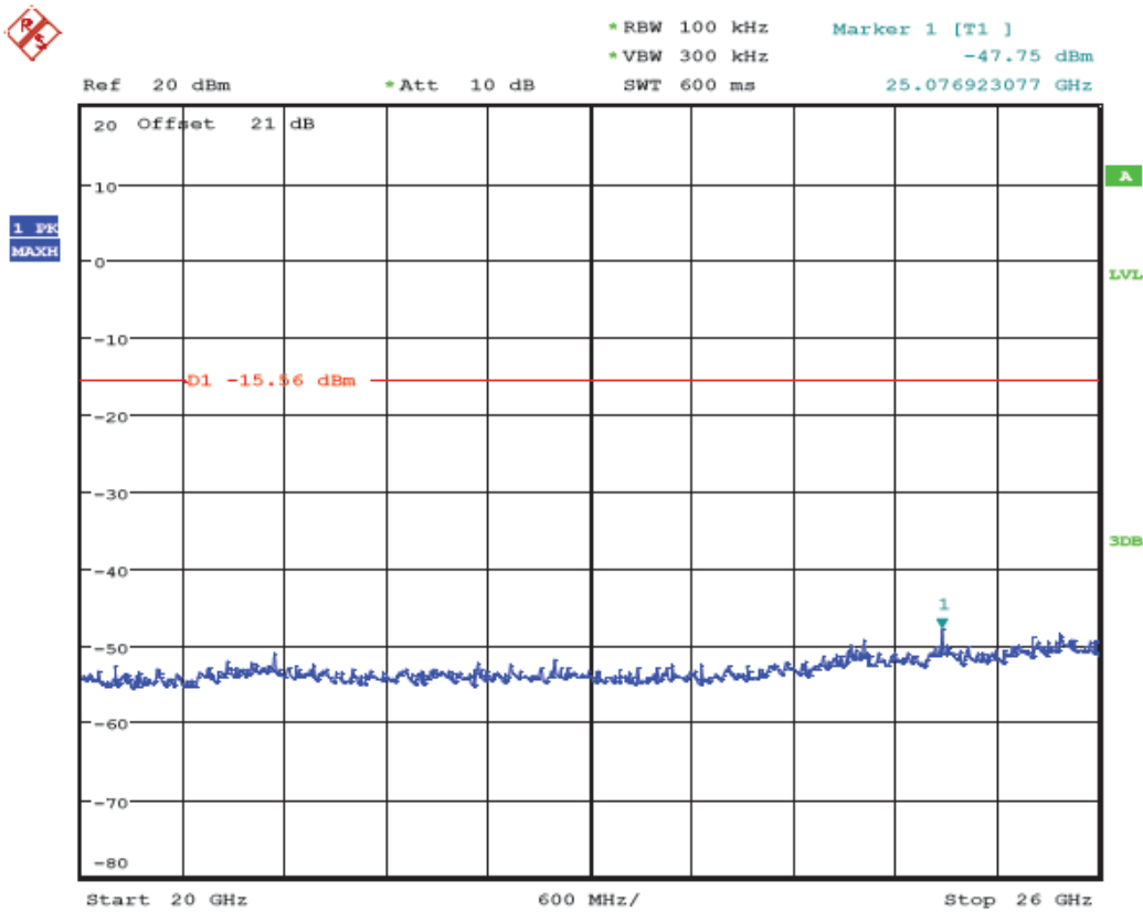
(Plot 4.6.1 C9: Channel 11: 2462MHz @ 802.11b)
