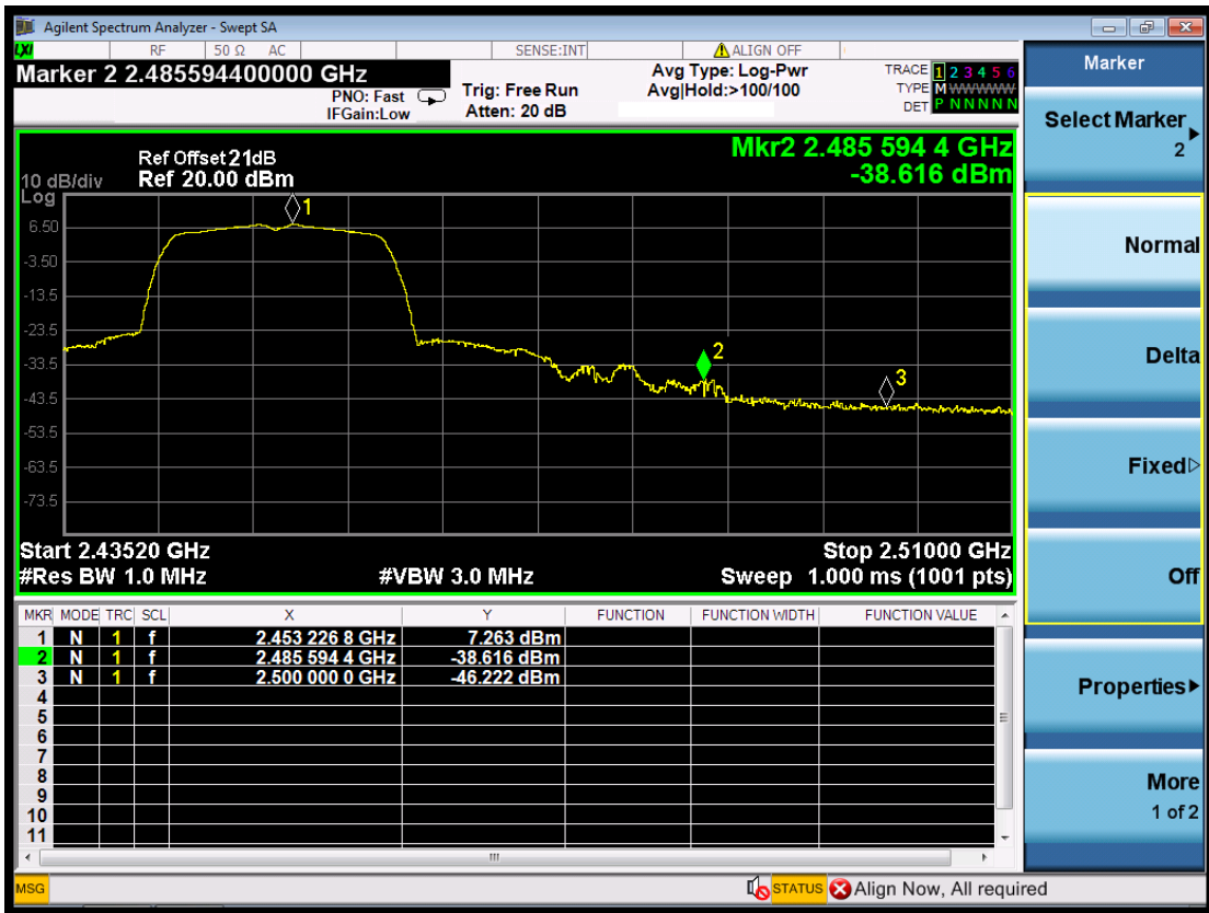
(Plot 6.5.4 A3: Channel 9: 2452MHz @ 802.11n HT40MHz)
