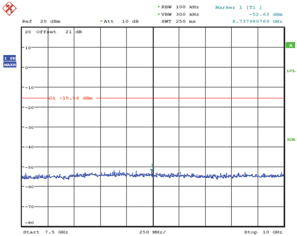
(Plot 4.6.1 C6: Channel 11: 2462MHz @ 802.11b)
