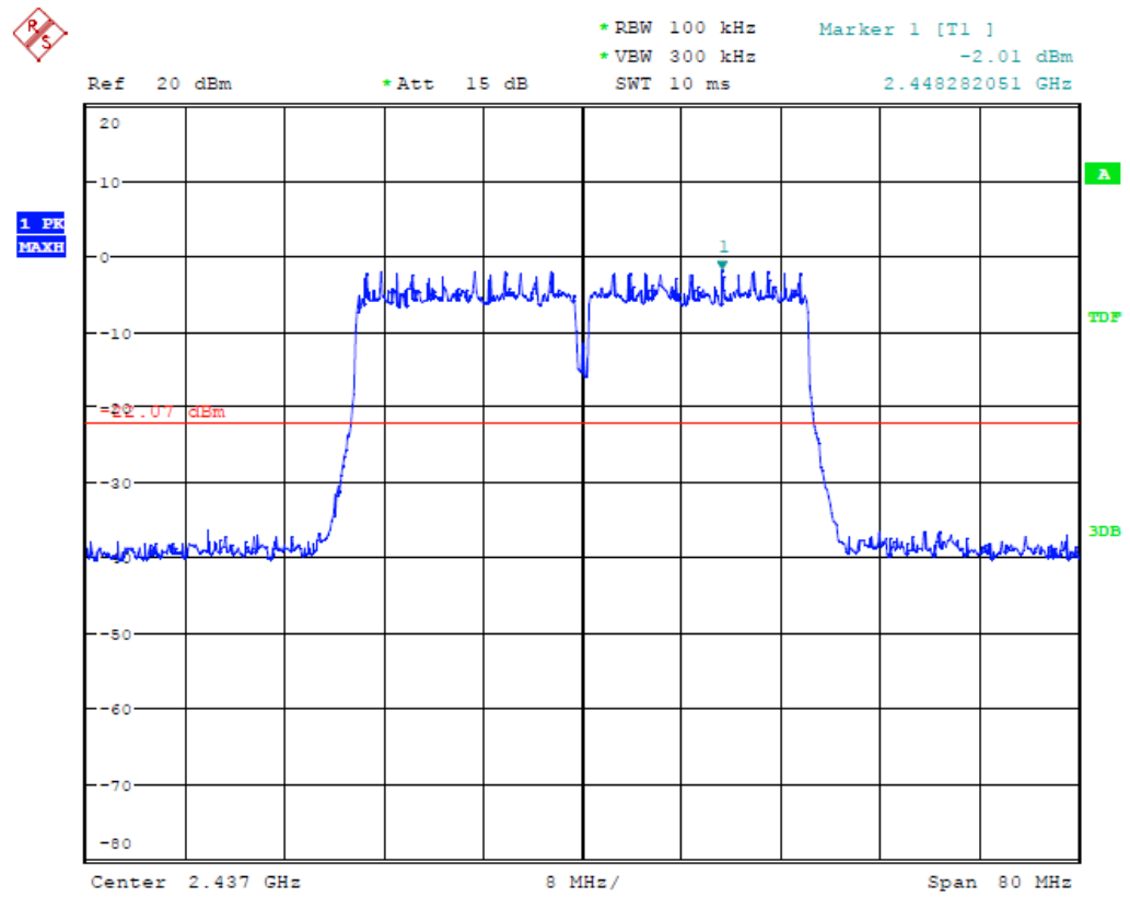
(Plot 4.6.4 B1: Channel 6: 2437MHz @ 802.11n HT40)
