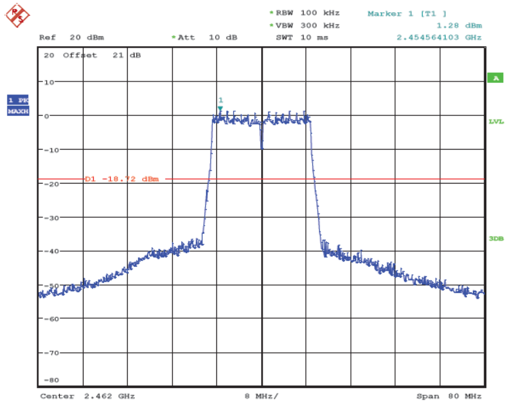
(Plot 4.6.3 C1: Channel 11: 2462MHz @ 802.11n HT20)
