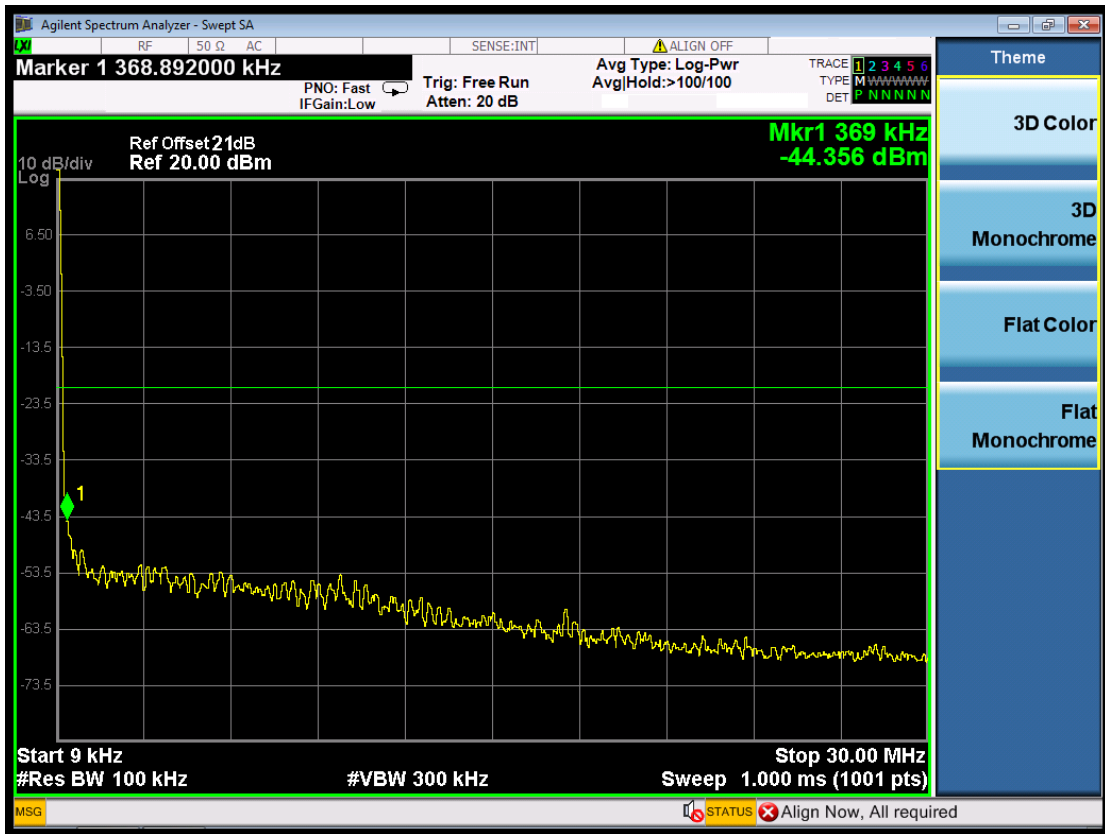
(Plot 4.6.2 B2: Channel 6: 2437MHz @ 802.11g)
