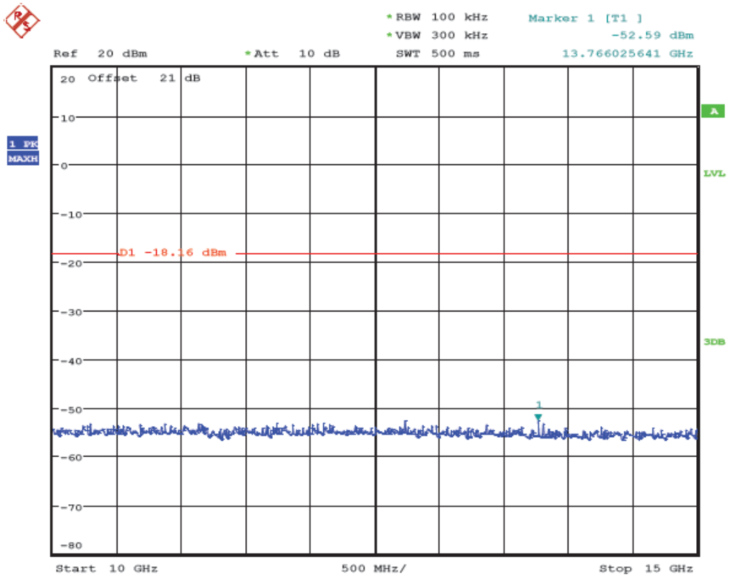
(Plot 4.6.3 B7: Channel 6: 2437MHz @ 802.11n HT20)
