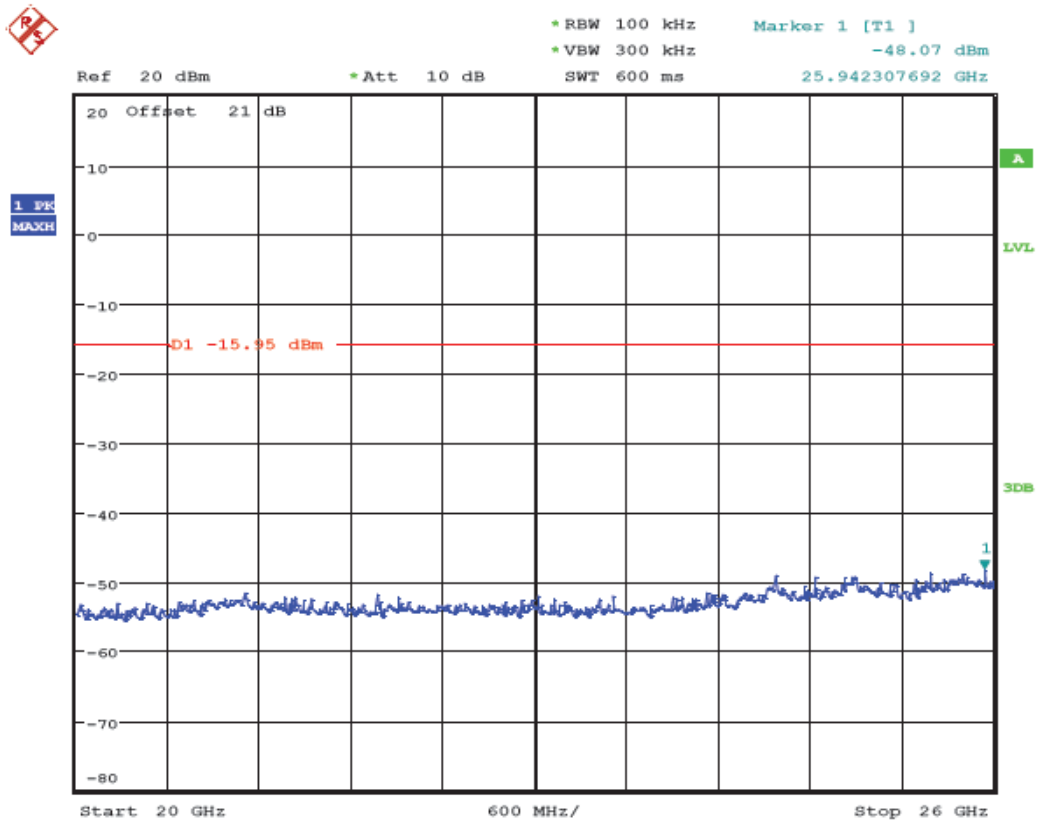
(Plot 4.6.1 B9: Channel 6: 2437MHz @ 802.11b)
