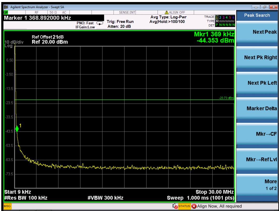
(Plot 4.6.2 A2: Channel 1: 2412MHz @ 802.11g)
