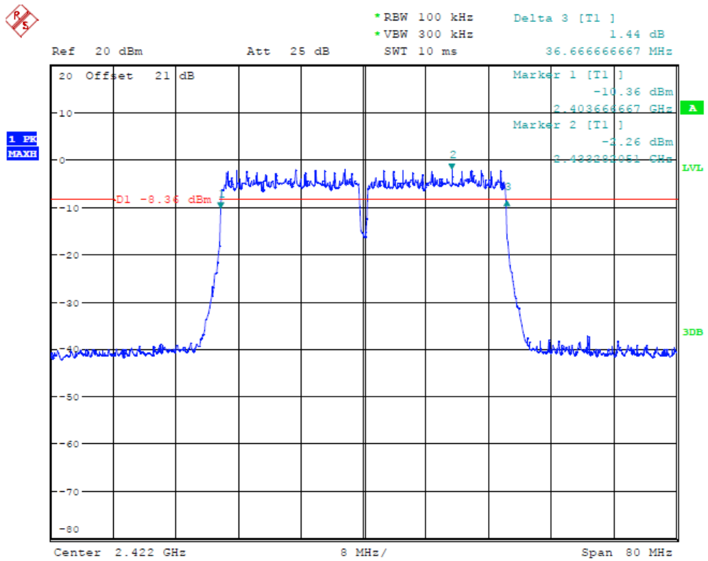
(Plot 4.7.4 A: Channel 3: 2422MHz @ 802.11n HT40MHz)
