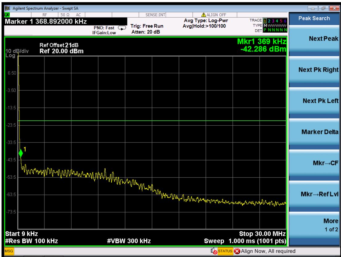
(Plot 4.6.2 C2: Channel 11: 2462MHz @ 802.11g)
