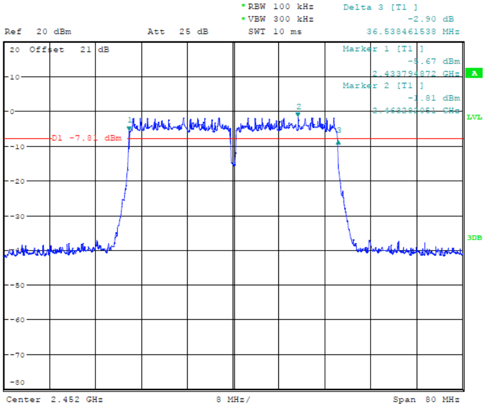
(Plot 4.7.4 C: Channel 9: 2452MHz @ 802.11n HT40MHz)
