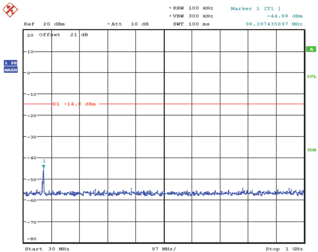
(Plot 6.6.1 A3: Channel 1: 2412MHz @ 802.11b)
