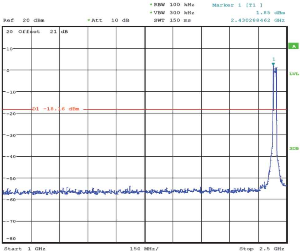
(Plot 4.6.3 B4: Channel 6: 2437MHz @ 802.11n HT20)
