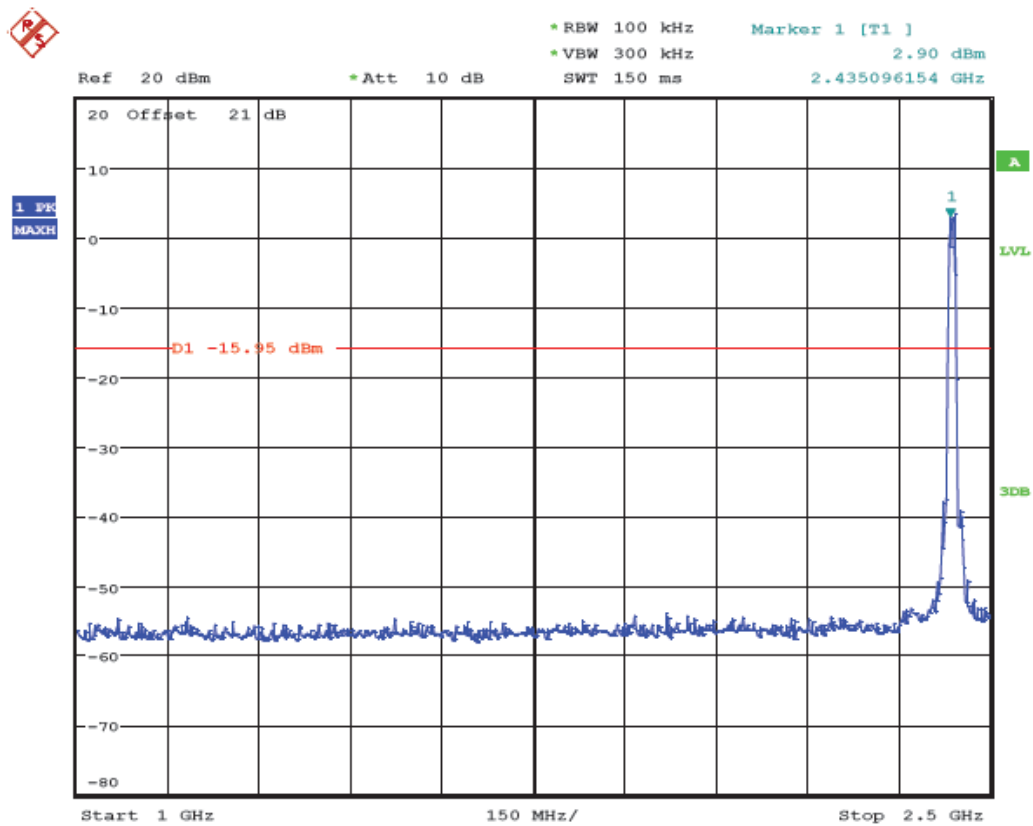
(Plot 4.6.1 B4: Channel 6: 2437MHz @ 802.11b)
