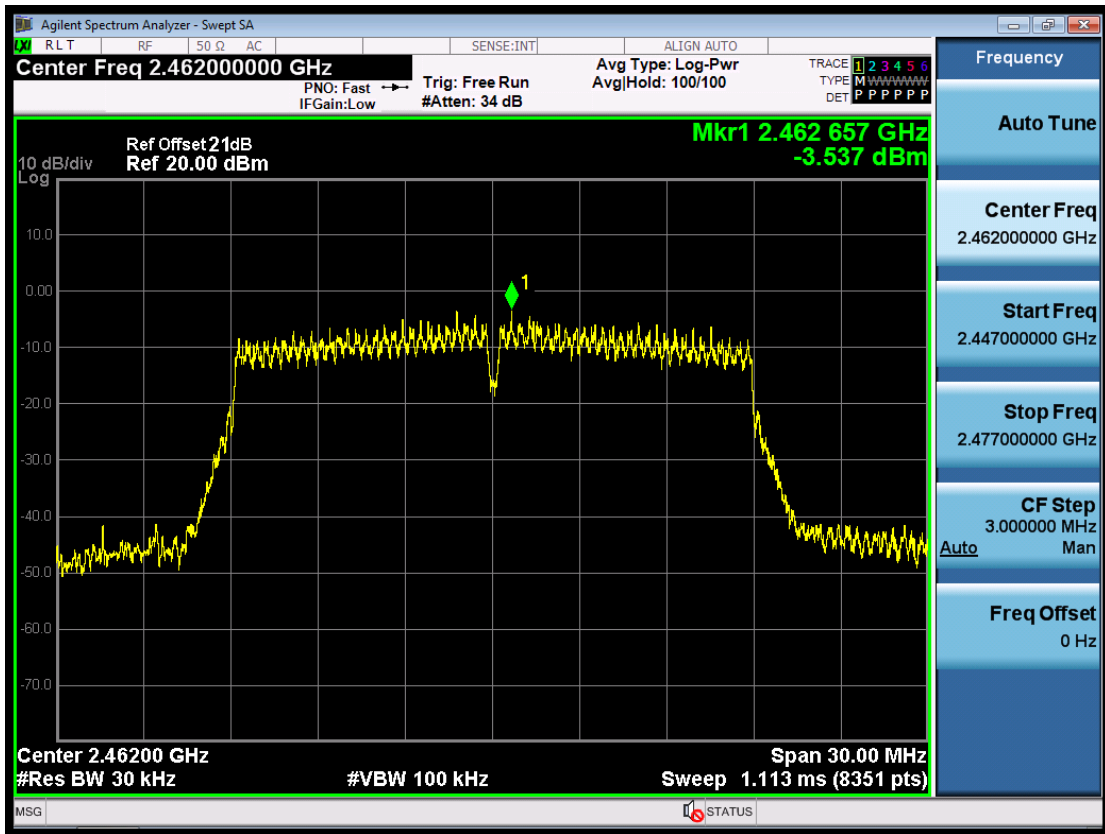
(Plot 4.4.3 C: Channel 11: 2462MHz @ 802.11n HT20)
