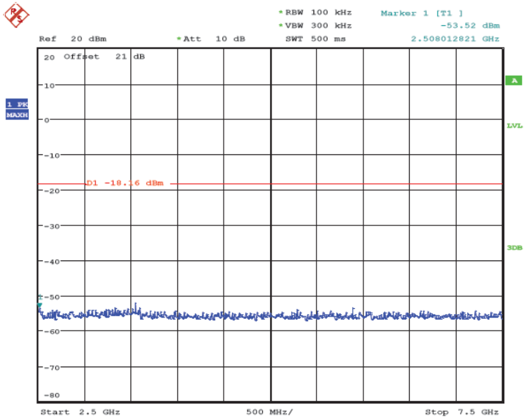
(Plot 4.6.3 B5: Channel 6: 2437MHz @ 802.11n HT20)
