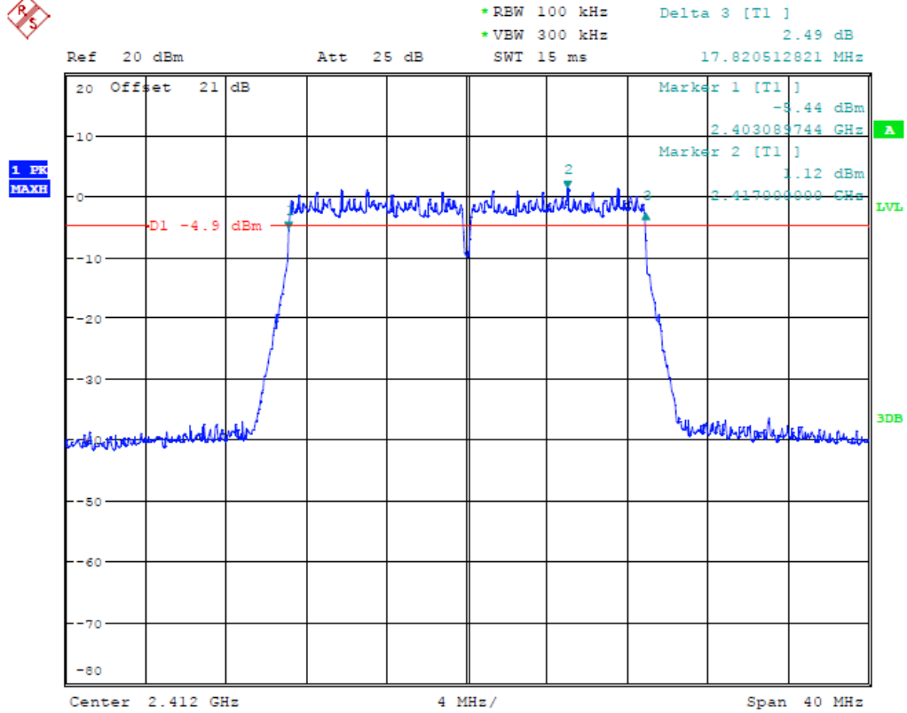
(Plot 4.7.3 A: Channel 1: 2412MHz @ 802.11n HT20)
