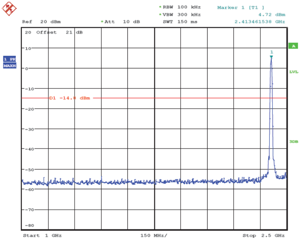
(Plot 4.6.1 A4: Channel 1: 2412MHz @ 802.11b)
