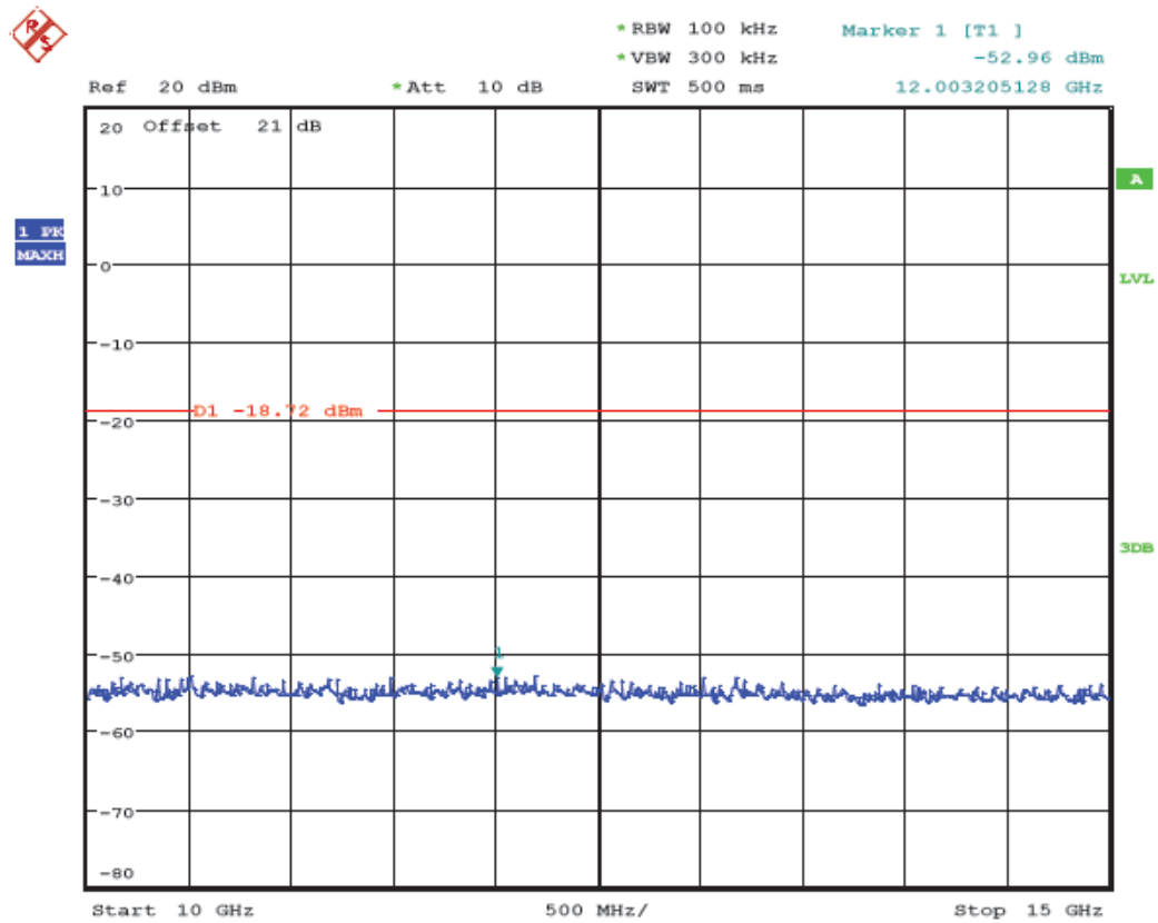
(Plot 4.6.3 C7: Channel 11: 2462MHz @ 802.11n HT20)
