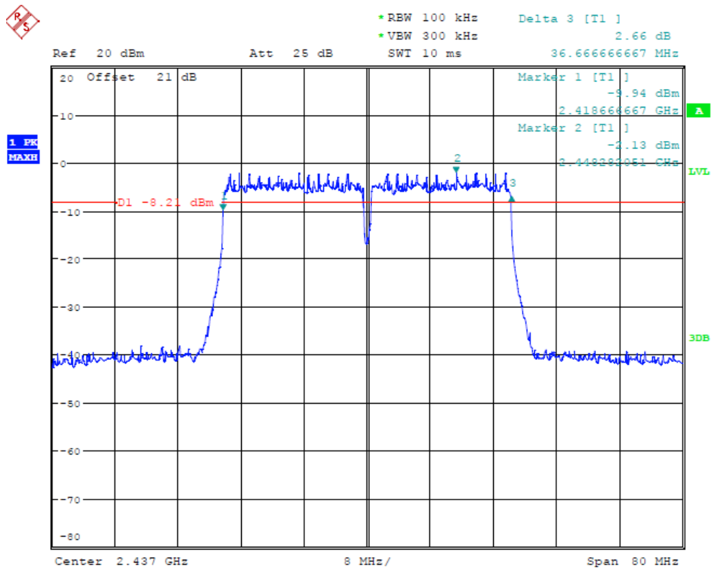
(Plot 4.7.3 B: Channel 6: 2437MHz @ 802.11n HT40MHz)
