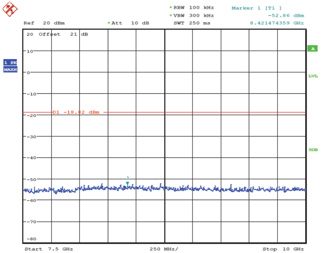
(Plot 4.6.2 A6: Channel 1: 2412MHz @ 802.11g)
