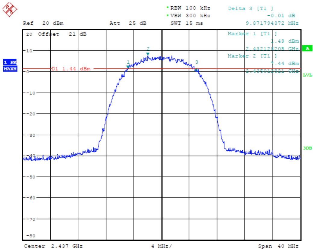
(Plot 4.7.1 B: Channel 6: 2437MHz @ 802.11b)
