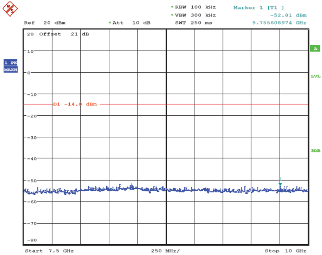
(Plot 4.6.1 A6: Channel 1: 2412MHz @ 802.11b)
