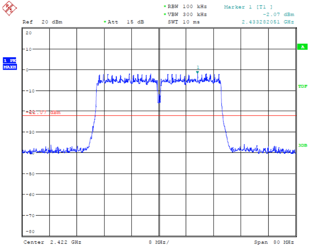
(Plot 4.6.4 A1: Channel 3: 2422MHz @ 802.11n HT40)
