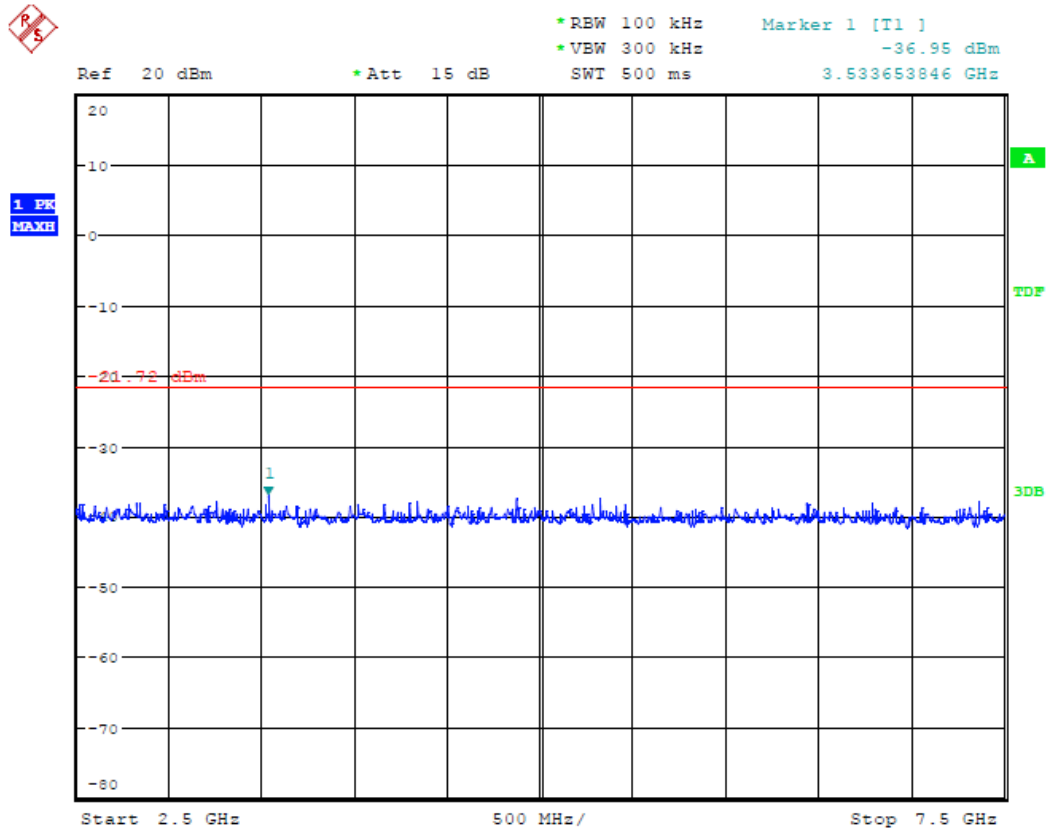
(Plot 4.6.4 C5: Channel 11: 2462MHz @ 802.11n HT40)
