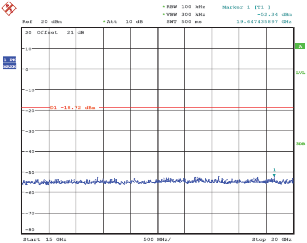
(Plot 4.6.3 C8: Channel 11: 2462MHz @ 802.11n HT20)
