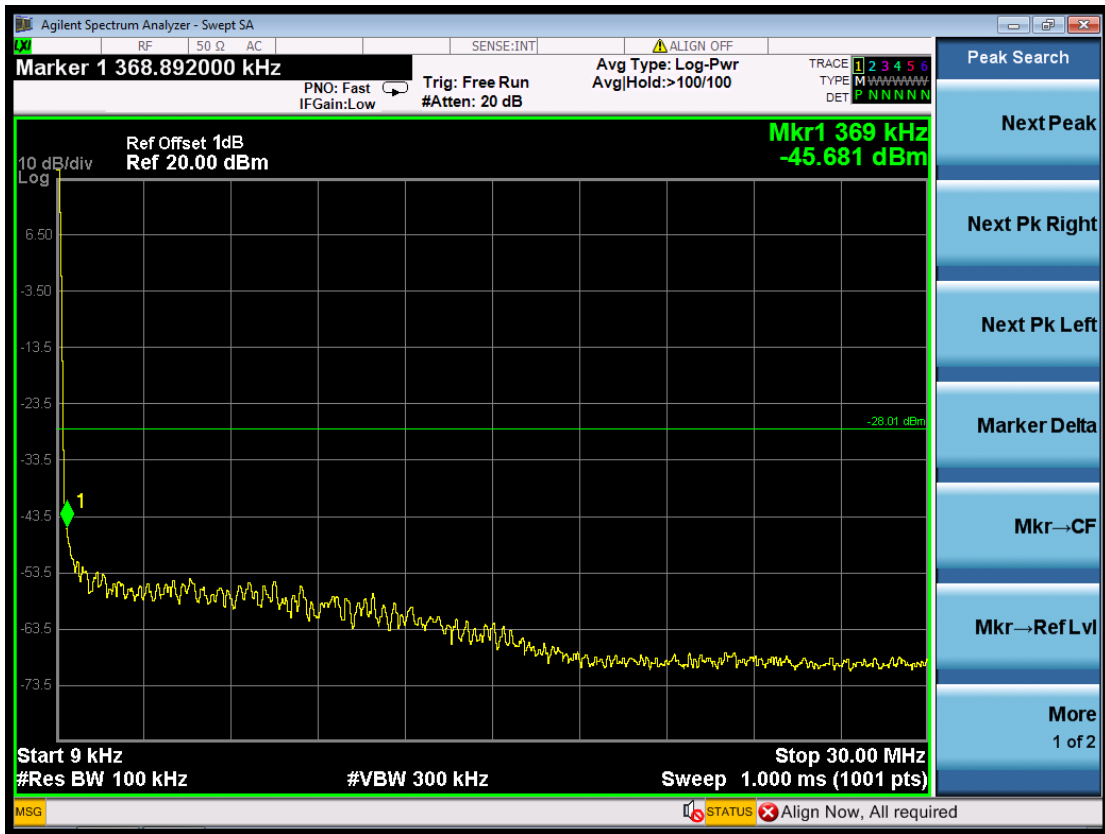
(Plot 4.6.4 B2: Channel 6: 2437MHz @ 802.11n HT40)
