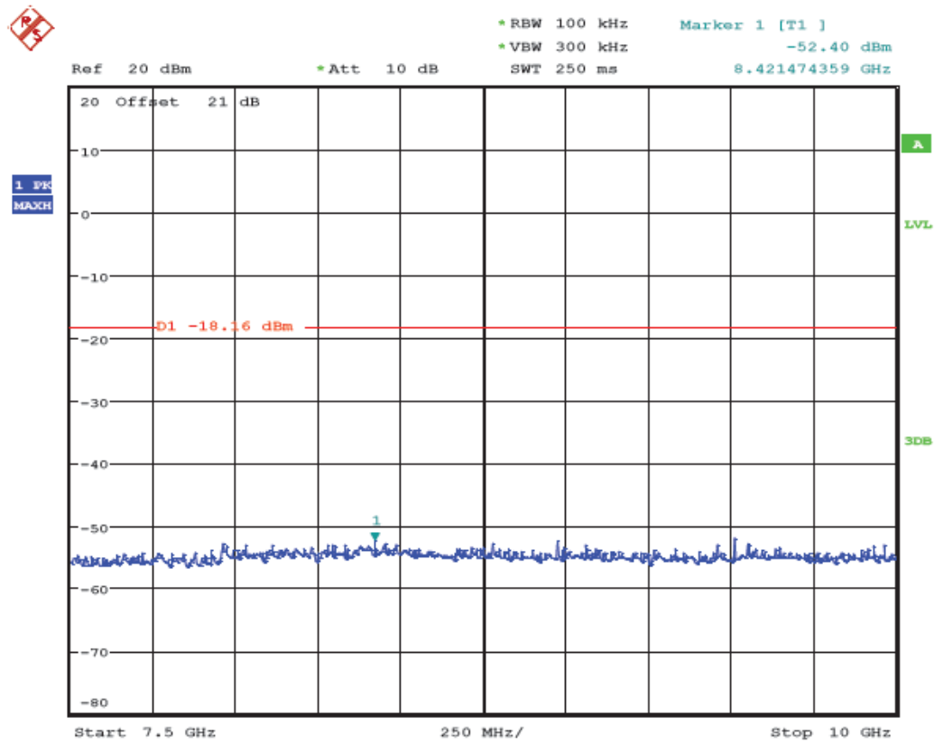
(Plot 4.6.3 B6: Channel 6: 2437MHz @ 802.11n HT20)
