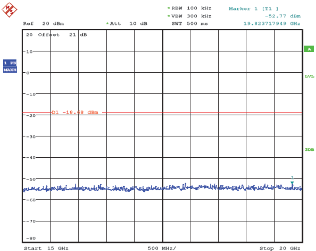
(Plot 4.6.2 C8: Channel 11: 2462MHz @ 802.11g)
