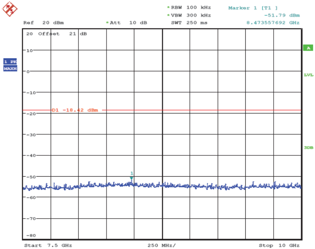
(Plot 4.6.3 A6: Channel 1: 2412MHz @ 802.11n HT20)
