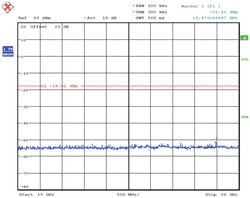
(Plot 4.6.2 B8: Channel 6: 2437MHz @ 802.11g)
