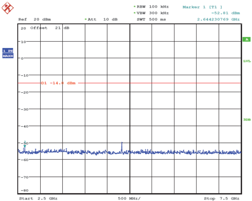
(Plot 4.6.1 A5: Channel 1: 2412MHz @ 802.11b)
