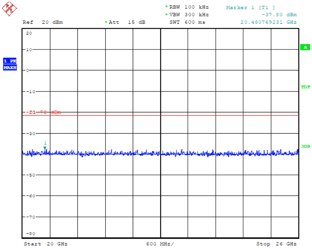
(Plot 4.6.4 C9: Channel 11: 2462MHz @ 802.11n HT40)
