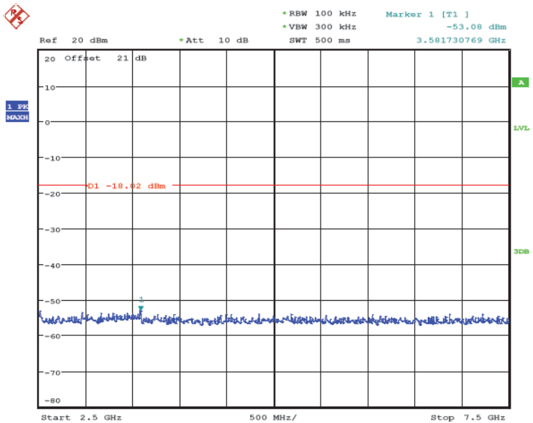
(Plot 4.6.2 B5: Channel 6: 2437MHz @ 802.11g)
