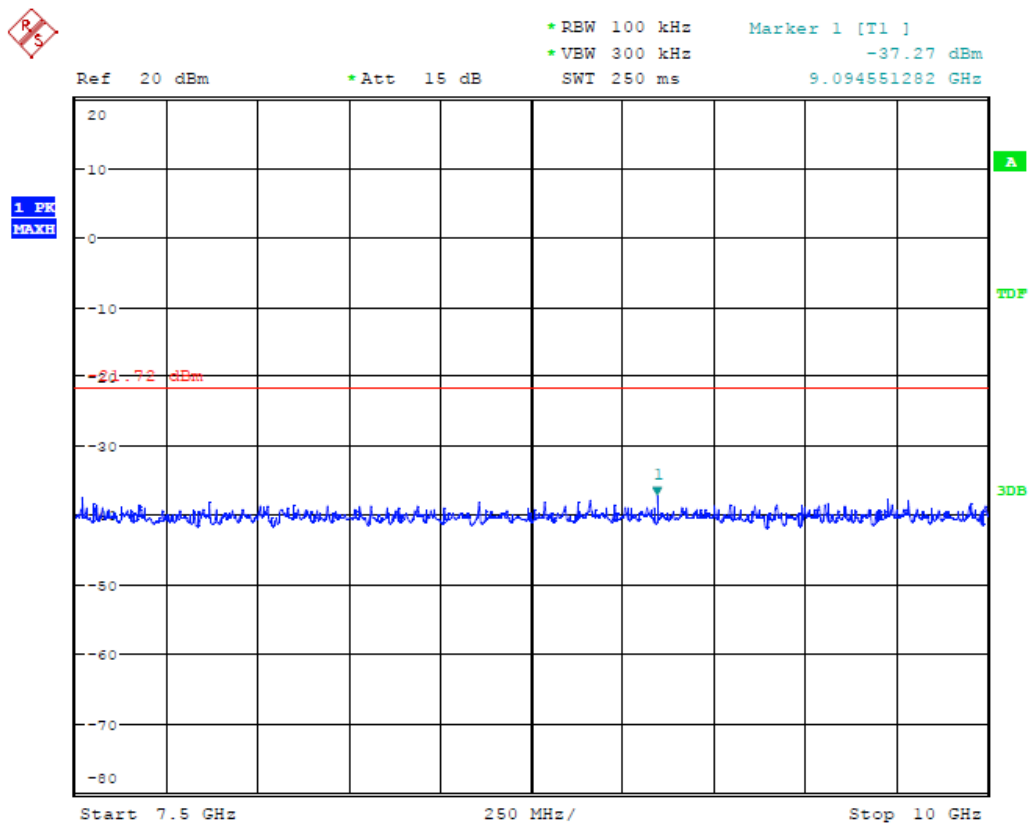
(Plot 4.6.4 C6: Channel 11: 2462MHz @ 802.11n HT40)
