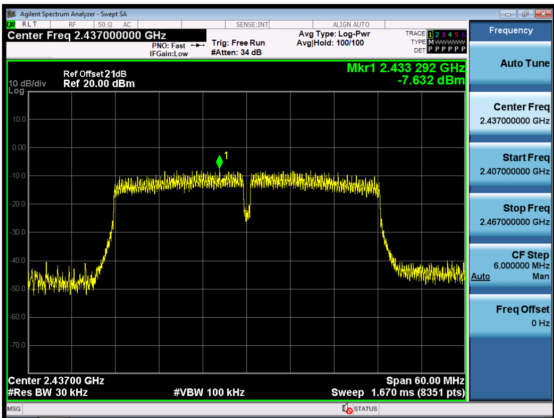
(Plot 4.4.4 B: Channel 6: 2437MHz @ 802.11n HT40)
