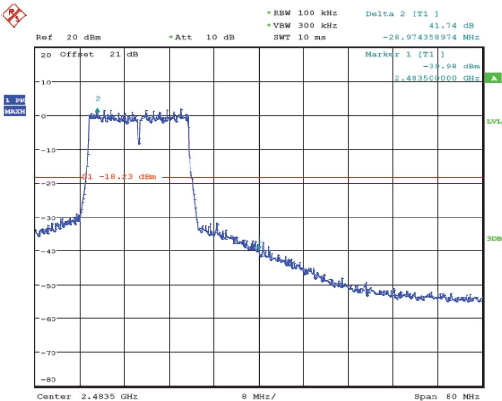
(Plot 4.6.3 E: Channel 11: 2462MHz @ 802.11n HT20)
