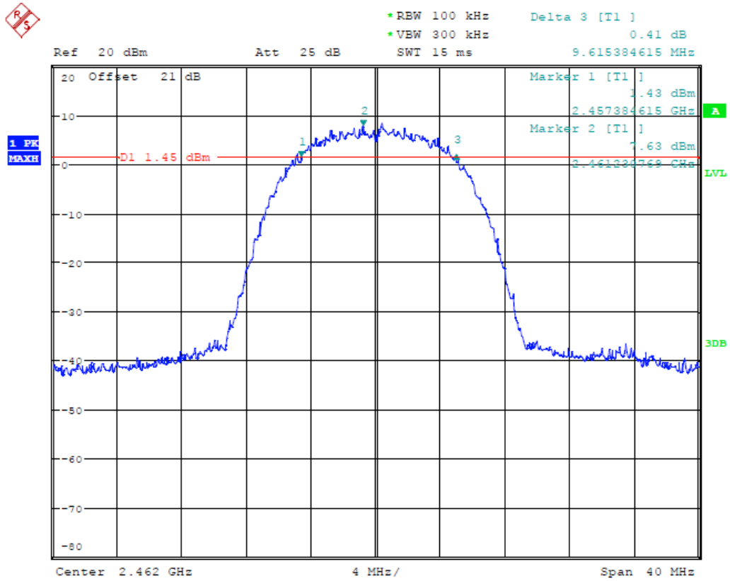
(Plot 4.7.1 C: Channel 11: 2462MHz @ 802.11b)
