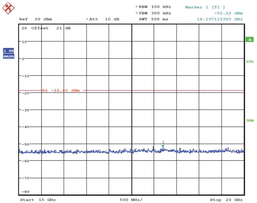
(Plot 4.6.2 A8: Channel 1: 2412MHz @ 802.11g)
