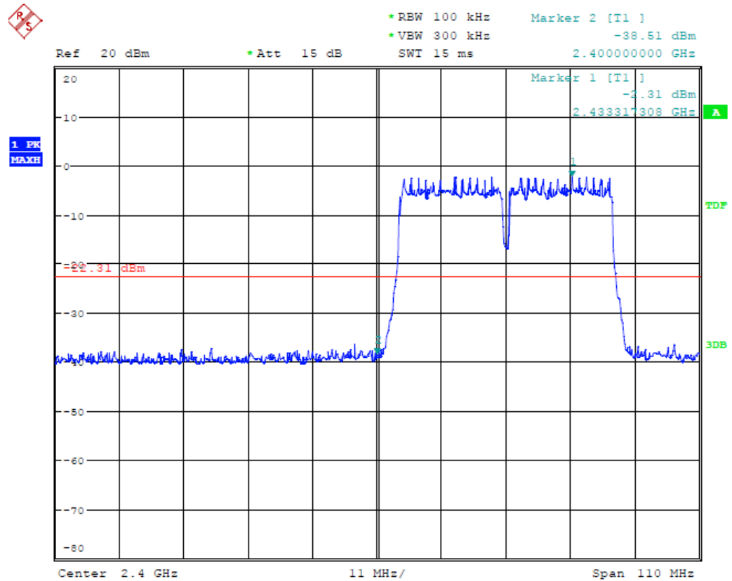
(Plot 4.6.4 D: Channel 1: 2412MHz @802.11n HT40)
