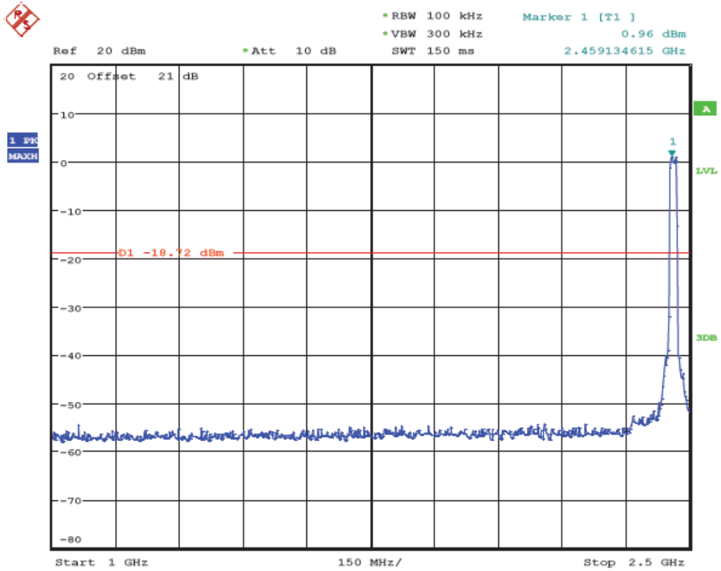
(Plot 4.6.3 C4: Channel 11: 2462MHz @ 802.11n HT20)
