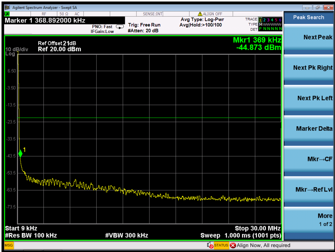
(Plot 4.6.3 C2: Channel 11: 2462MHz @ 802.11n HT20)
