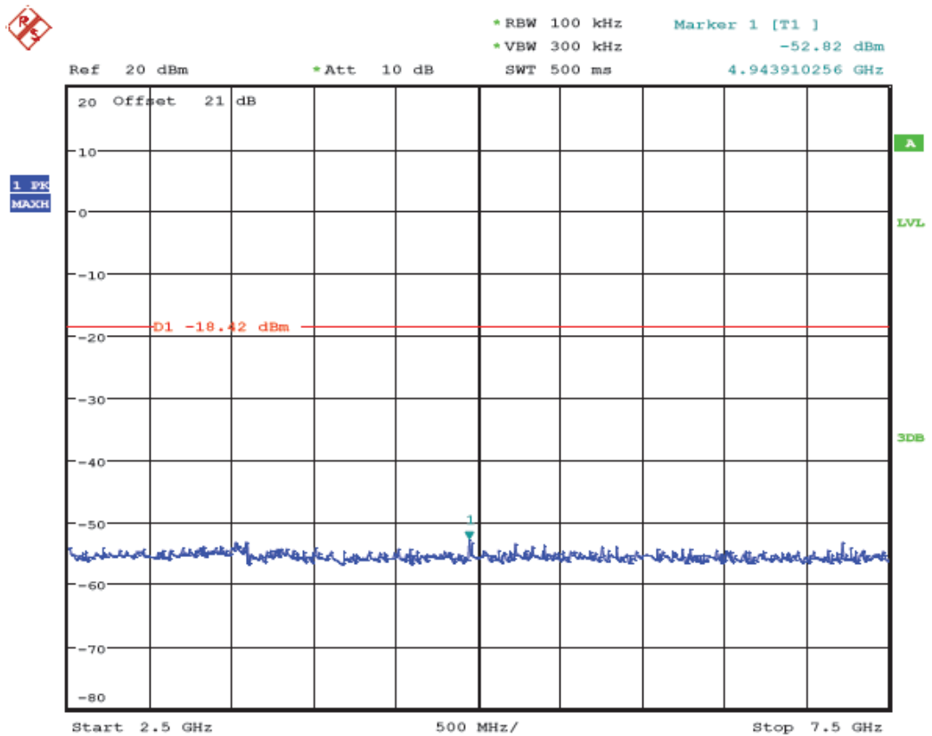
(Plot 4.6.3 A5: Channel 1: 2412MHz @ 802.11n HT20)
