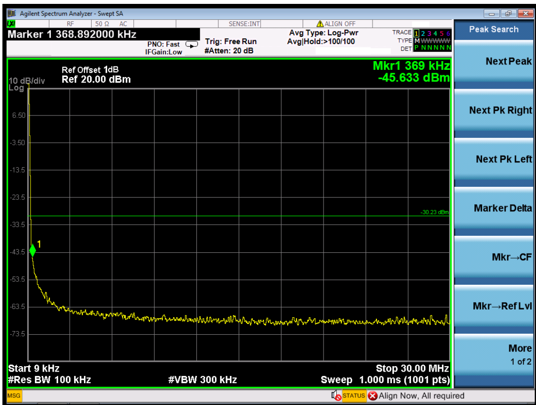
(Plot 4.6.4 A2: Channel 3: 2422MHz @ 802.11n HT40)
