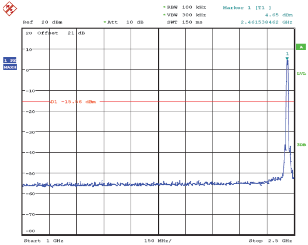
(Plot 4.6.1 C4: Channel 11: 2462MHz @ 802.11b)
