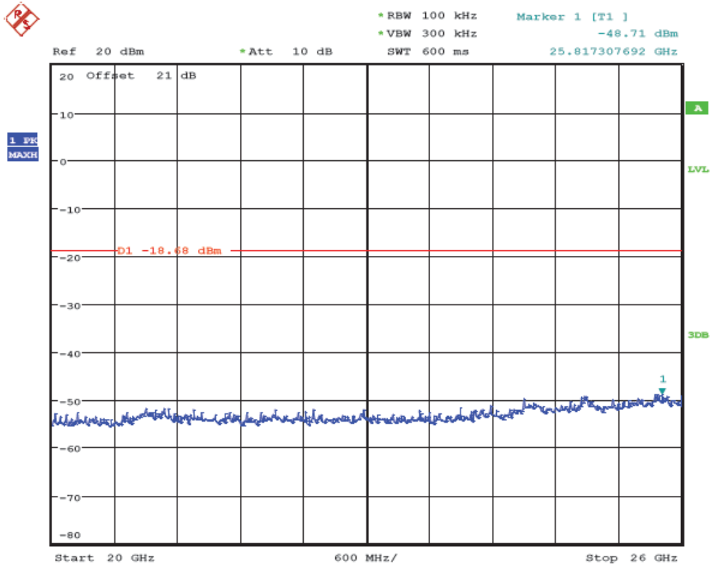
(Plot 4.6.2 C9: Channel 11: 2462MHz @ 802.11g)
