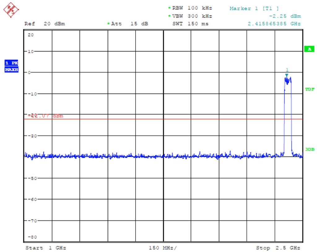
(Plot 4.6.4 A4: Channel 3: 2422MHz @ 802.11n HT40)
