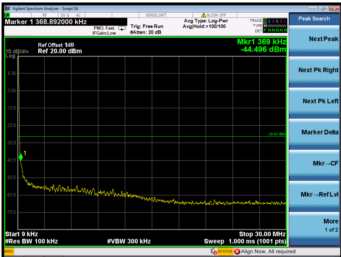
(Plot 4.6.4 C2: Channel 11: 2462MHz @ 802.11n HT40)
