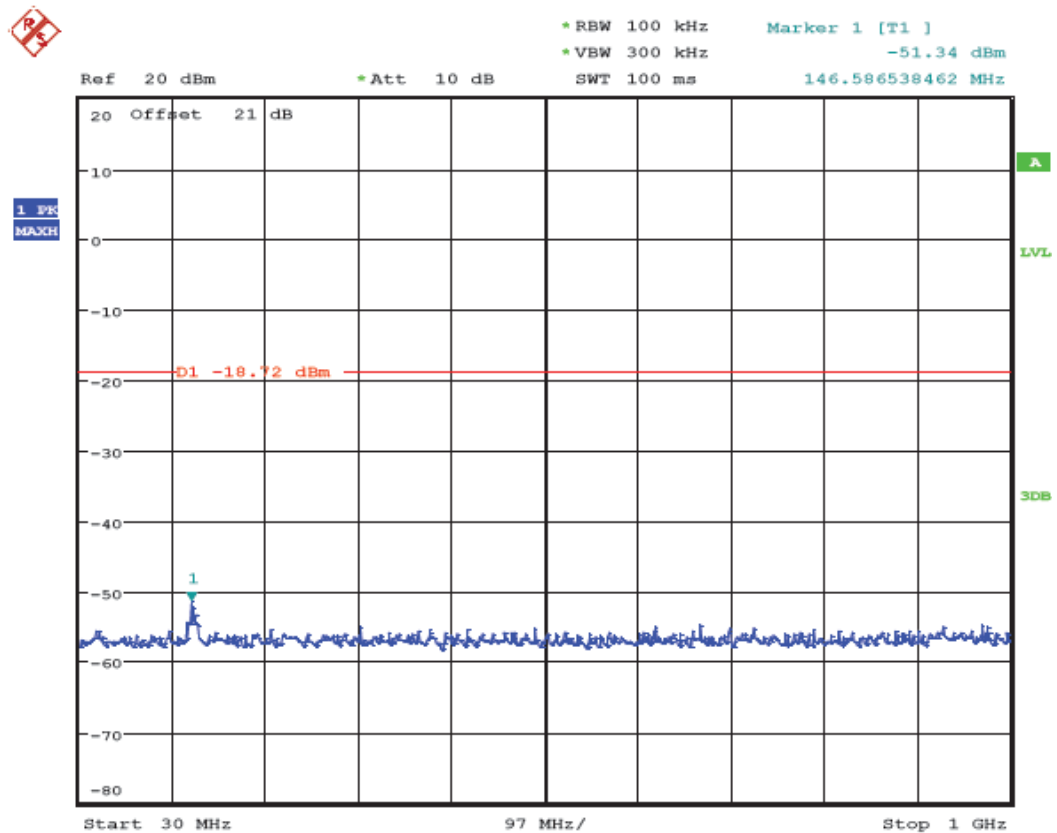
(Plot 4.6.3 C3: Channel 11: 2462MHz @ 802.11n HT20)
