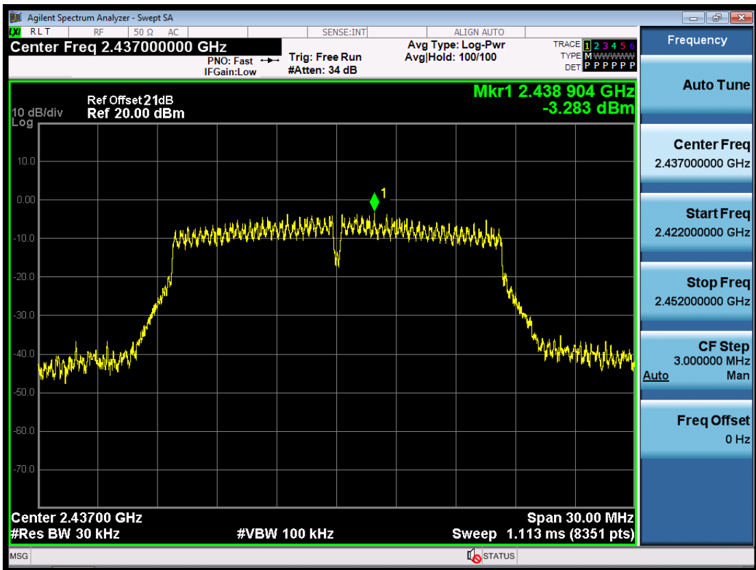
(Plot 4.4.2 B: Channel 6: 2437MHz @ 802.11g)
