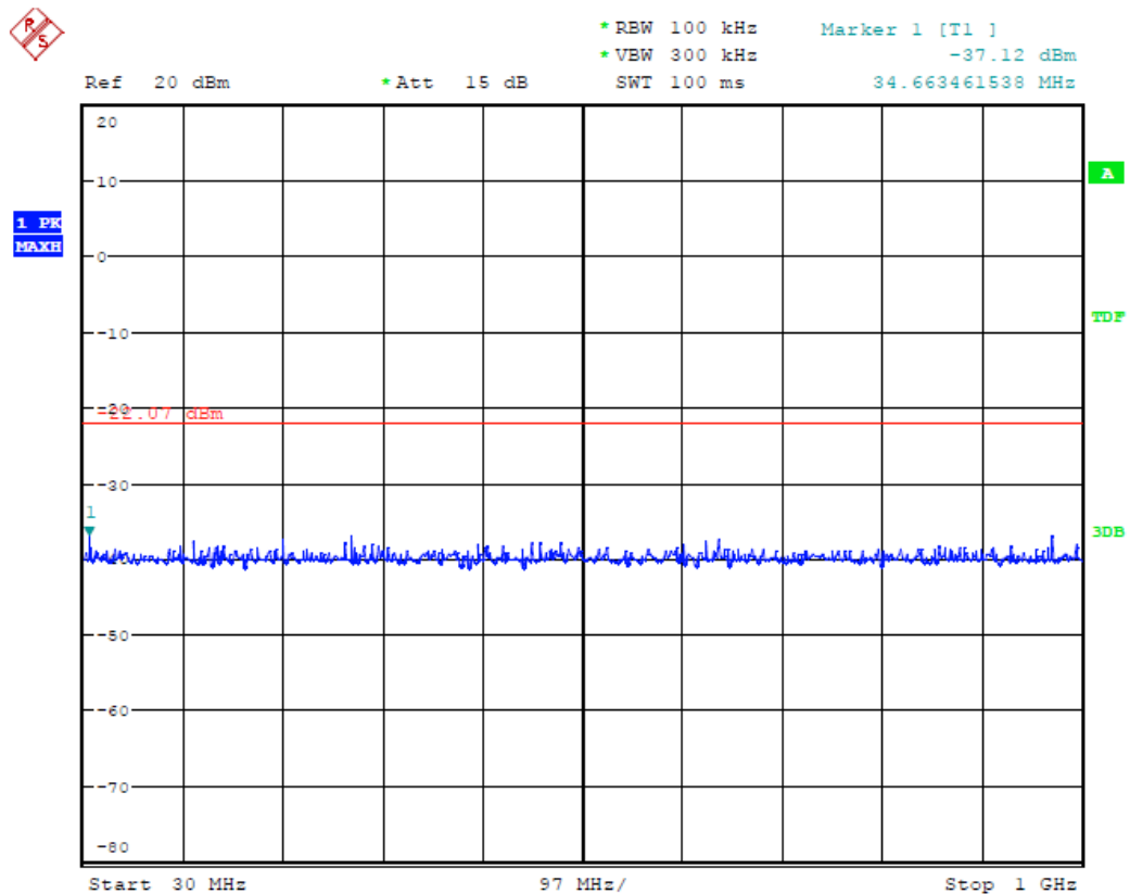
(Plot 4.6.4 B3: Channel 6: 2437MHz @ 802.11n HT40)
