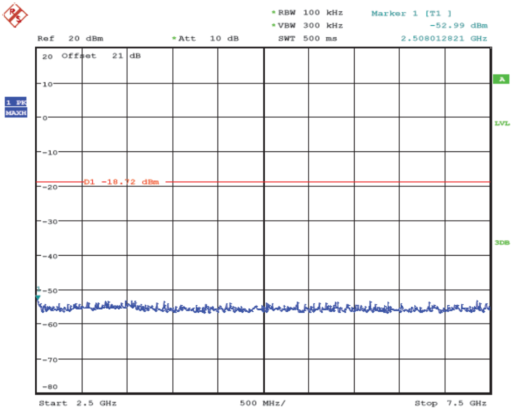
(Plot 4.6.3 C5: Channel 11: 2462MHz @ 802.11n HT20)
