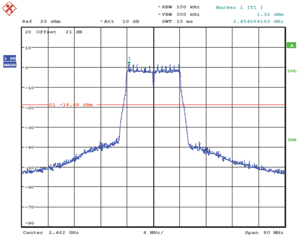
(Plot 4.6.2 C1: Channel 11: 2462MHz @ 802.11g)
