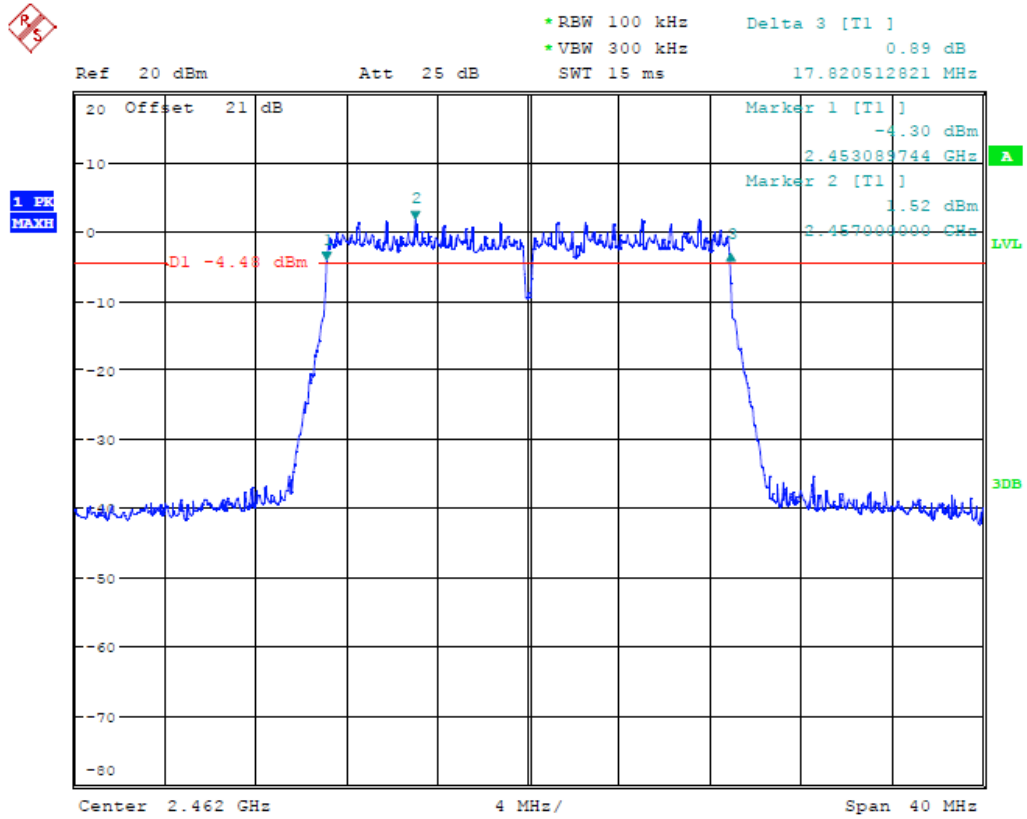
(Plot 4.7.3 C: Channel 11: 2462MHz @ 802.11n HT20MHz)
