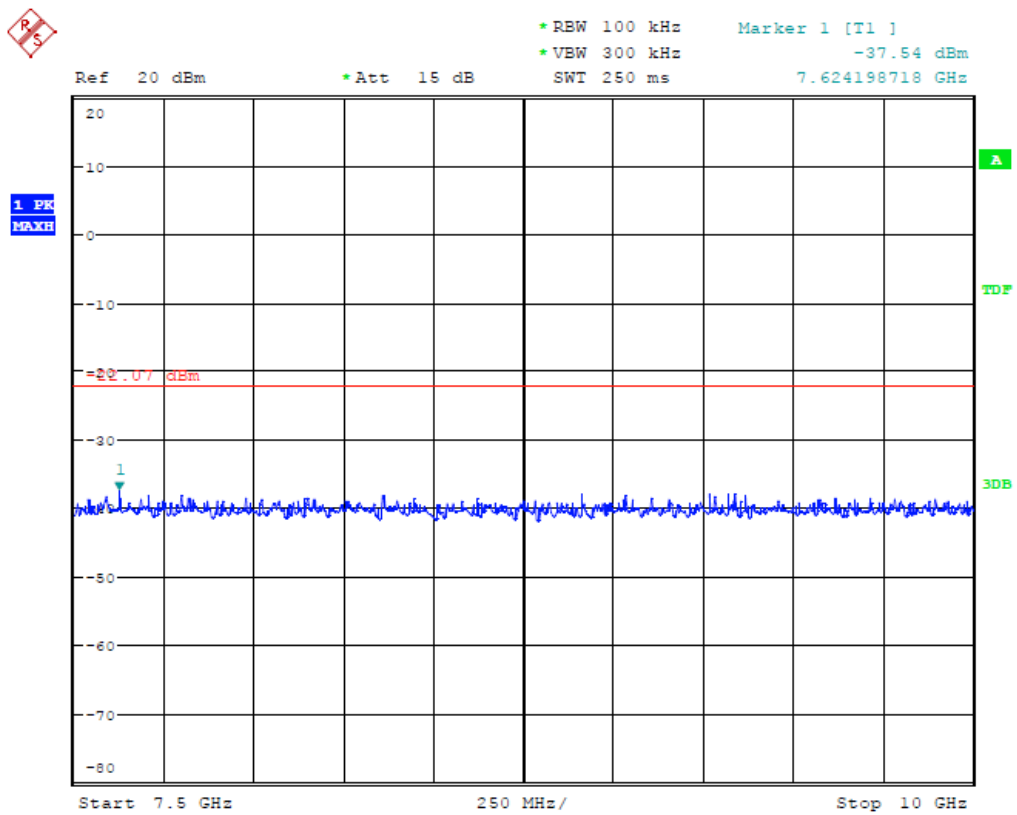
(Plot 4.6.4 A6: Channel 3: 2422MHz @ 802.11n HT40)
