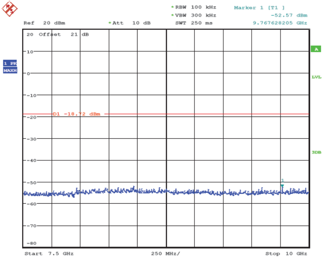
(Plot 4.6.3 C6: Channel 11: 2462MHz @ 802.11n HT20)
