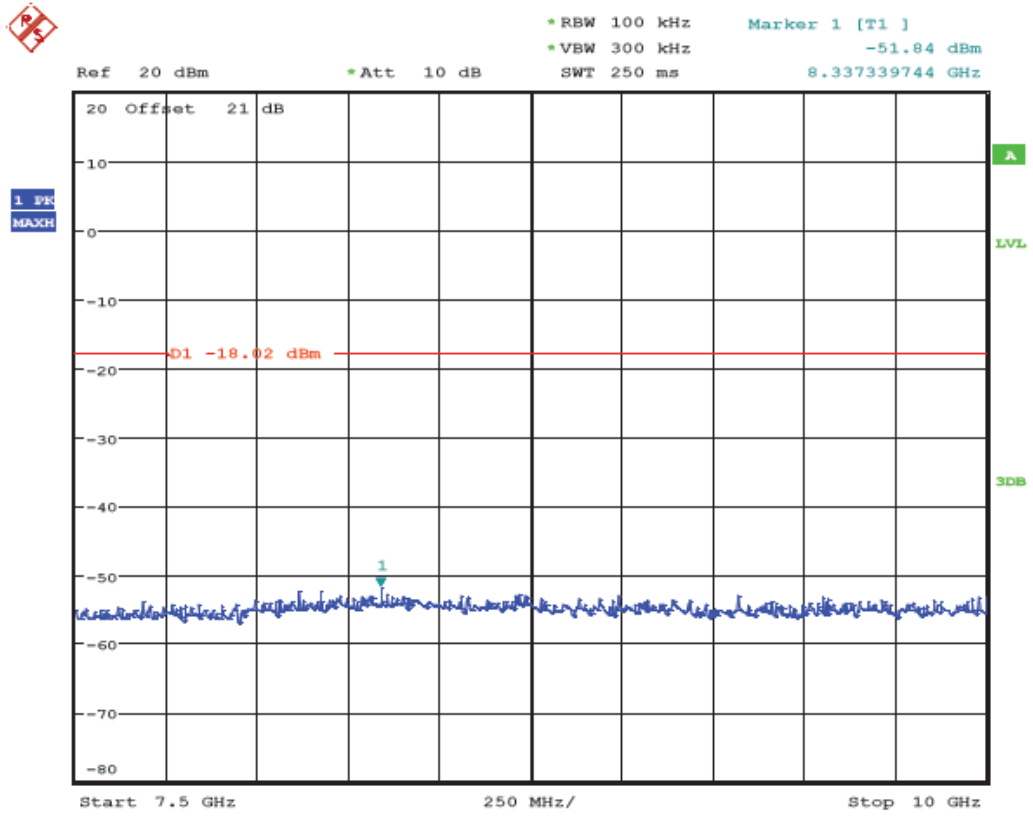
(Plot 4.6.2 B6: Channel 6: 2437MHz @ 802.11g)
