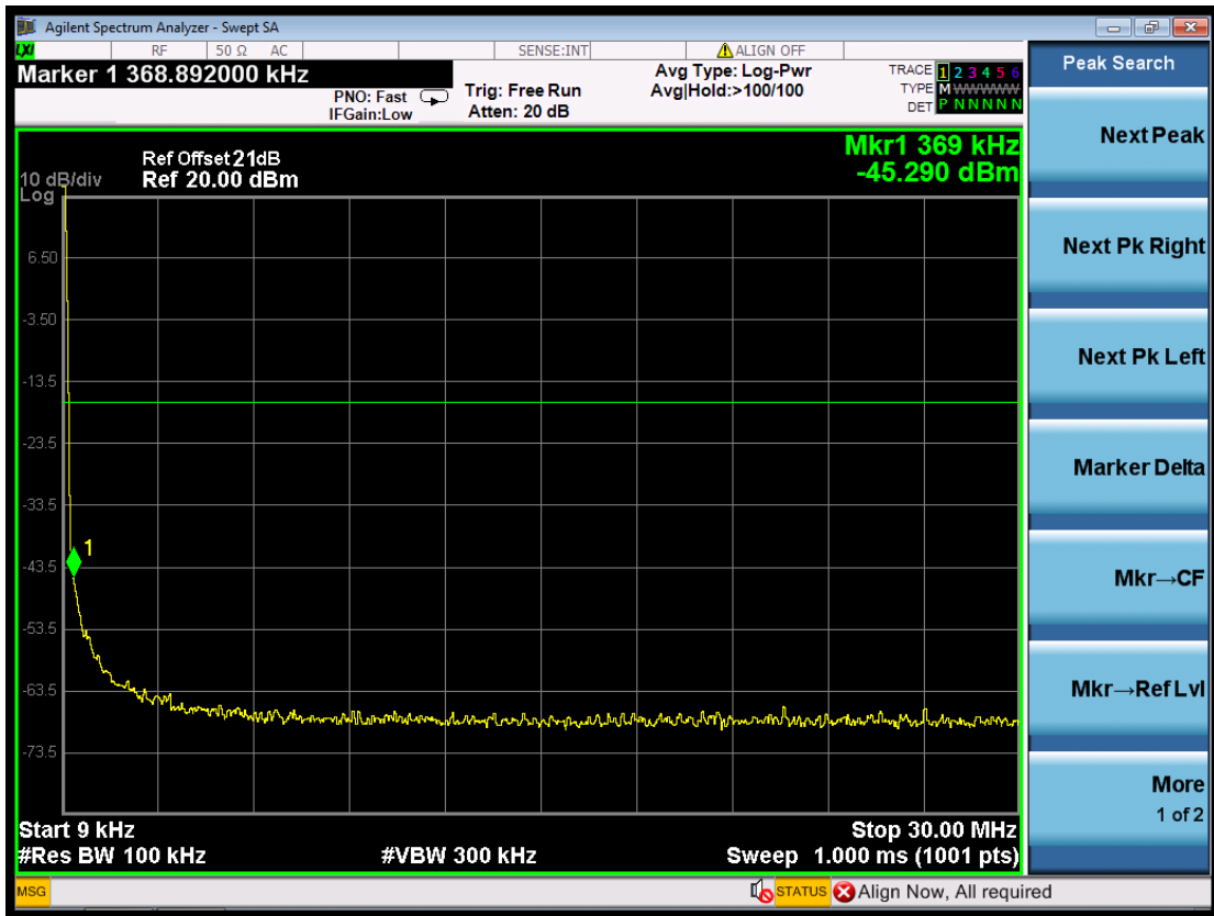
(Plot 4.6.1 C2: Channel 11: 2462MHz @ 802.11b)
