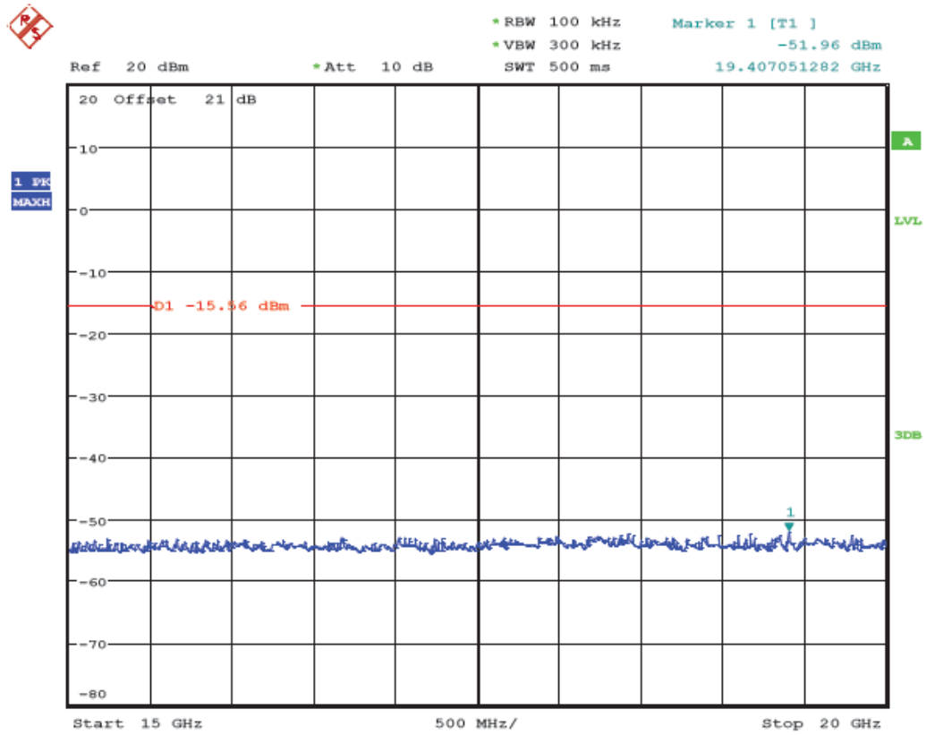
(Plot 4.6.1 C8: Channel 11: 2462MHz @ 802.11b)
