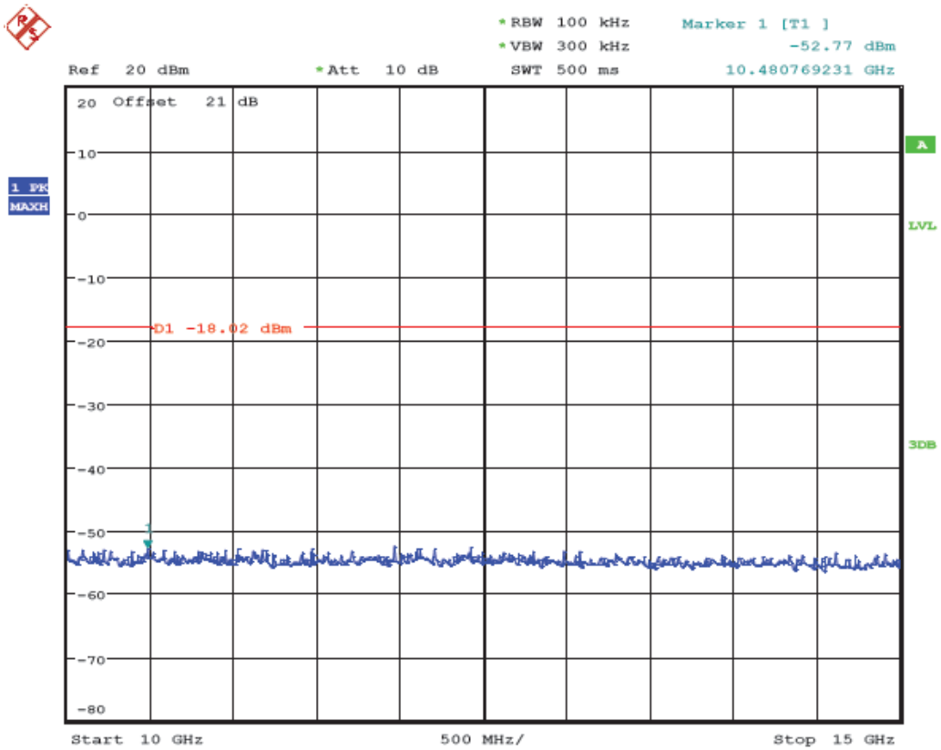
(Plot 4.6.2 B7: Channel 6: 2437MHz @ 802.11g)
