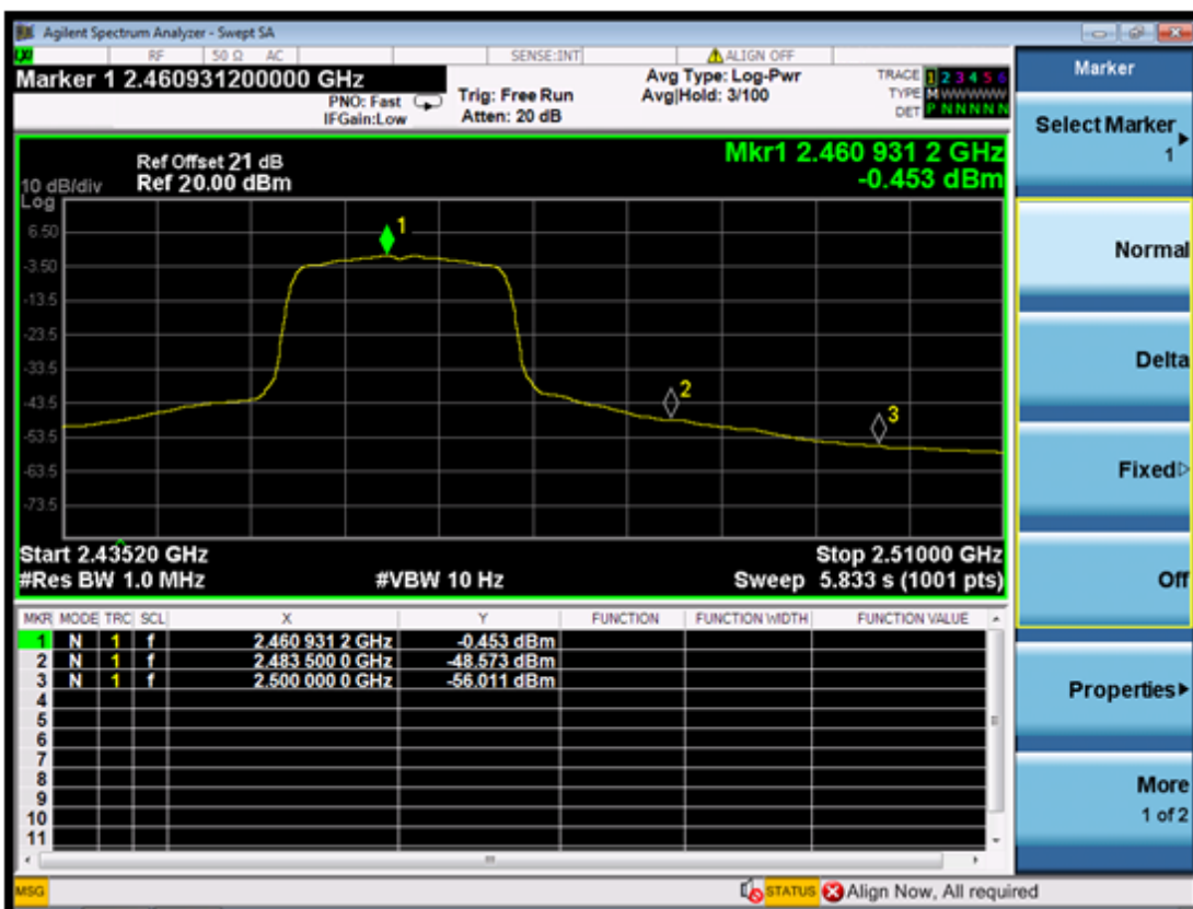
(Plot 4.5.2 A4: Channel 11: 2462MHz @ 802.11g)
