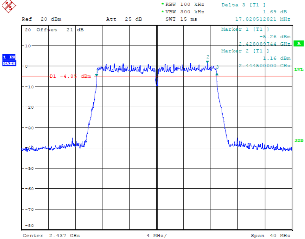
(Plot 4.7.3 B: Channel 6: 2437MHz @ 802.11n HT20)
