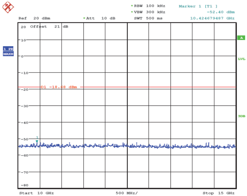
(Plot 4.6.2 C7: Channel 11: 2462MHz @ 802.11g)
