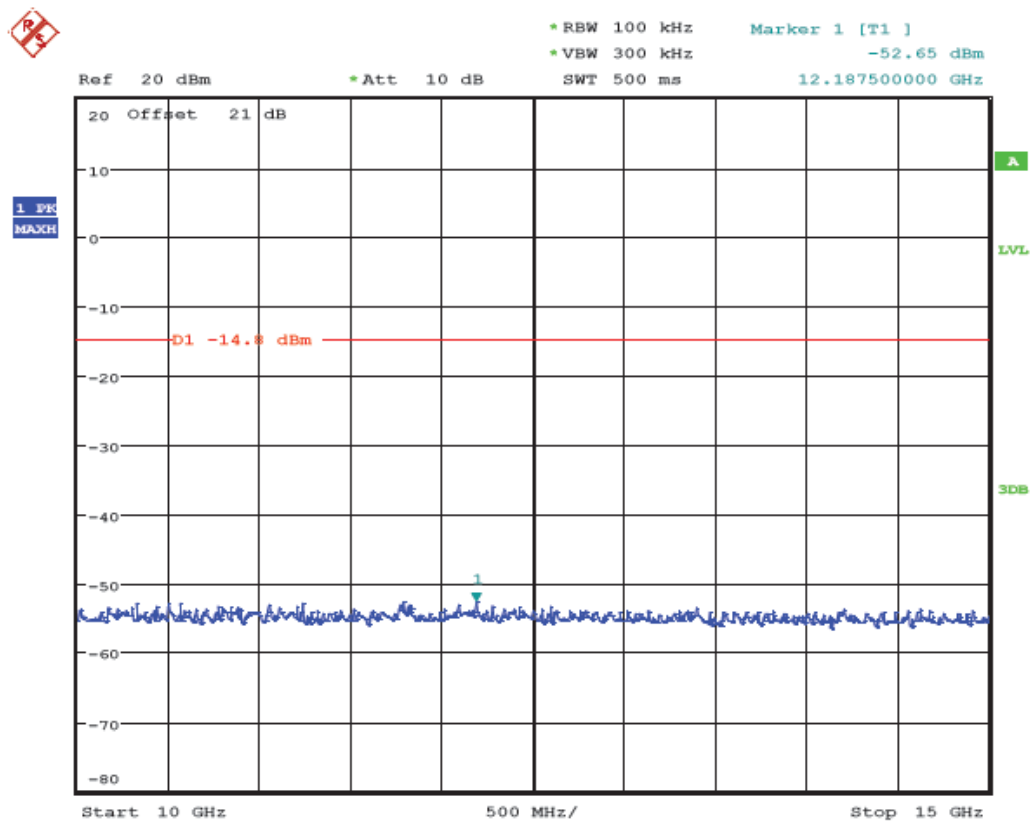
(Plot 4.6.1 A7: Channel 1: 2412MHz @ 802.11b)
