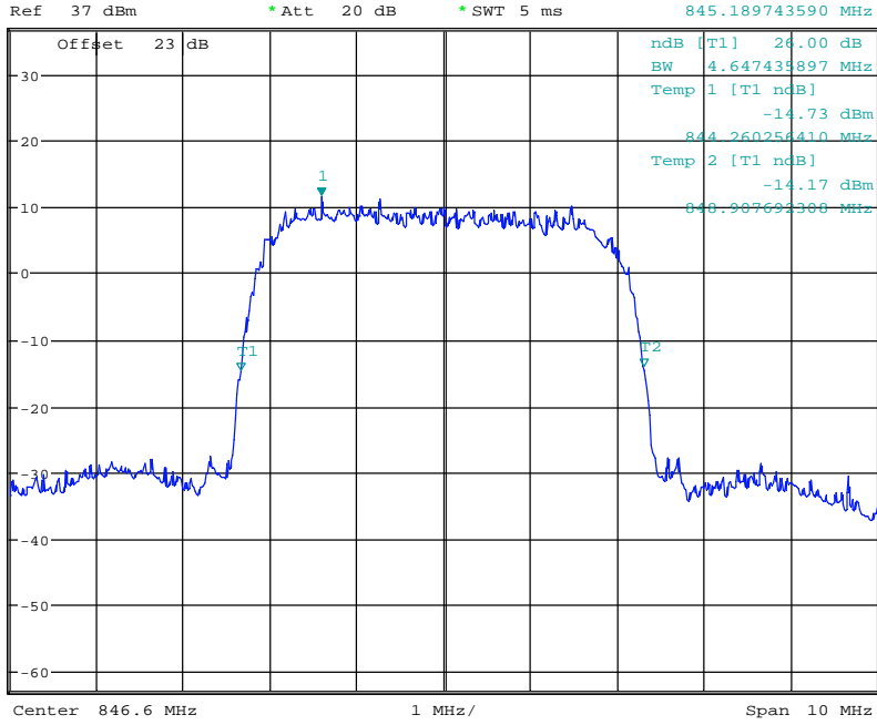
(Plot 4.4.2 C: Channel 4233:846.6MHz @ WCDMA Band V)
