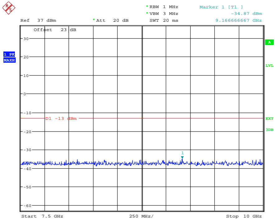
(Plot 4.6.2 C5: Channel 4233: 846.60 MHz @ WCDMA Band V)
