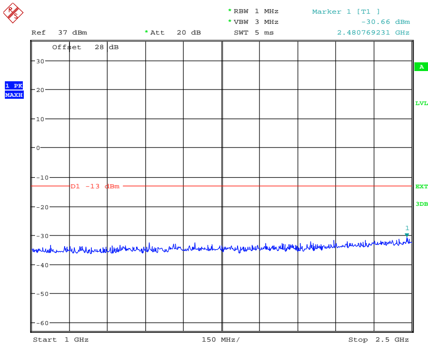
(Plot 4.6.2 D3: Idle @ PCS1900)
