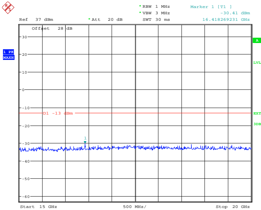
(Plot 4.6.2 A7: Channel 512: 1850.20MHz @ Traffic @ PCS1900)
