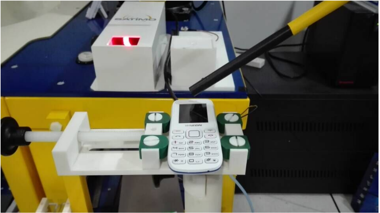
Fig.1 Testing Photo
