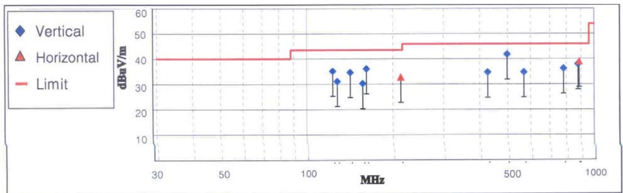
< Fig 7. Radiated emission result >
