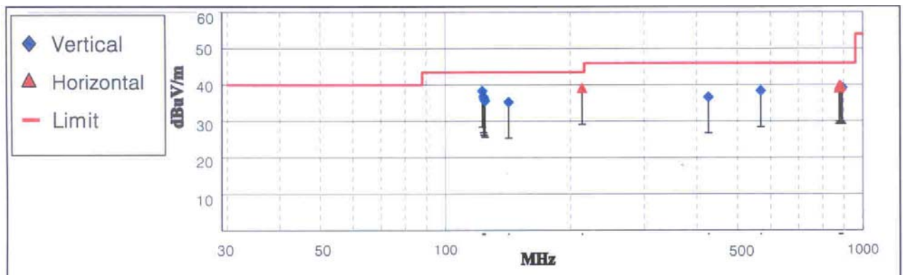
< Fig 5. Radiated emission result >
