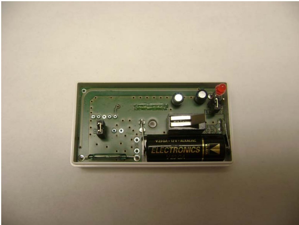
Figure 1 Circuit Board top side
