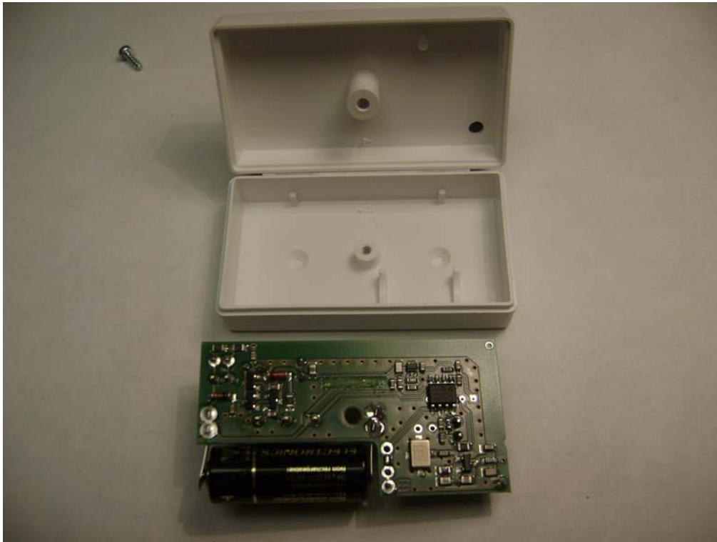
Figure 3 Bottom side
