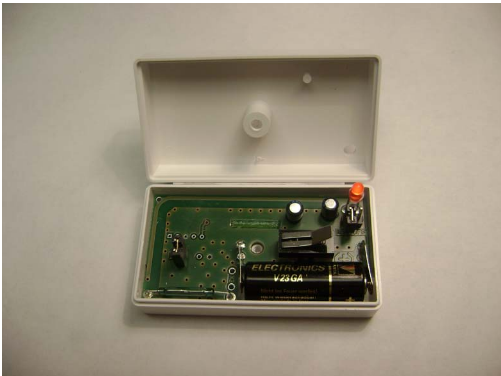
Figure 2 Top side
