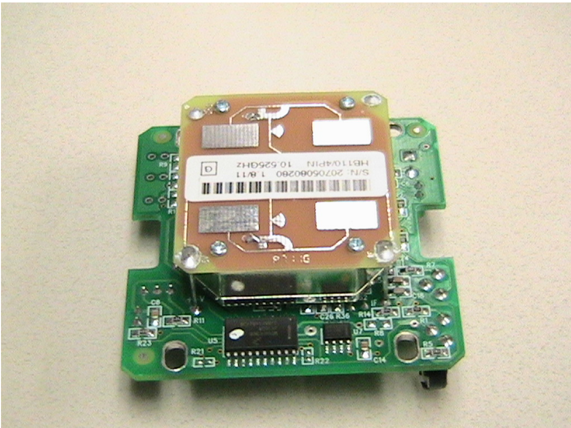
Larco Model 336806 - Sensor View 2
