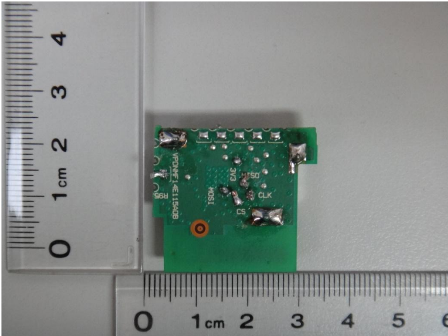
BTM01 Back View
