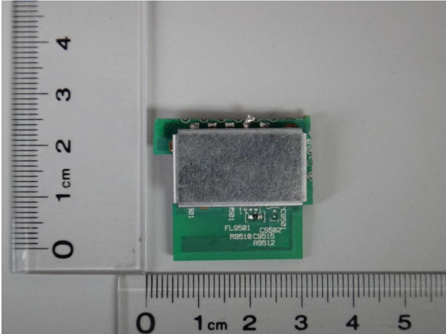
BTM01 Front View
