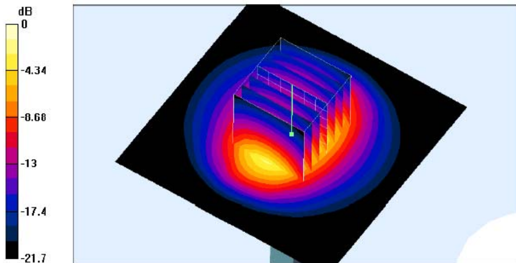
0 dB = 6.29mW/g
