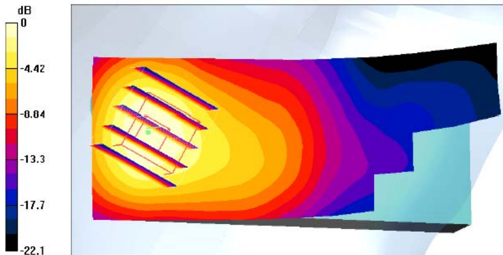
0 dB = 0.221mW/g
