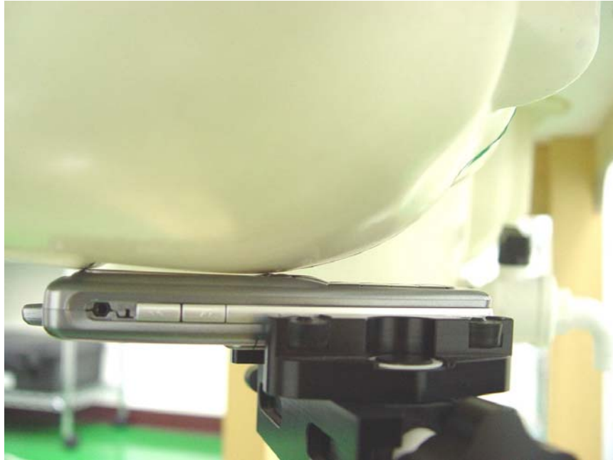
Fig. 9.3 Right Cheek
