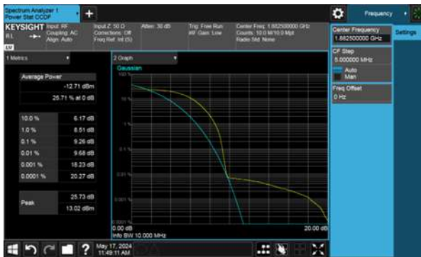
Test Mode: Band 25 QPSK 20MHz CH26365
