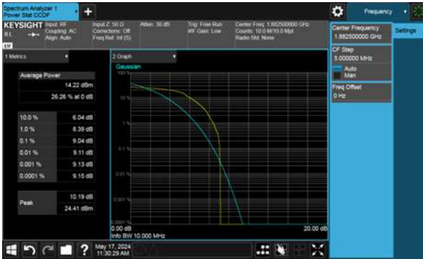
Test Mode: Band 25 QPSK 15MHz CH26365
