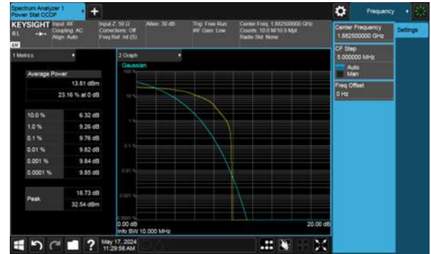
Test Mode: Band 25 16QAM 15MHz CH26365
