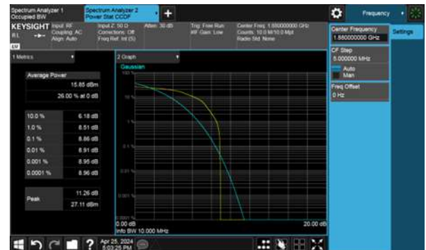
Test Mode: Band 2 16QAM 5MHz CH18900
