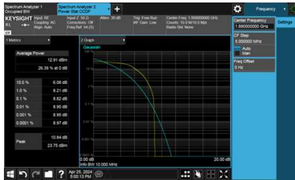
Test Mode: Band 2 QPSK 20MHz CH18900
