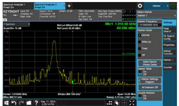
Test Mode: QPSK Band 2 20M CH19100-1 @MAX
