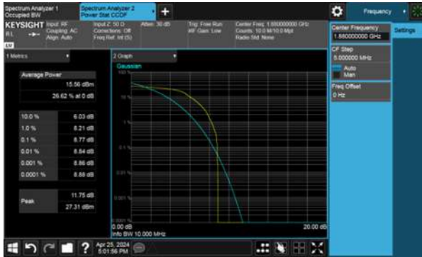
Test Mode: Band 2 QPSK 15MHz CH18900
