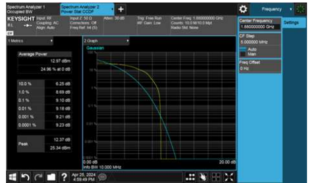
Test Mode: Band 2 16QAM 20MHz CH18900
