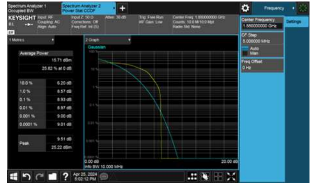
Test Mode: Band 2 16QAM 15MHz CH18900
