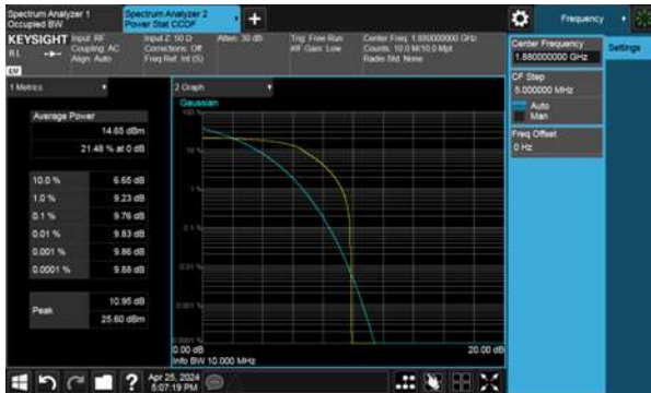
Test Mode: Band 2 QPSK 3MHz CH18900
