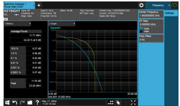
Test Mode: Band 25 16QAM 20MHz CH26365
