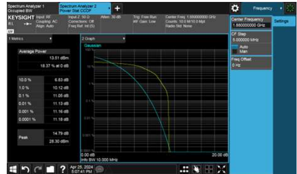
Test Mode: Band 2 16QAM 3MHz CH18900
