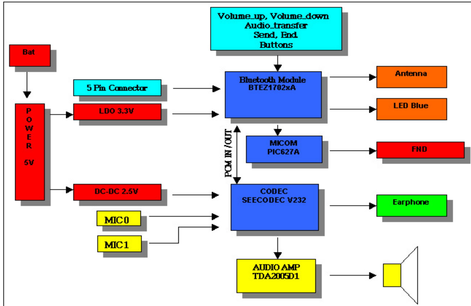
[Fig 1.1 ] Block Diagram for Vossor
