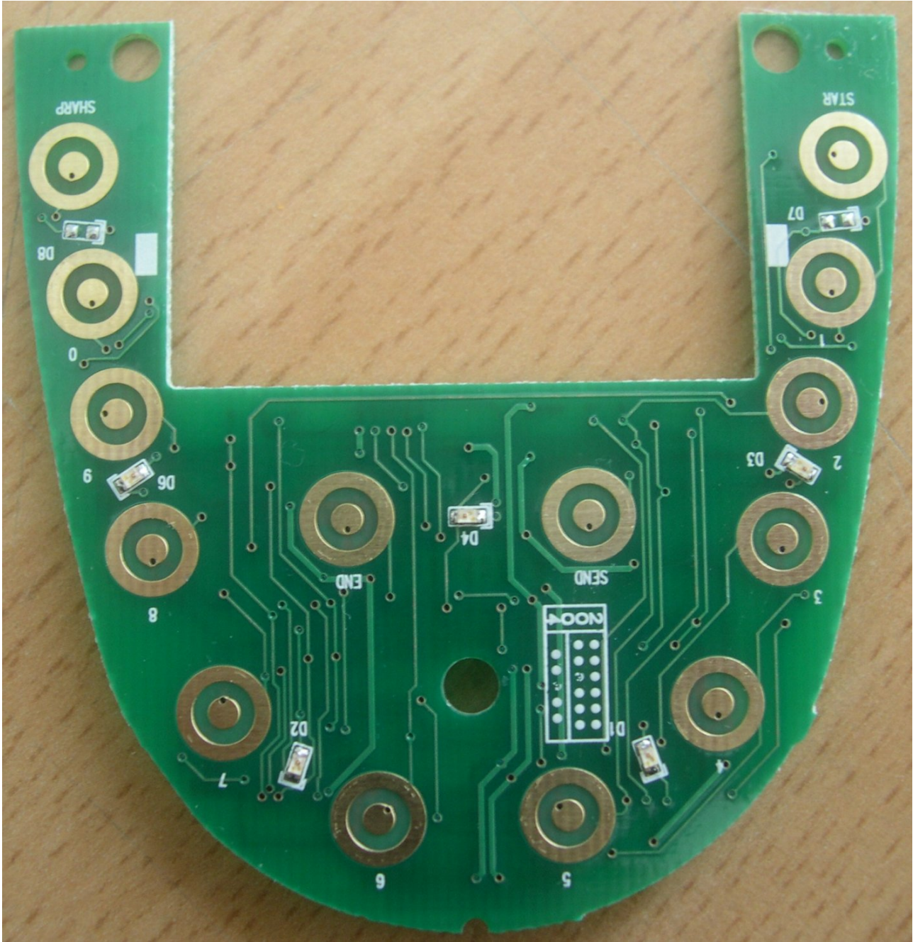
<Photograph 5: Rear View - Keyboard>
