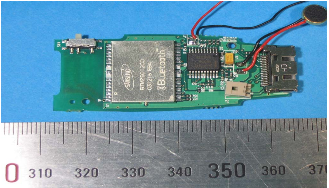
1.7 The Front side of PCB for Headset
