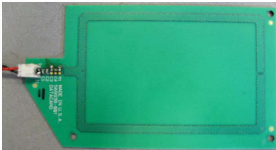
Figure 3: Antenna circuit
