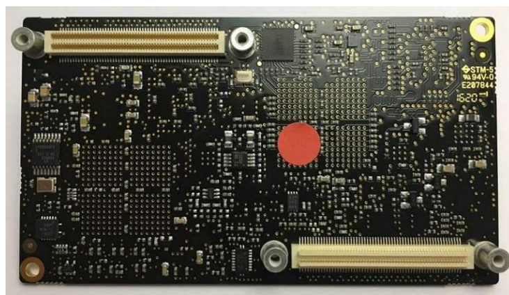
US-NANO board (bottom)
