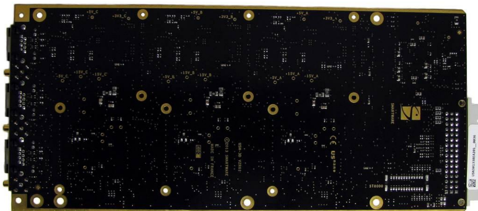
USN-3D board (bottom view) (USN3se)
