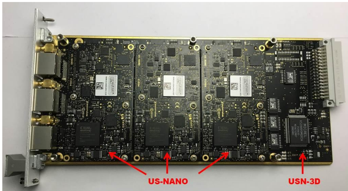
USN-3D board equipped with 3 US-NANO boards without shielding
