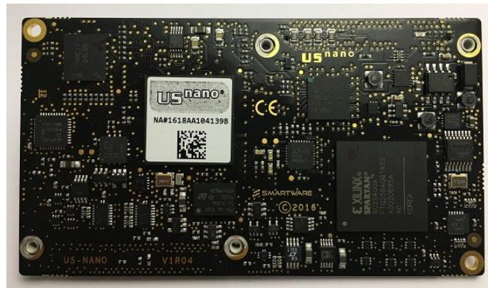
US-NANO board (top)
