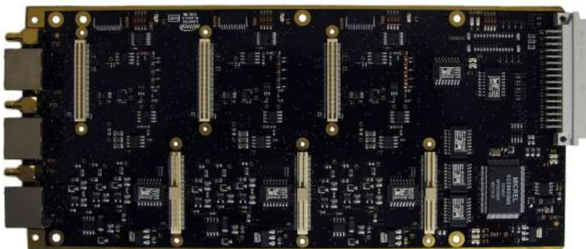
MX3e-3I3P top view without US-nano daughterboards (RF)
