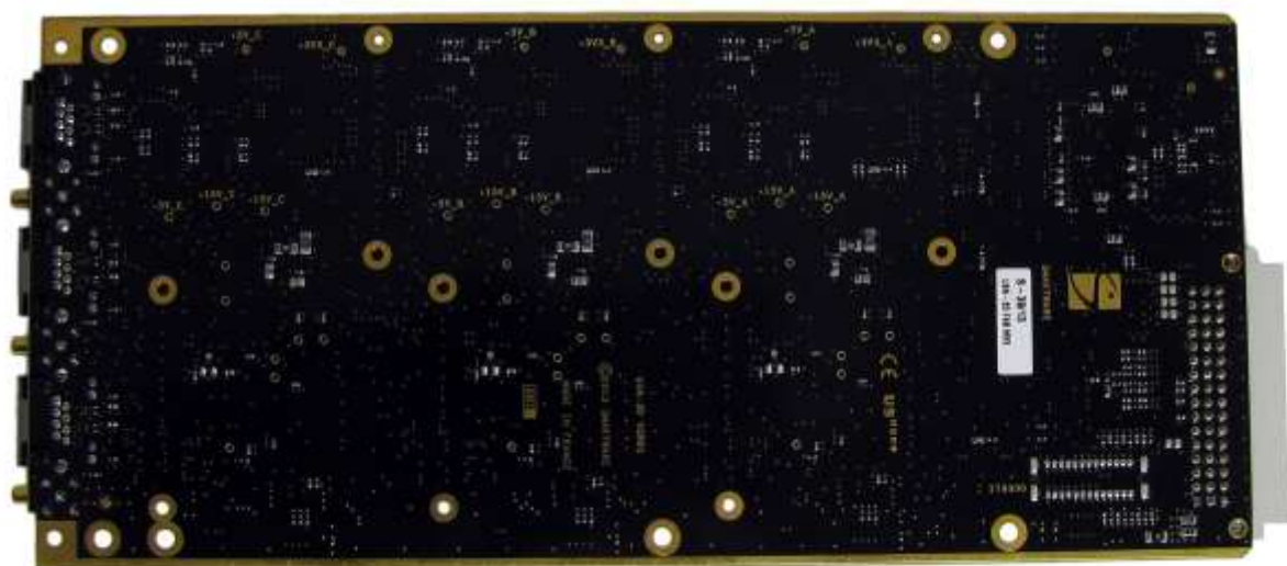
MX3e-3I3P bottom view
