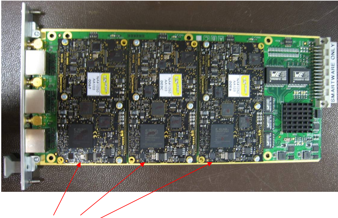
USnano board (TOP view)
