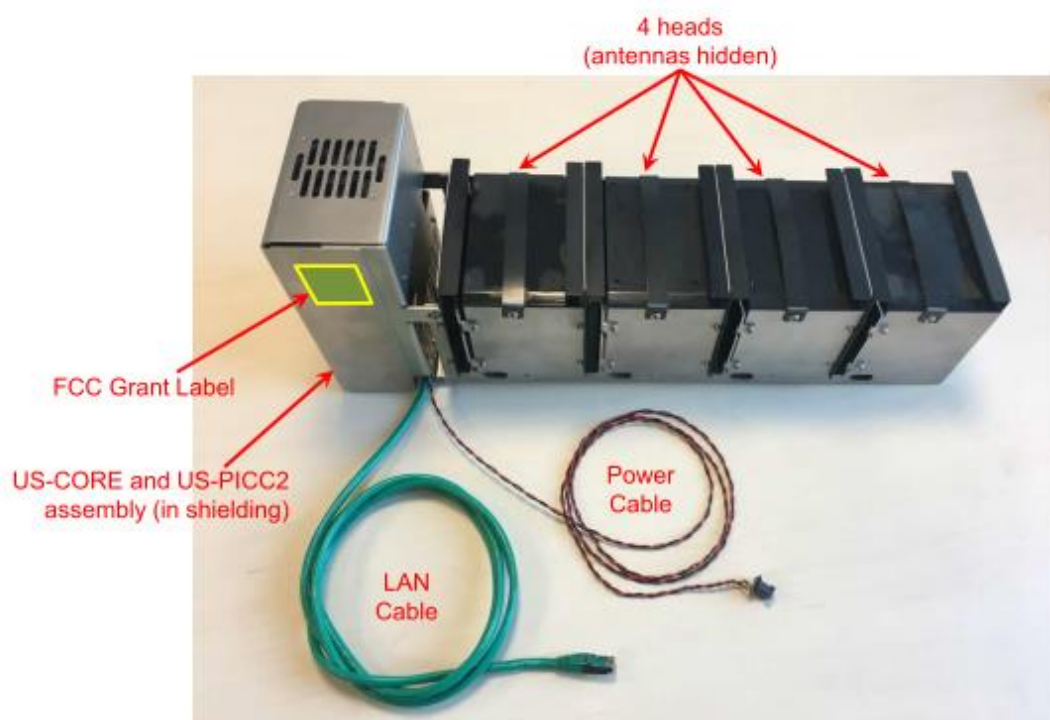
Fig. 1: Passport Station chassis picture.
