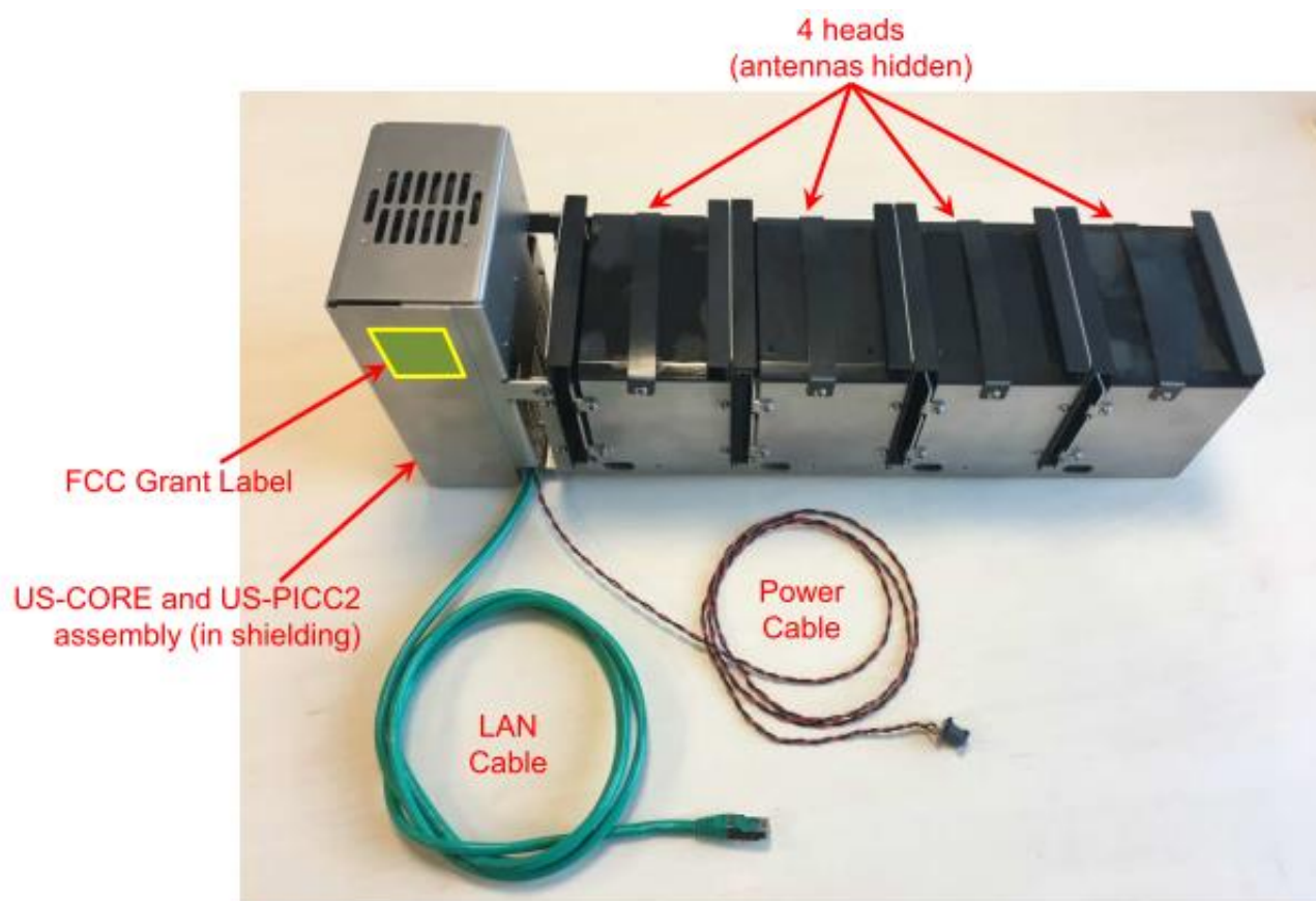
Fig. 1: Passport Station chassis picture.
