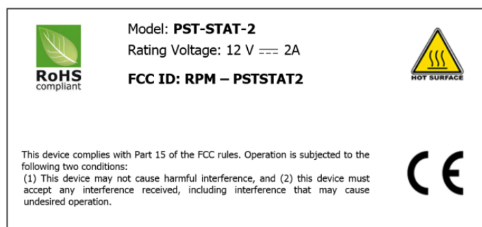
Fig. 16: View of label (45×21 mm approx.).
