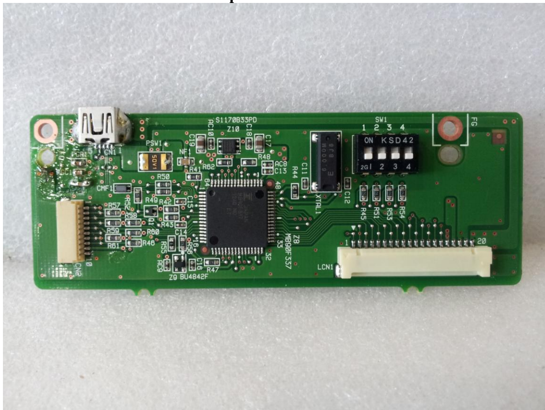
Top of Main Board
