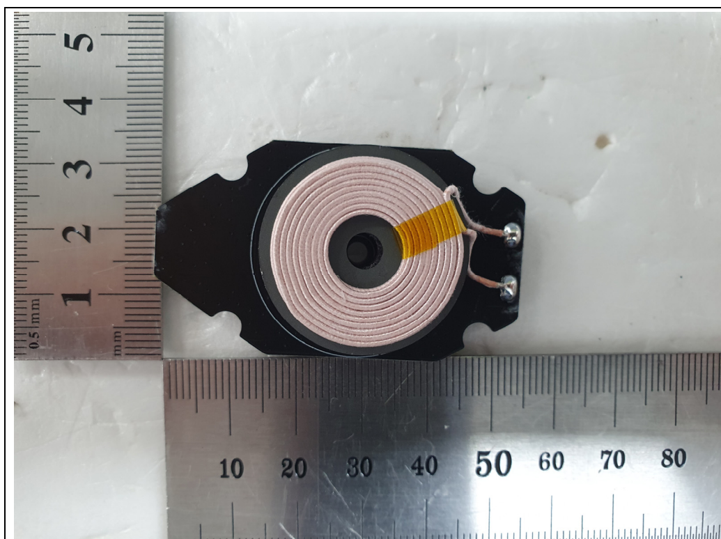
<Coil Antenna>
