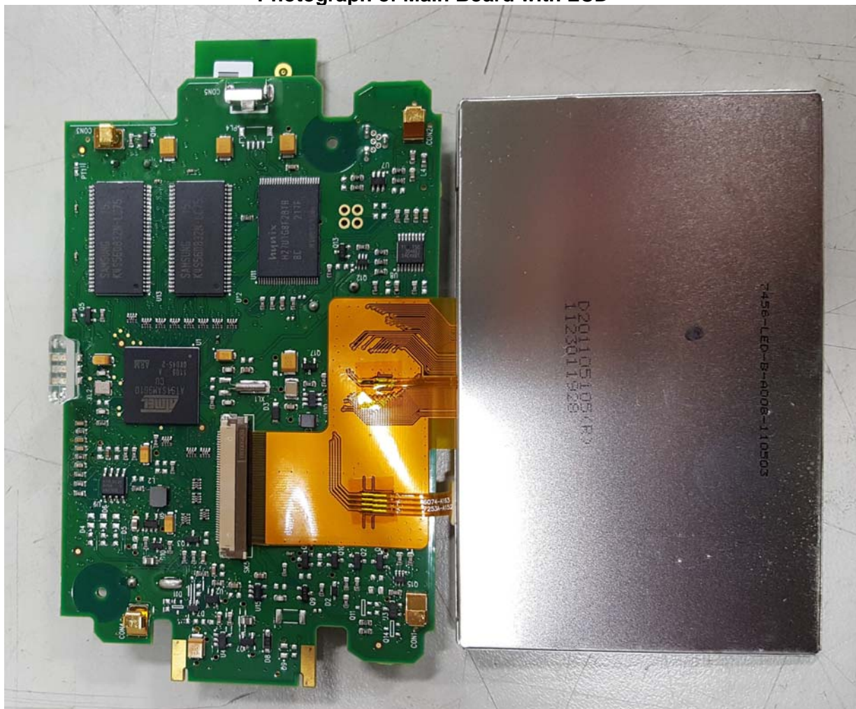
Photograph of Main Board with LCD
