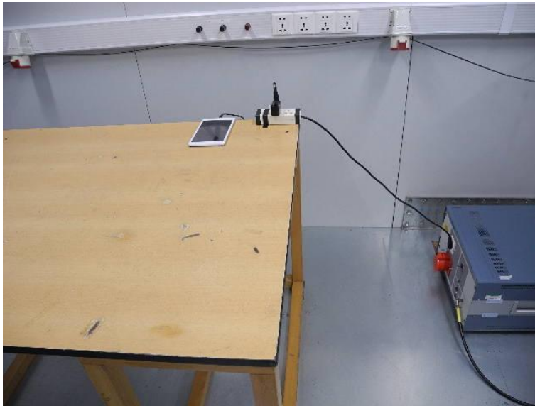
AC Conducted Emission Test Setup
