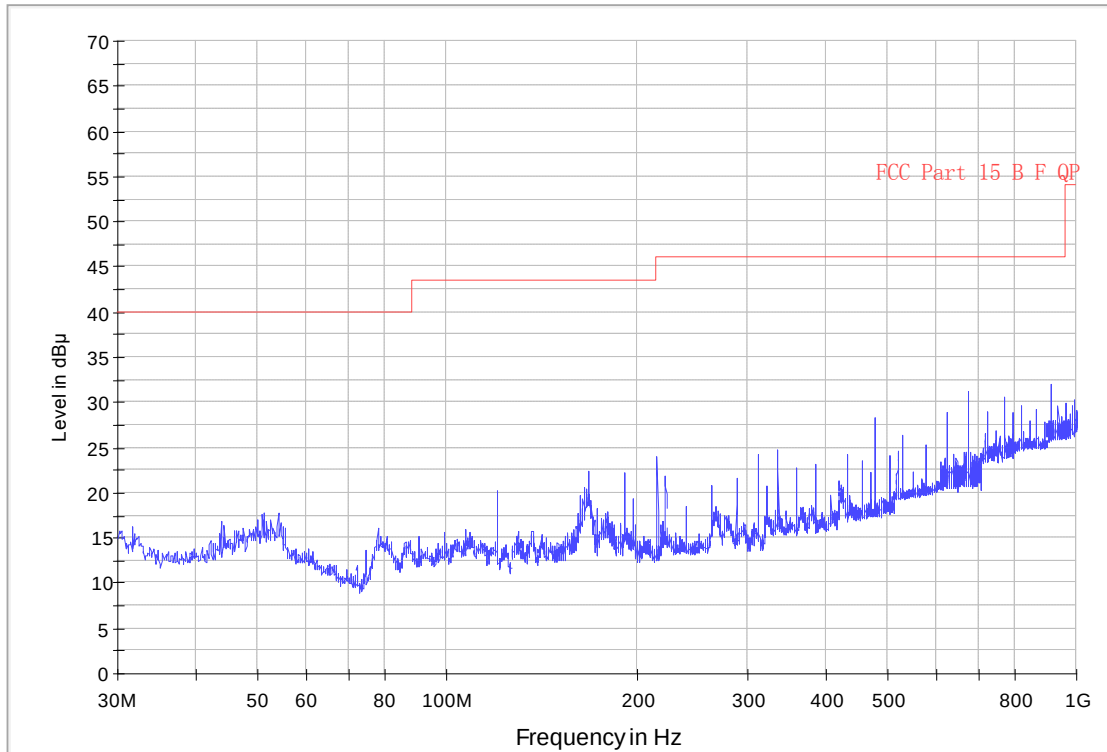
Field strength 30M-1GHz 1F 3m chamber
