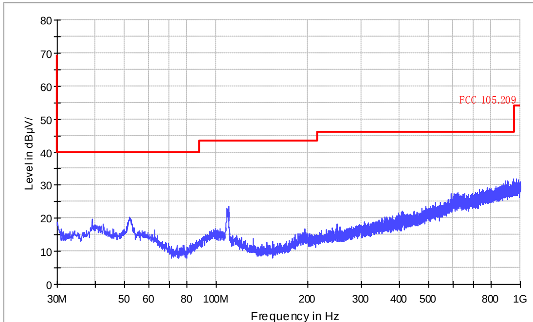
Electric Field Strength 30M-1GHz
