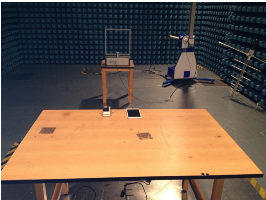
FCC Part 22H/24E Radiated Emission 9K-30MHz
