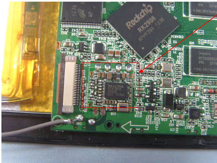
Wifi module front view
