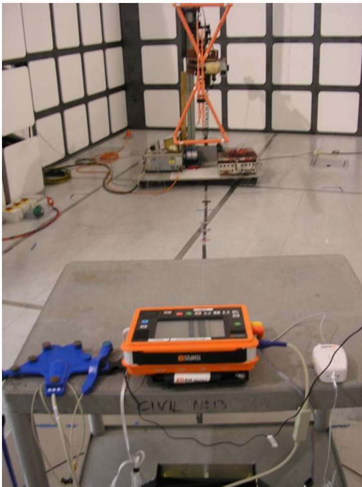
Radiated Emissions (Enclosure Port) Test Setup
