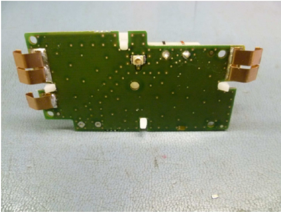
GSM antenna Top and Bottom Views
