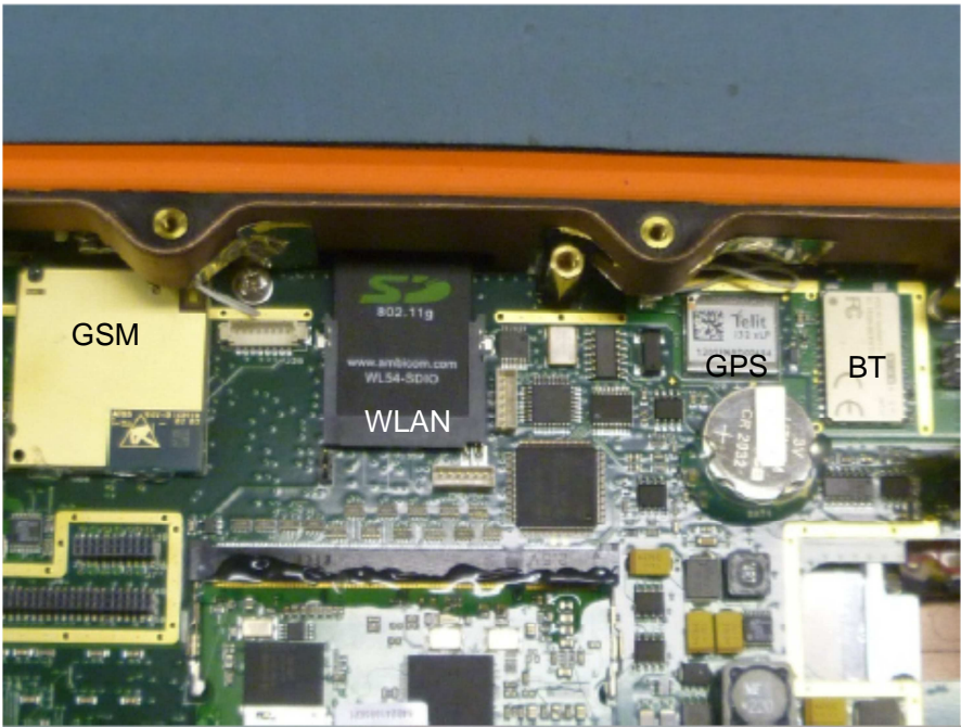
Location of all radio modules in Tempus IC host
