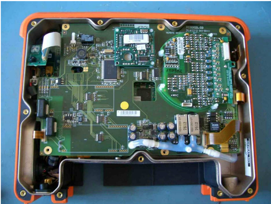
TempusIC host internal view 2 (showing radio module positions)
