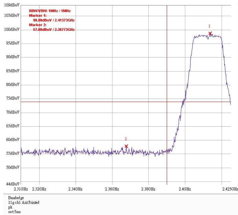
Band edge @ 802.11g mode channel 1 PK
