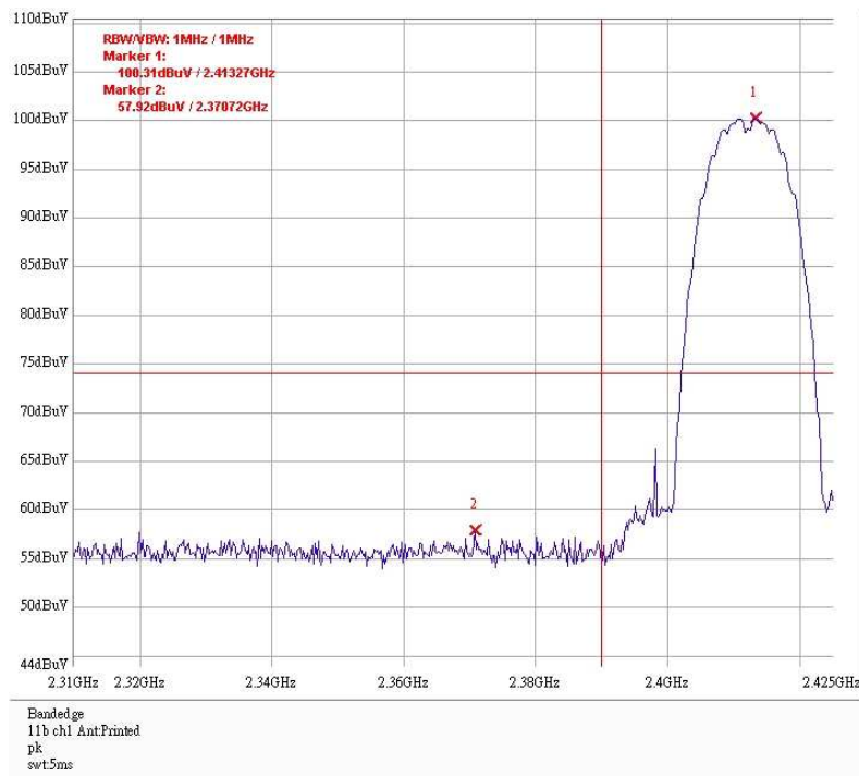
Band edge @ 802.11b mode channel 1 PK
