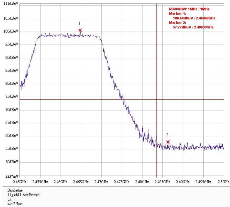
Band edge @ 802.11g mode channel 11 PK
