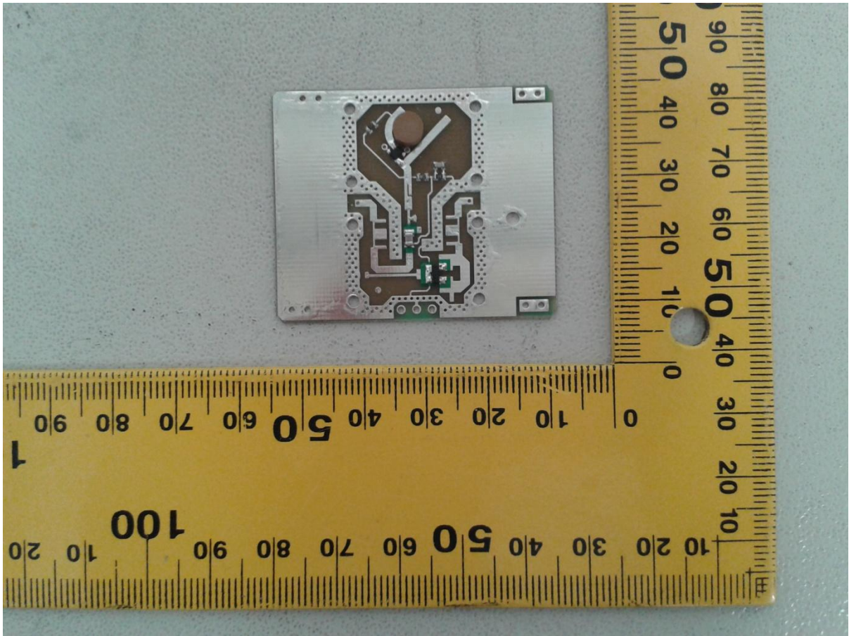
MDU2750L internal (can removed) photo
