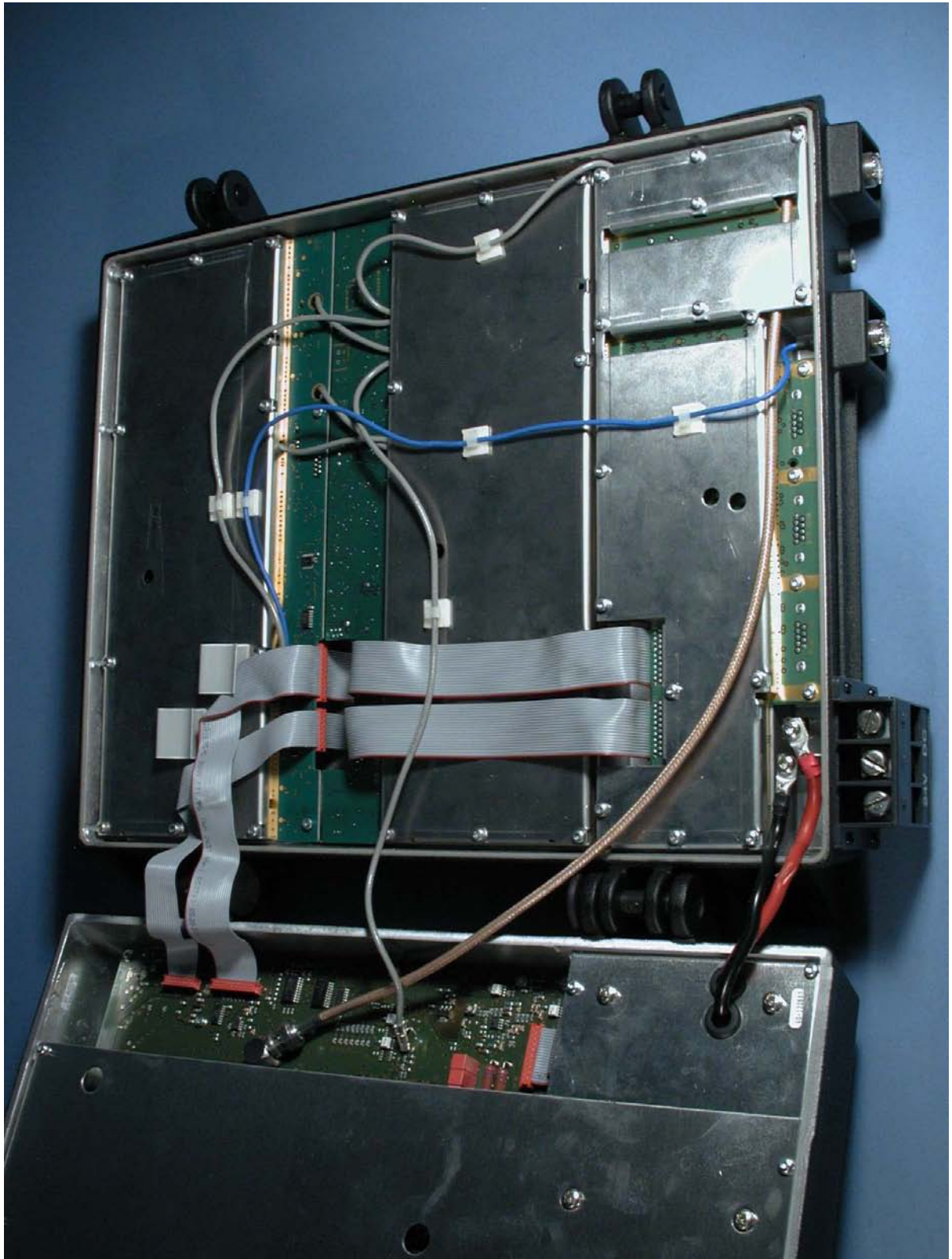
Photograph 1: Transceiver unit, SAILOR TU5160, internal view
