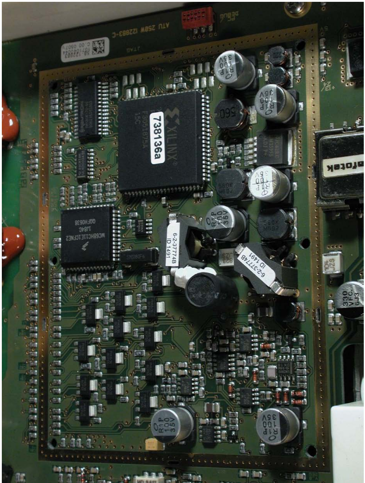
Photograph 9: Antenna tuner unit SAILOR ATU5215 Processor and memory
