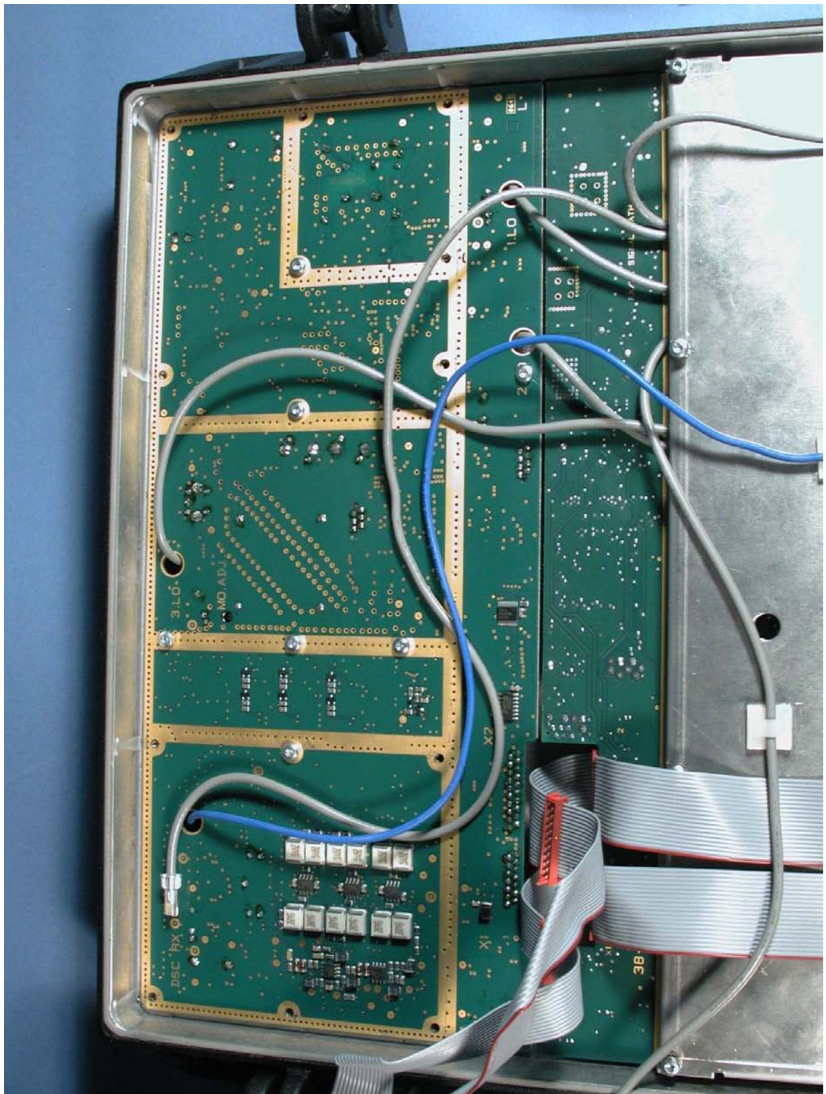
Photograph 5: Transceiver unit, SAILOR TU5160, Synth. and DSC WR 122879 Module
