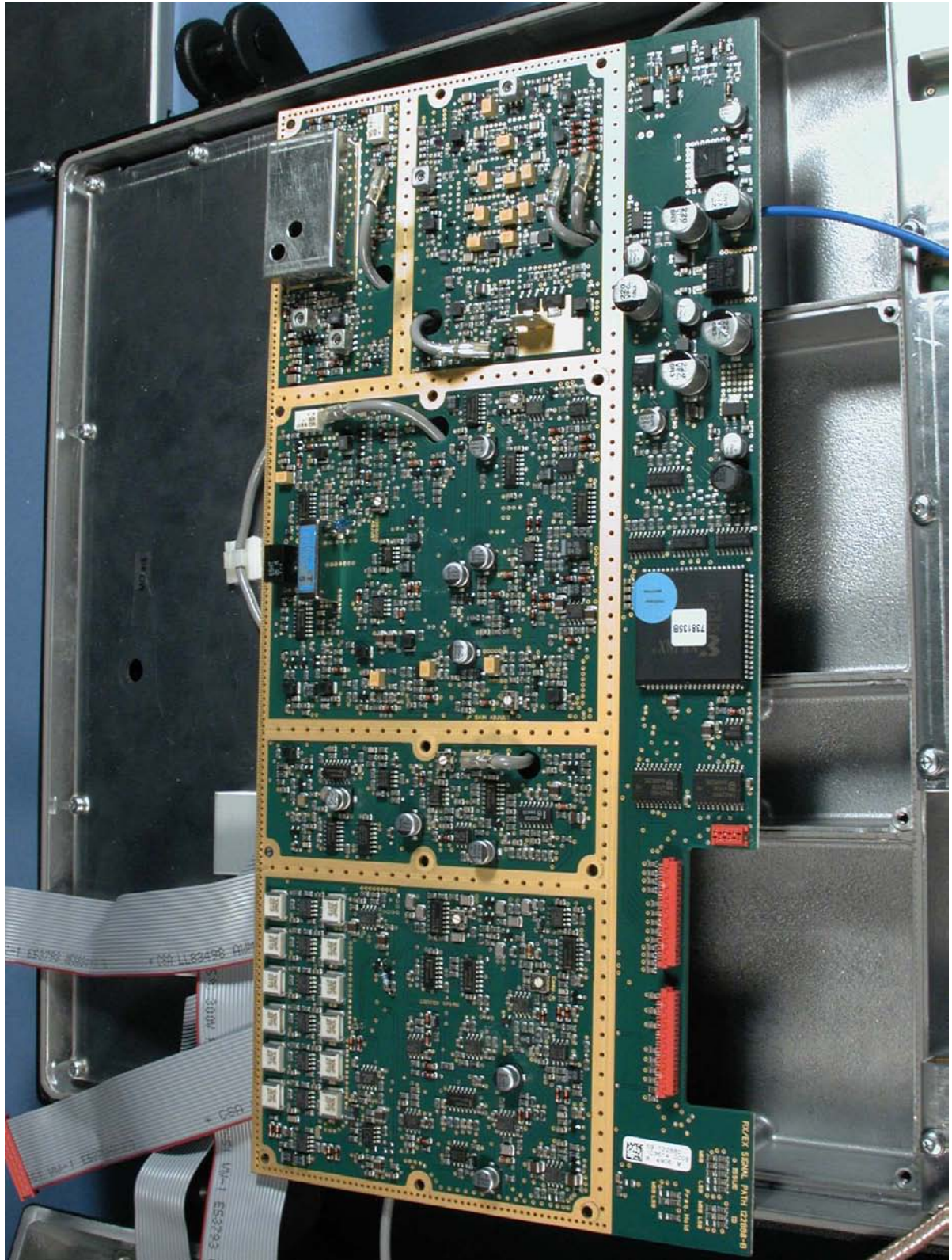
Photograph 4: Transceiver unit, SAILOR TU5160, Rx/Ex Signal Path 122880 Module
