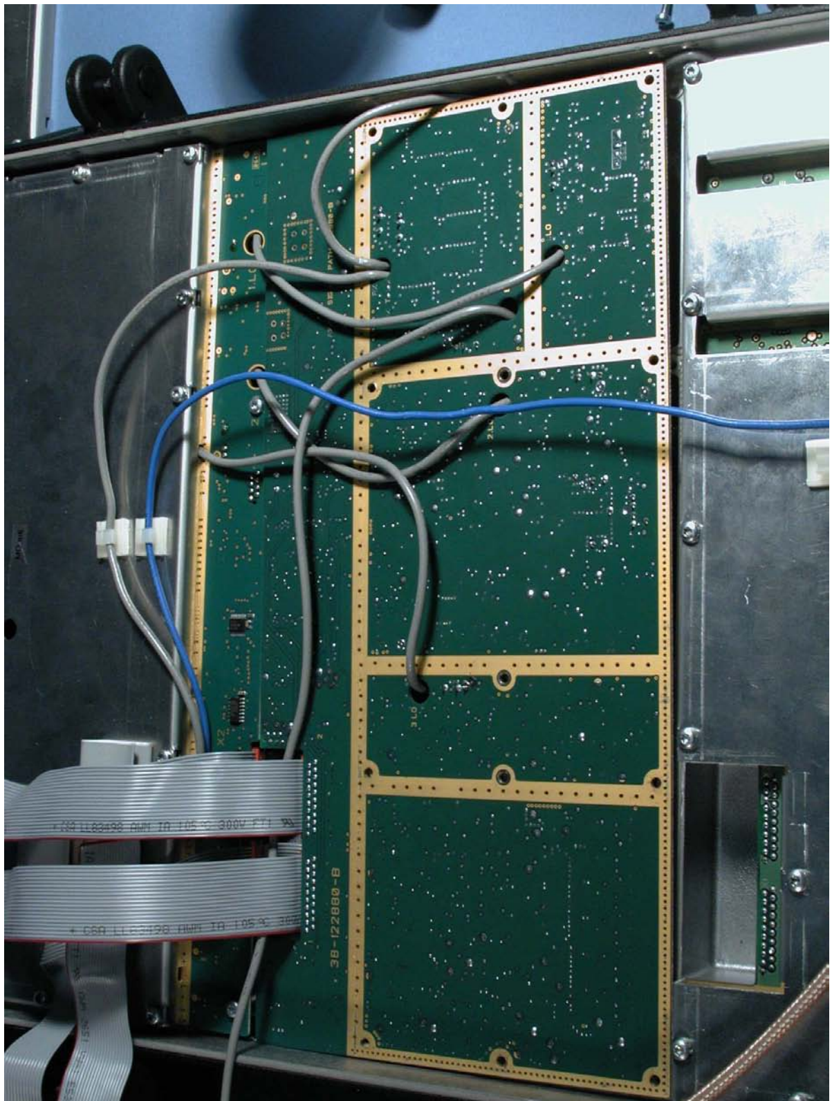
Photograph 3: Transceiver unit, SAILOR TU5160, Rx/Ex Signal Path 122880 Module
