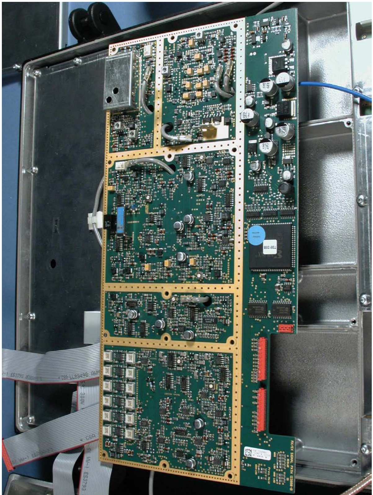
Photograph 6: Transceiver unit, SAILOR TU5160, Synth. and DSC WR 122879 Module
