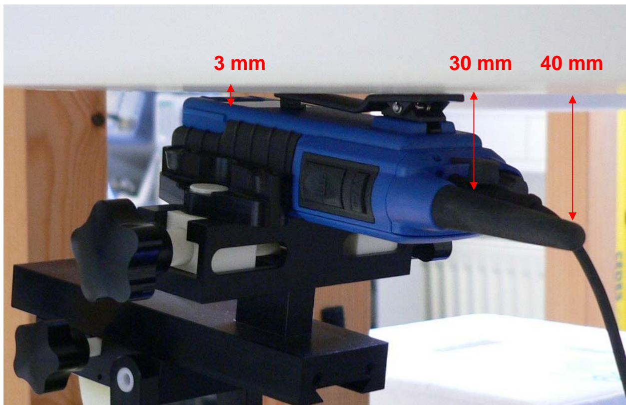
Fig. 18: Body worn with belt clip and headset.
