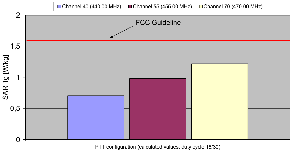
Fig. 8: The calculated SAR values in PTT configuration for the Thrane & Thrane SAILOR SP3560 in comparison to the FCC exposure limit.
