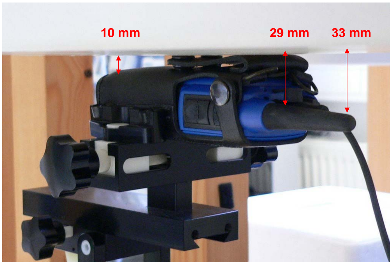
Fig. 19: Body worn with leather case and headset, display towards the ground.
