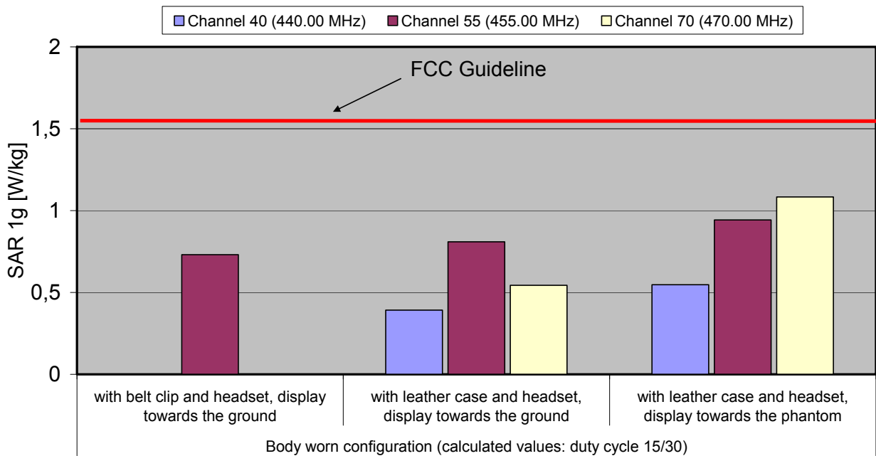
Fig. 9: The calculated SAR values in body worn configuration the Thrane & Thrane SAILOR SP3560 in comparison to the FCC exposure limit.
