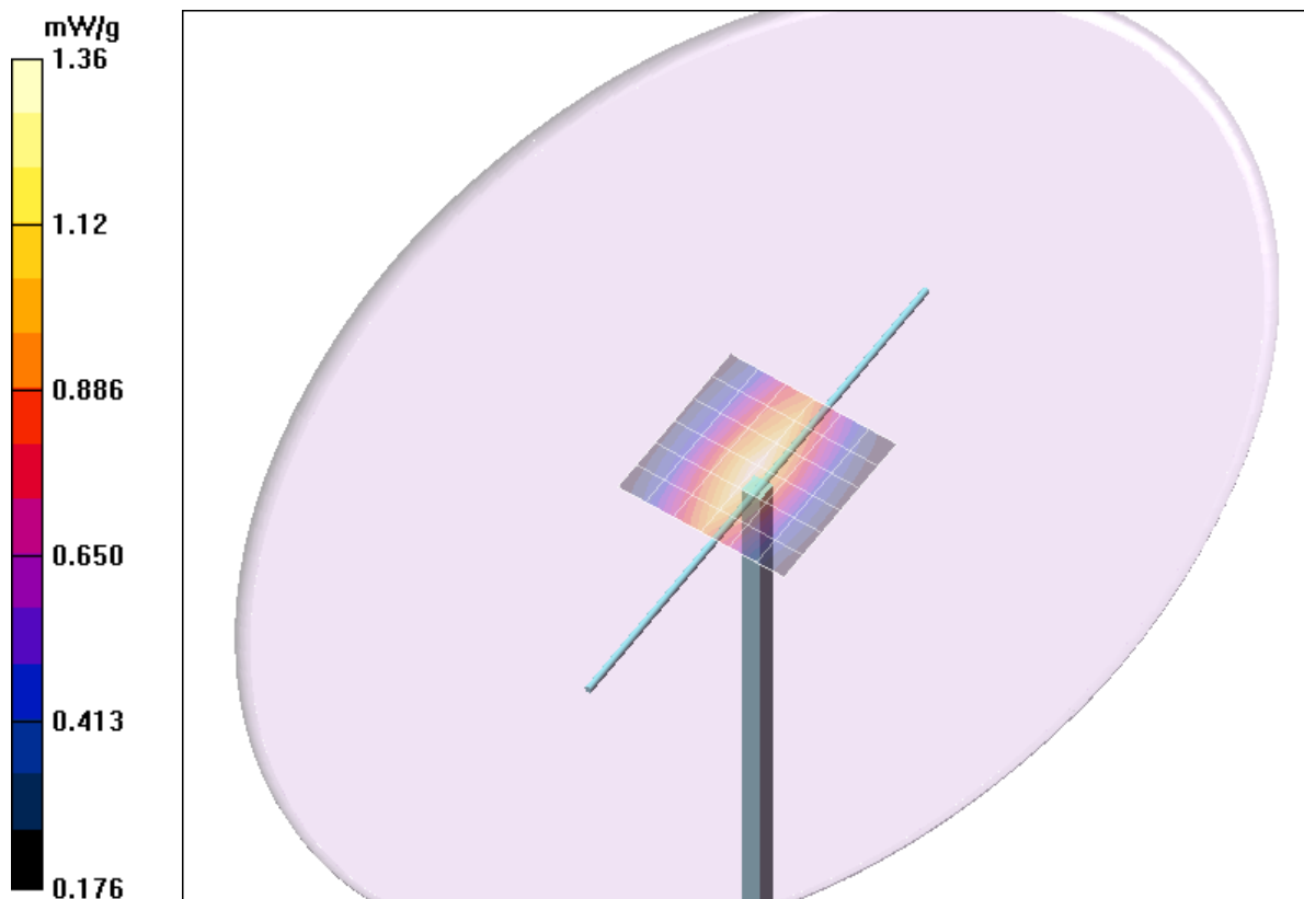
Fig. 10: Validation measurement 450 MHz Head (November 14, 2008), coarse grid. Ambient Temperature: 21.5° C, Liquid Temperature: 20.7° C.
