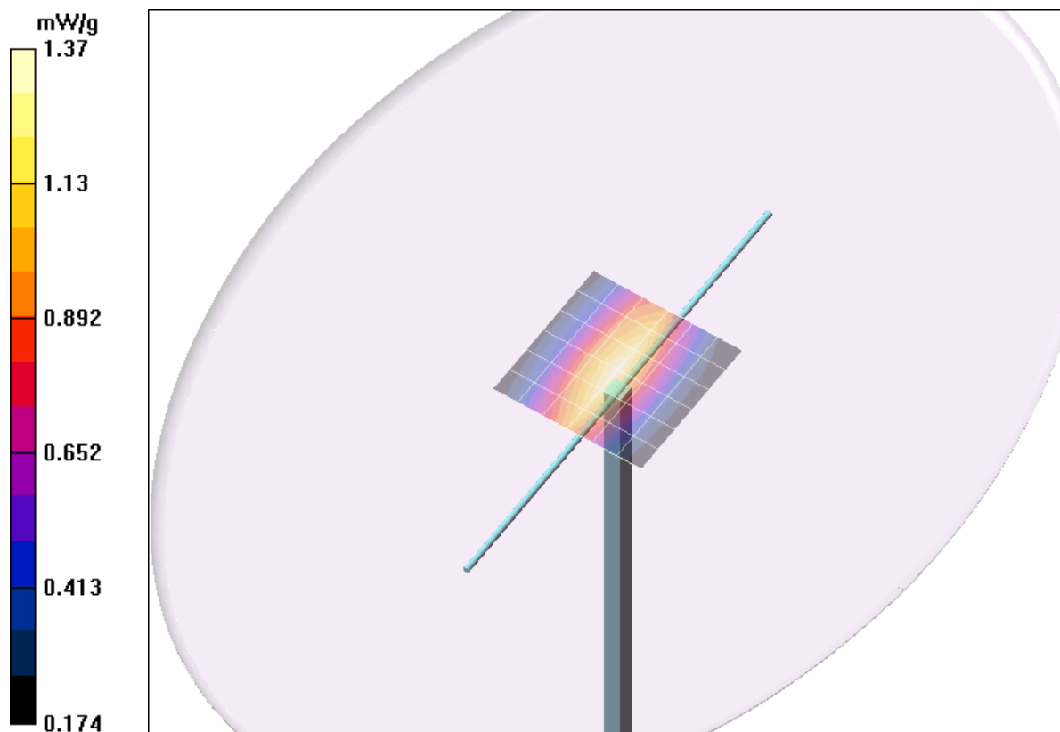
Fig. 11: Validation measurement 450 MHz body (November 13, 2008), coarse grid. Ambient Temperature: 21.6° C, Liquid Temperature: 20.8° C.
