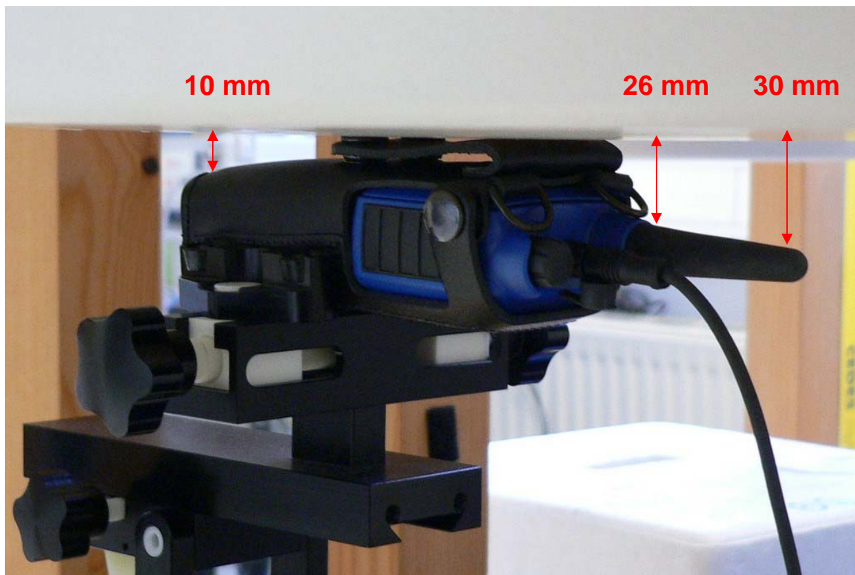
Fig. 20: Body worn with leather case, display towards the phantom.
