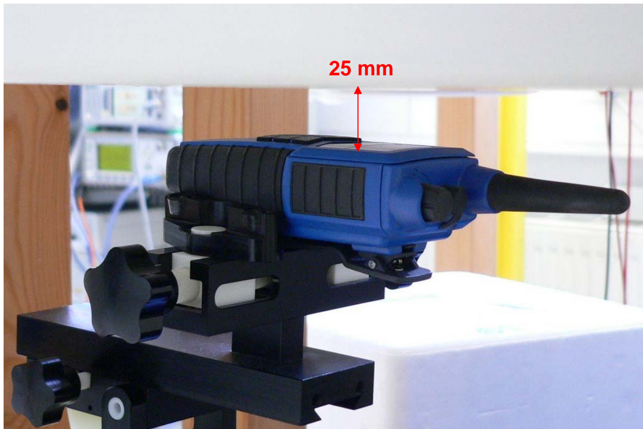
Fig. 17: PTT configuration, 25 mm distance.
