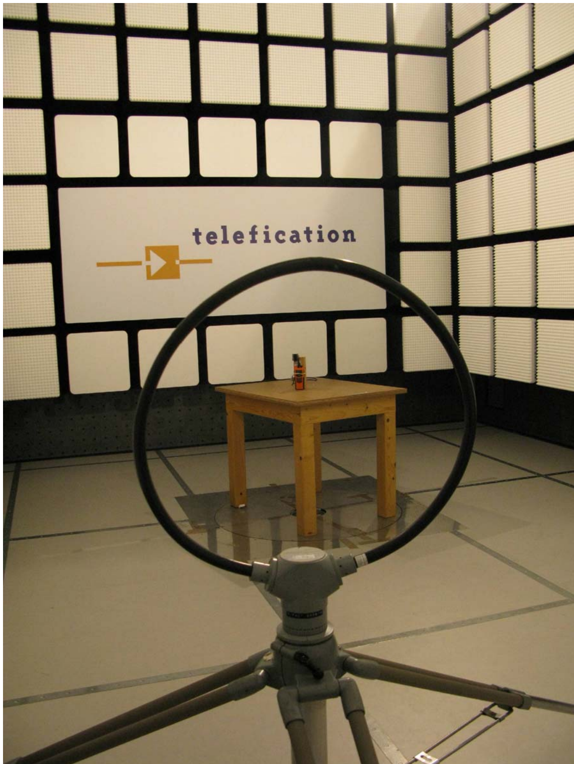
Photograph 2: Test setup cabinet radiation ( \leq 30 MHz)
