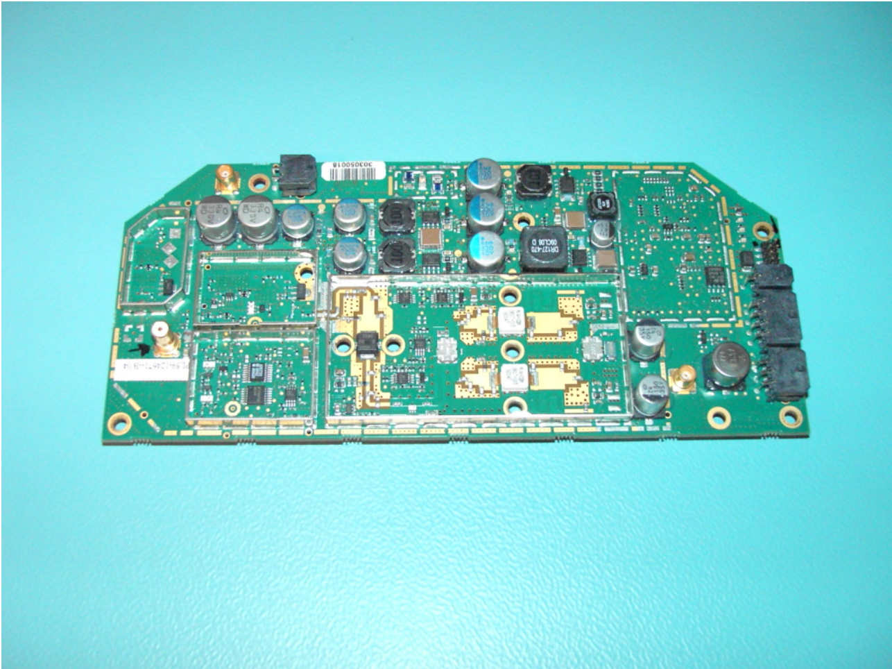
Figur 3 HPA LNA Board
