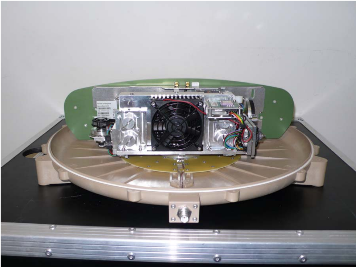
Figur 7 Without Radome 3
