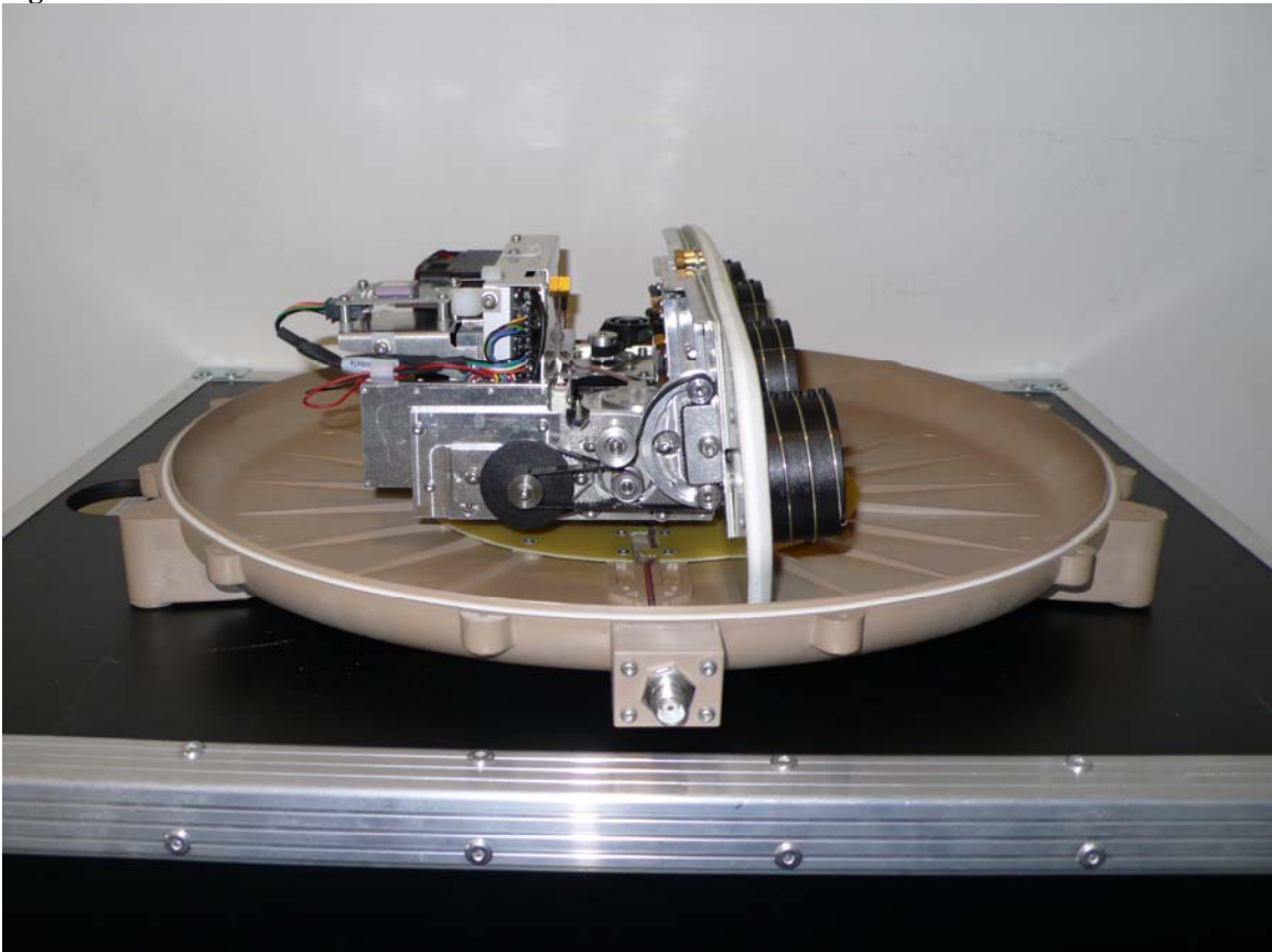
Figur 8 Without Radome 4
