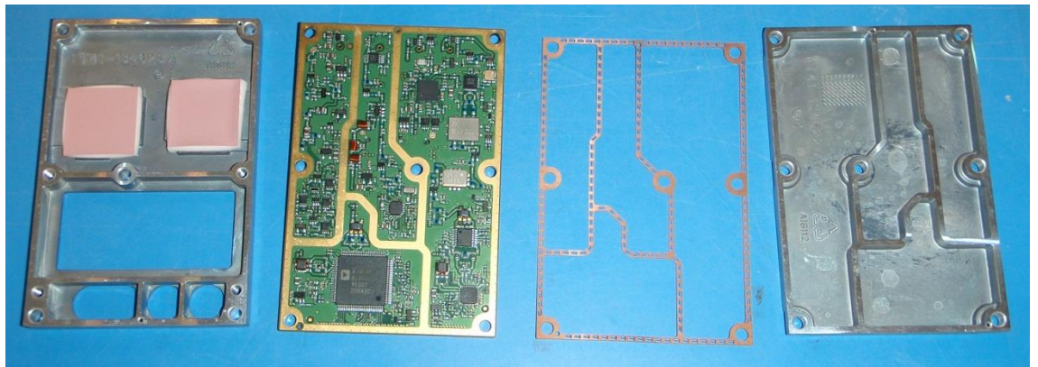
Figure 13 Explore 710 Radio Module TT3750A
