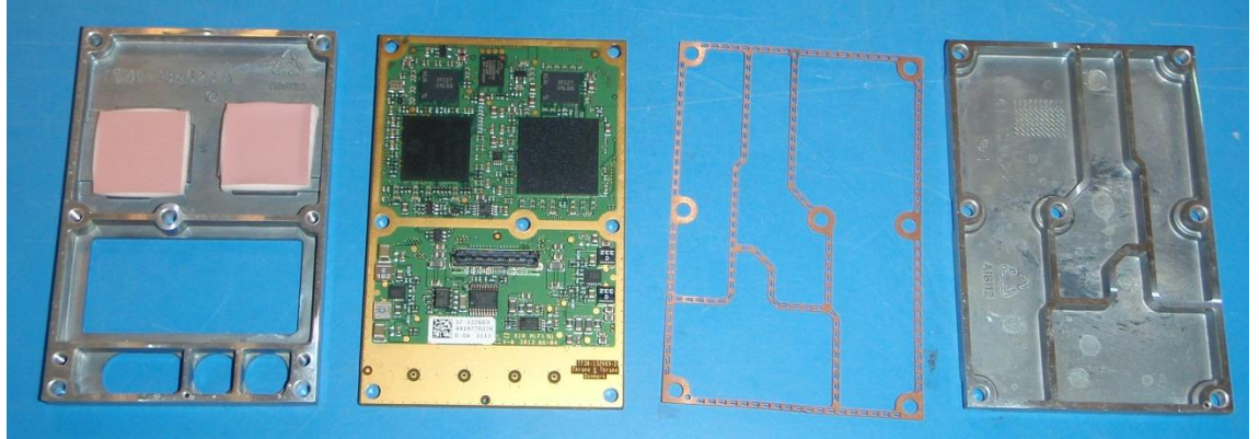
Figure 12 Explore 710 Radio Module TT3750A
