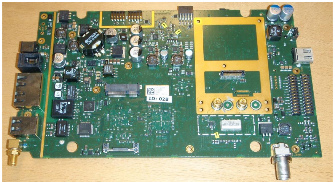
Figure 11 Explore 710 Transceiver unit TT-3732B, PCB top, no covers
