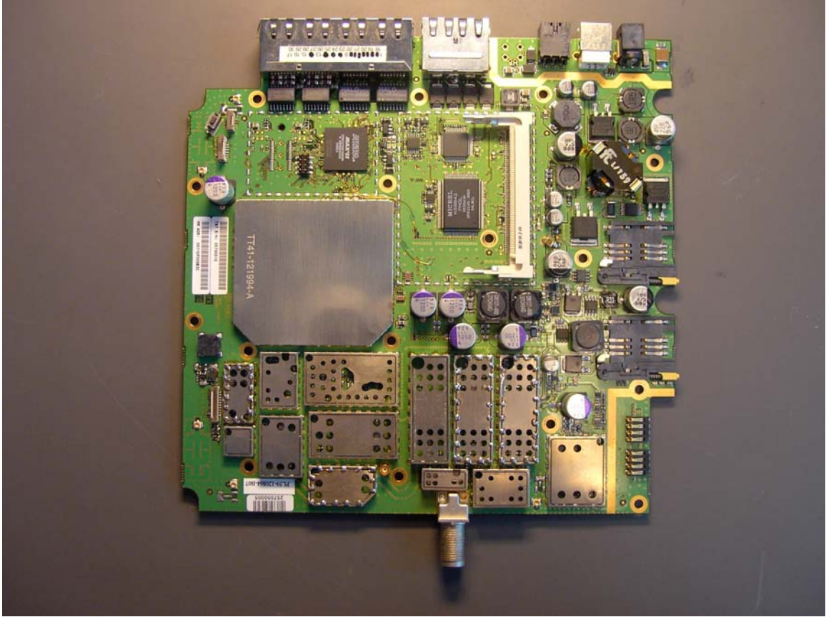
Figure 5 Transceiver Module with shields
