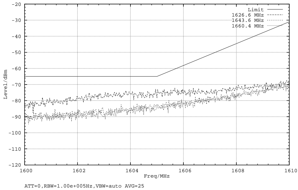
Plot 4, Mod: R20T45Q, Subtype: R, Tamb: +25DegC, Passed
