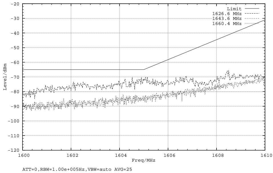
Plot 4, Mod: R5T2X, Subtype: H6, Tamb: +25DegC, Passed
