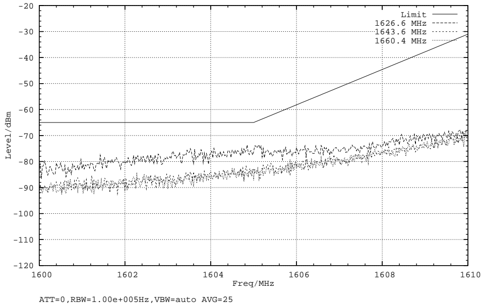
Plot 4, Mod: R20T05Q, Subtype: R, Tamb: +25DegC, Passed
