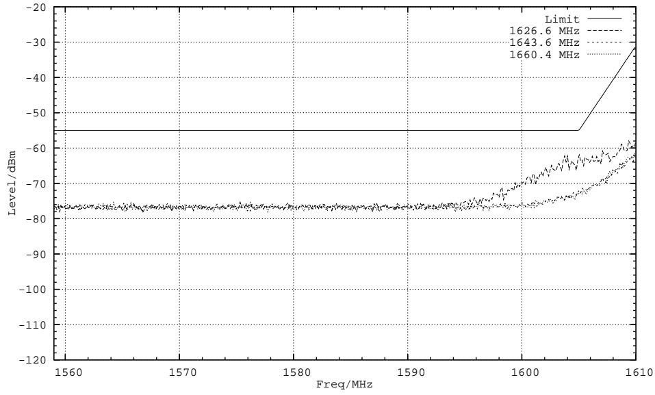
Plot 6, Mod: R5T1X, Subtype: H6, Tamb: +25DegC, Passed
