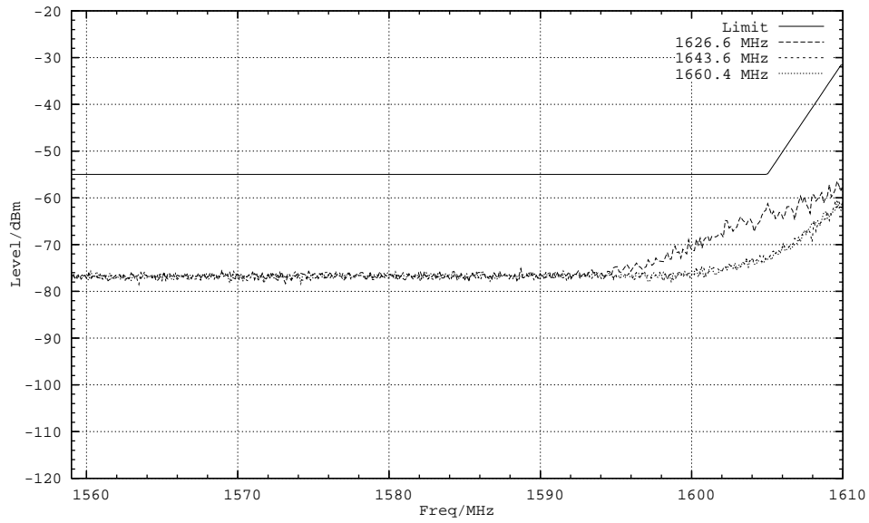
Plot 6, Mod: R20T1X, Subtype: H6, Tamb: +25DegC, Passed
