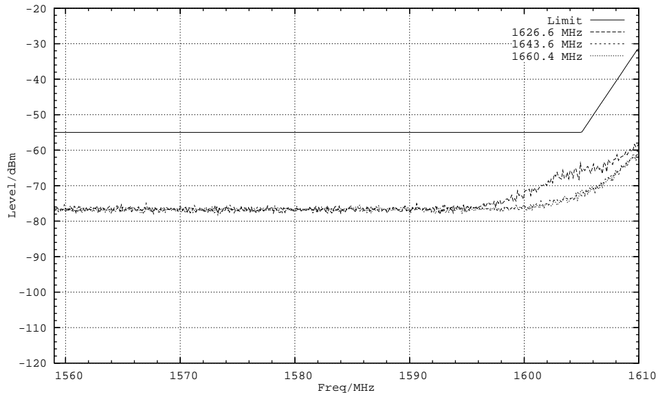
Plot 6, Mod: R20T45Q, Subtype: R, Tamb: +25DegC, Passed
