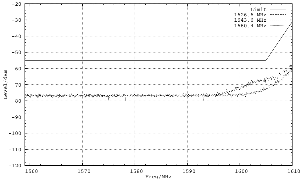
Plot 6, Mod: R5T2Q, Subtype: R, Tamb: +25DegC, Passed
