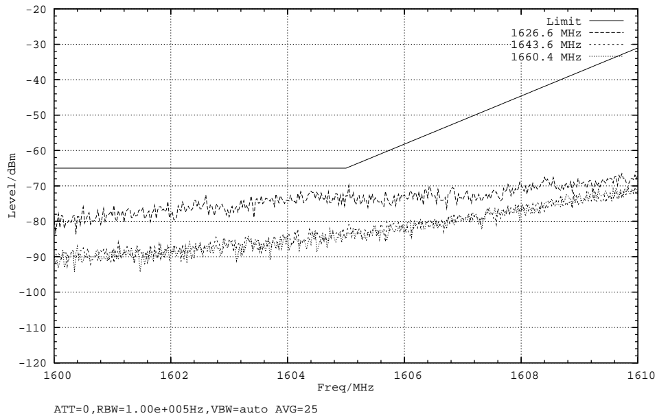
Plot 4, Mod: R20T2X, Subtype: H6, Tamb: +25DegC, Passed
