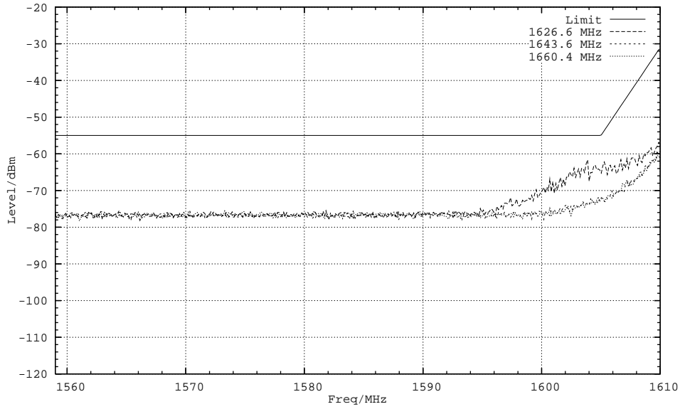
Plot 6, Mod: R20T2X, Subtype: H6, Tamb: +25DegC, Passed
