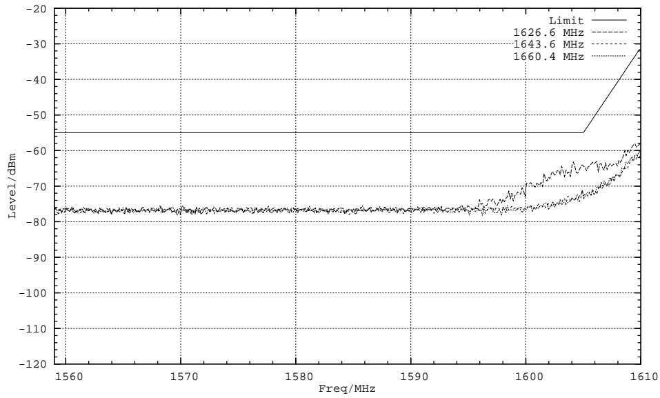
Plot 6, Mod: R20T4.5X, Subtype: H6, Tamb: +25DegC, Passed
