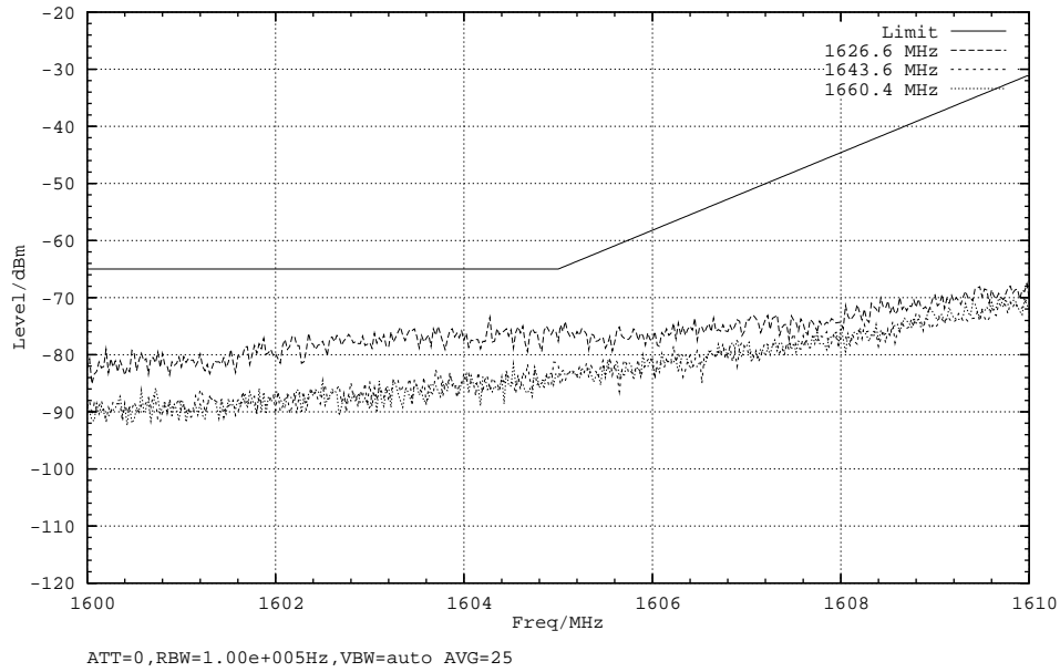
Plot 4, Mod: R5T4.5Q, Subtype: R, Tamb: +25DegC, Passed
