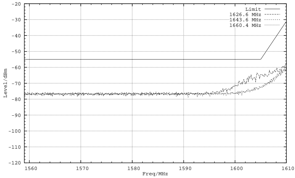
Plot 6, Mod: R20T1Q, Subtype: H1, Tamb: +25DegC, Passed
