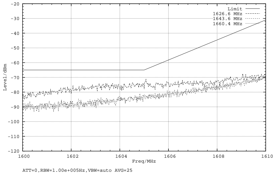
Plot 4, Mod: R20T2Q, Subtype: H1, Tamb: +25DegC, Passed
