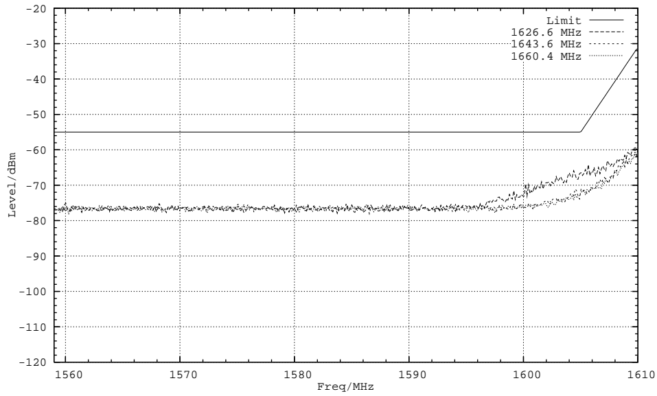
Plot 6, Mod: R5T4.5Q, Subtype: R, Tamb: +25DegC, Passed
