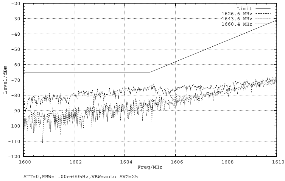
Plot 4, Mod: R5T2Q, Subtype: R, Tamb: +25DegC, Passed
