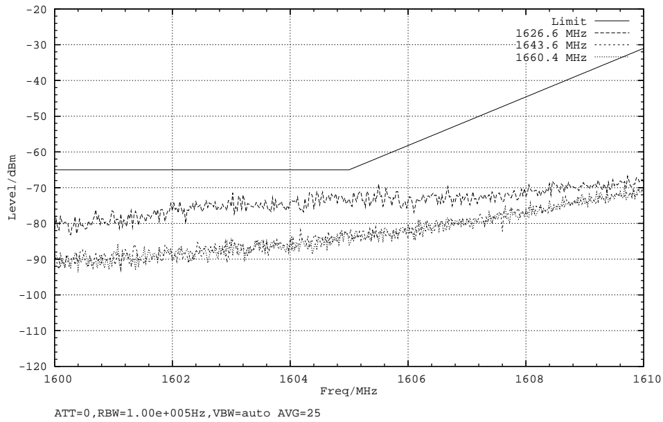
Plot 4, Mod: R20T4.5X, Subtype: H6, Tamb: +25DegC, Passed
