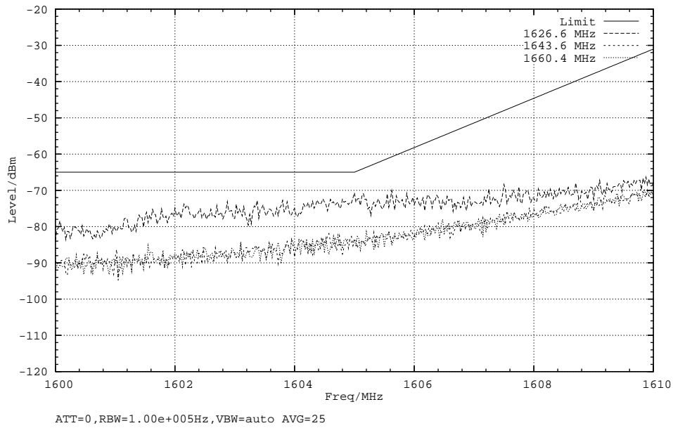
Plot 4, Mod: R20T1X, Subtype: H6, Tamb: +25DegC, Passed
