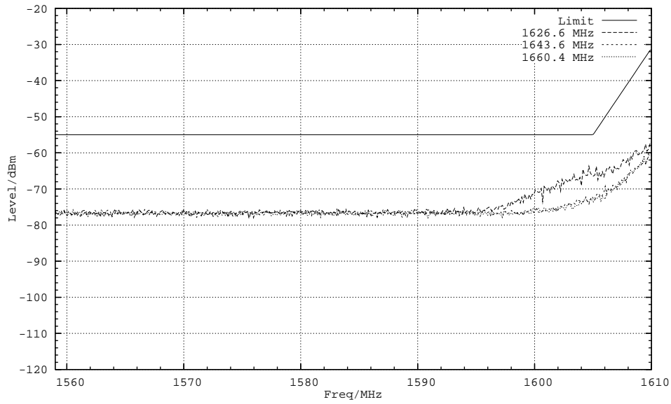
Plot 6, Mod: R20T2Q, Subtype: H1, Tamb: +25DegC, Passed
