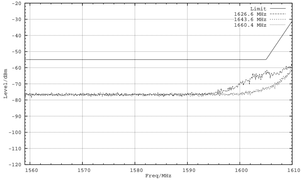
Plot 6, Mod: R5T2X, Subtype: H6, Tamb: +25DegC, Passed
