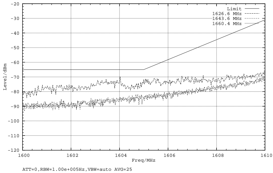
Plot 4, Mod: R5T1X, Subtype: H6, Tamb: +25DegC, Passed
