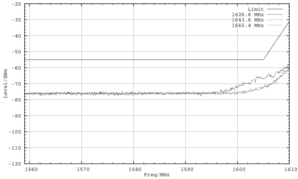
Plot 6, Mod: R20T05Q, Subtype: R, Tamb: +25DegC, Passed
