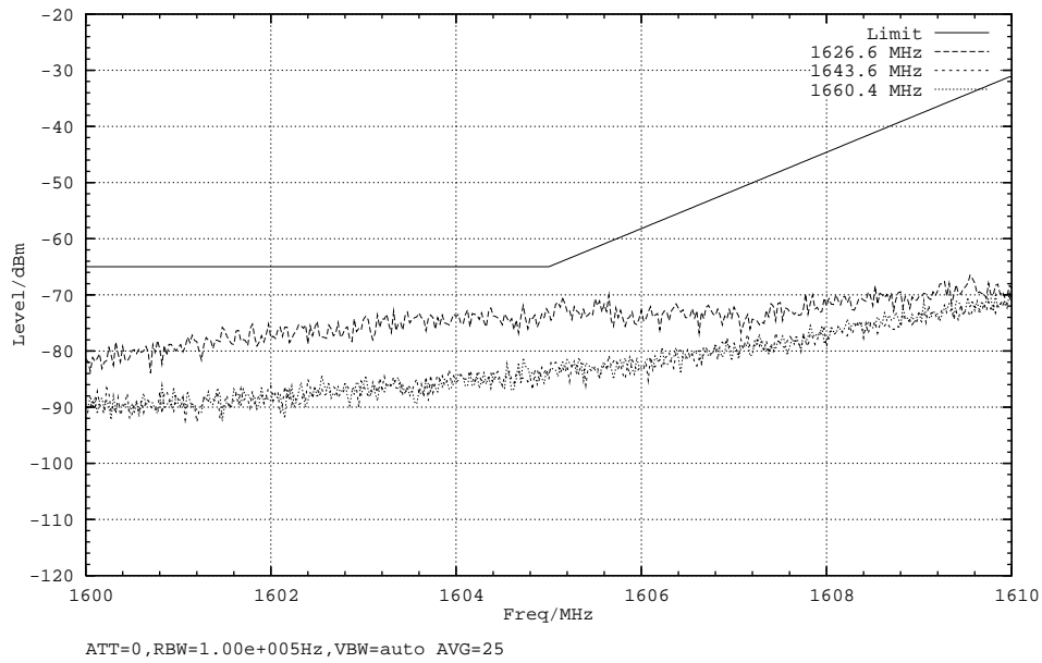
Plot 4, Mod: R5T4.5X, Subtype: H6, Tamb: +25DegC, Passed
