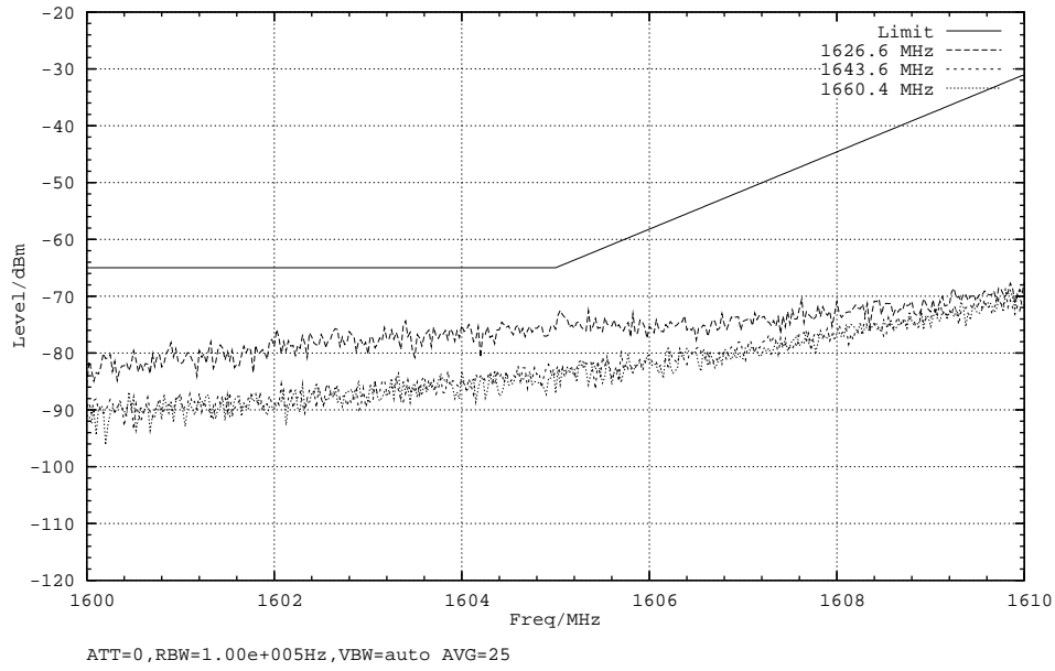
Plot 4, Mod: R20T1Q, Subtype: H1, Tamb: +25DegC, Passed
