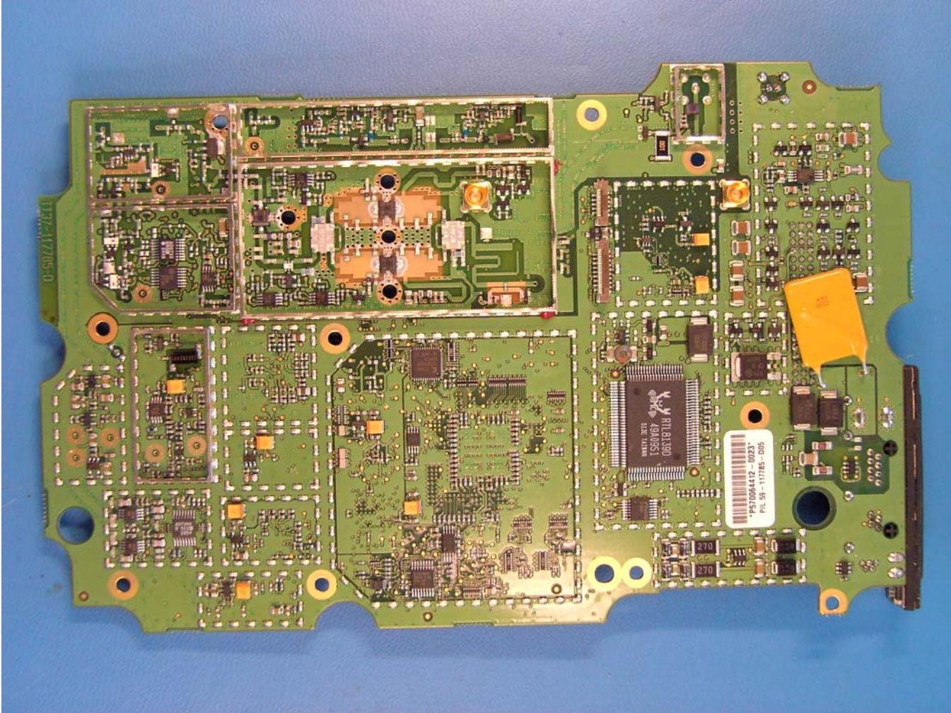
Figure 5 Mainboard
