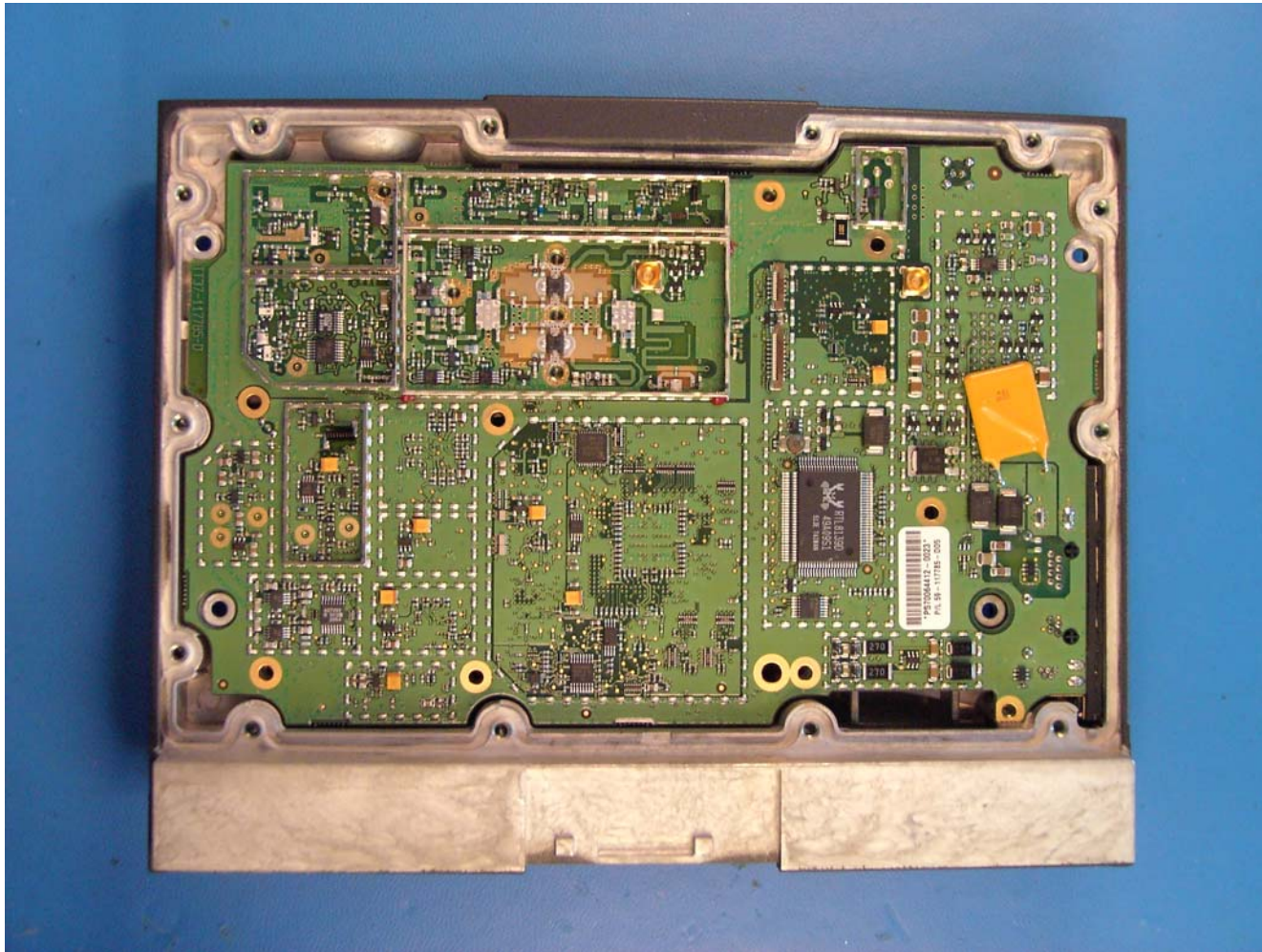
Figure 1 Mainboard
