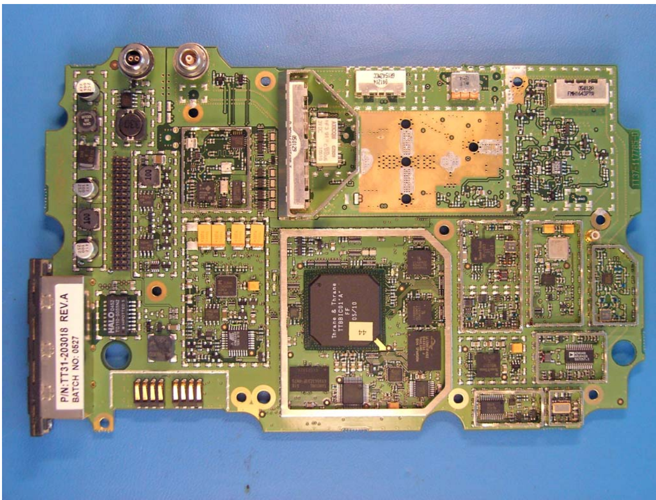
Figure 4 Mainboard
