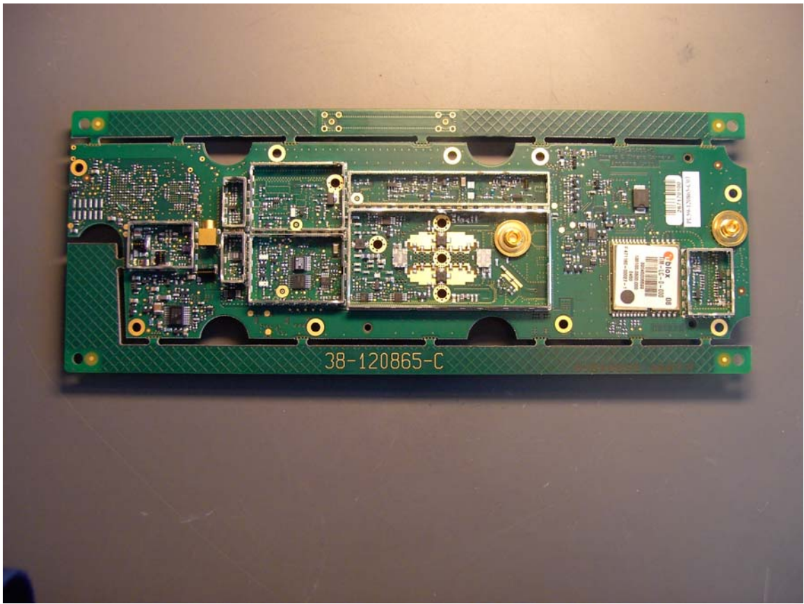
Figure 4 Frontend Module without shields
