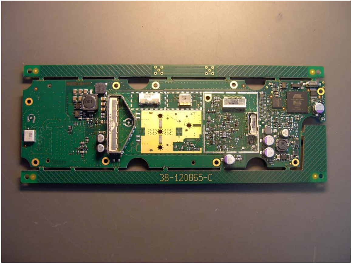
Figure 3 Frontend Module without shields
