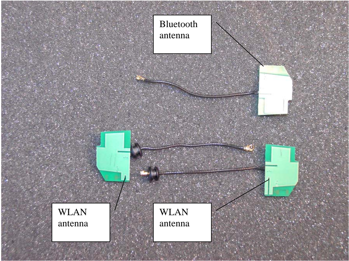
Figure 13 Bluetooth and WLAN antennas
