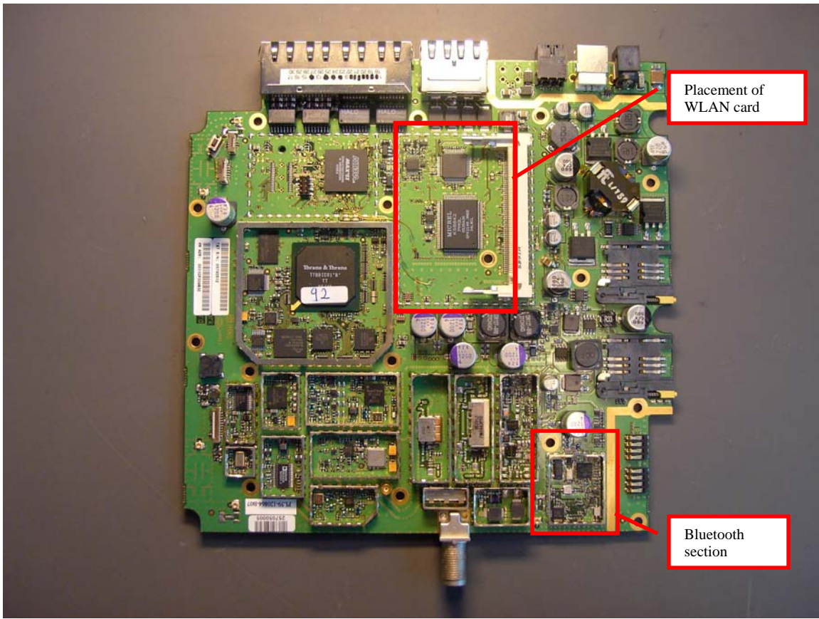
Figure 7 Transceiver Module without shields
