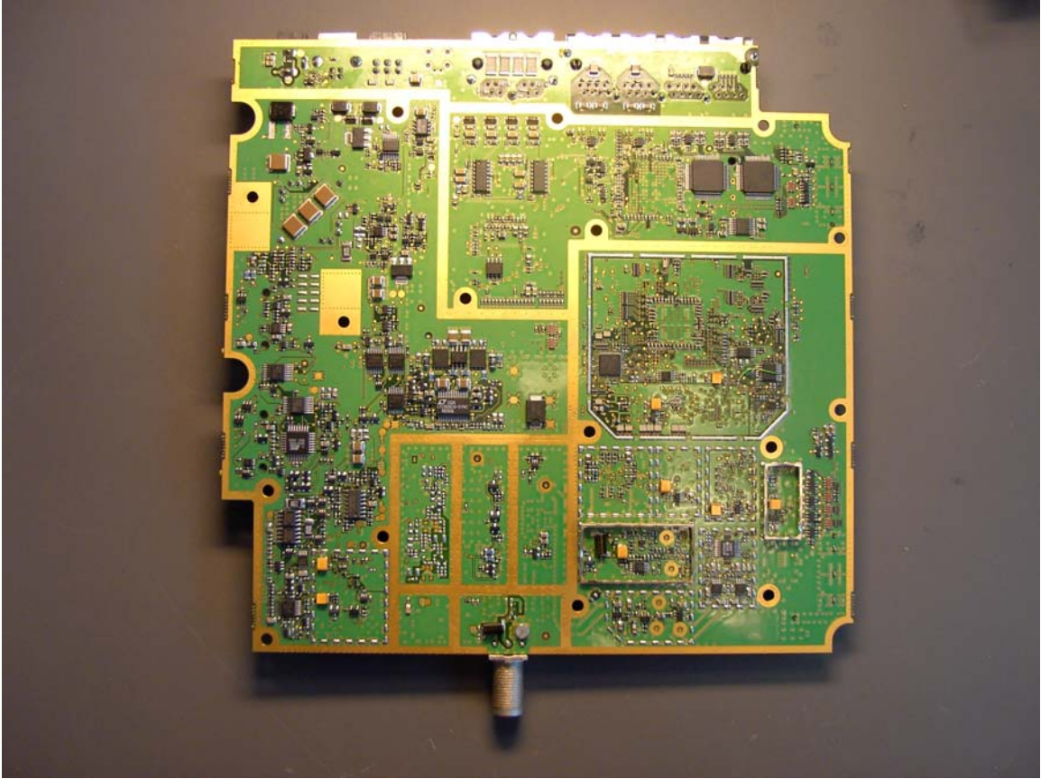
Figure 8 Transceiver Module without shields
