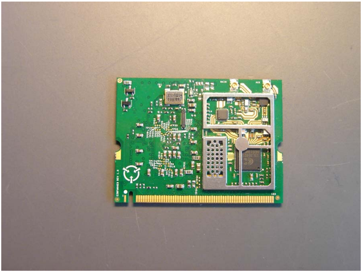
Figure 10 WLAN card without shield
