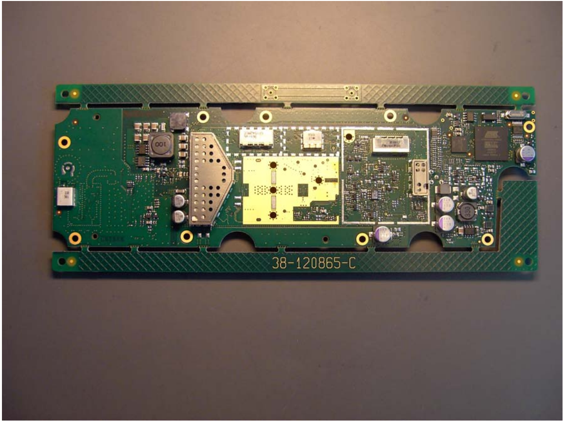
Figure 2 Frontend Module with shields
