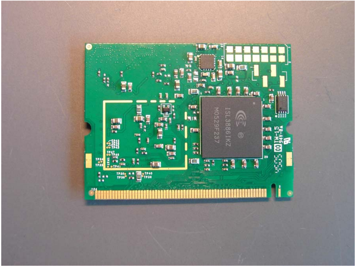
Figure 11 WLAN card
