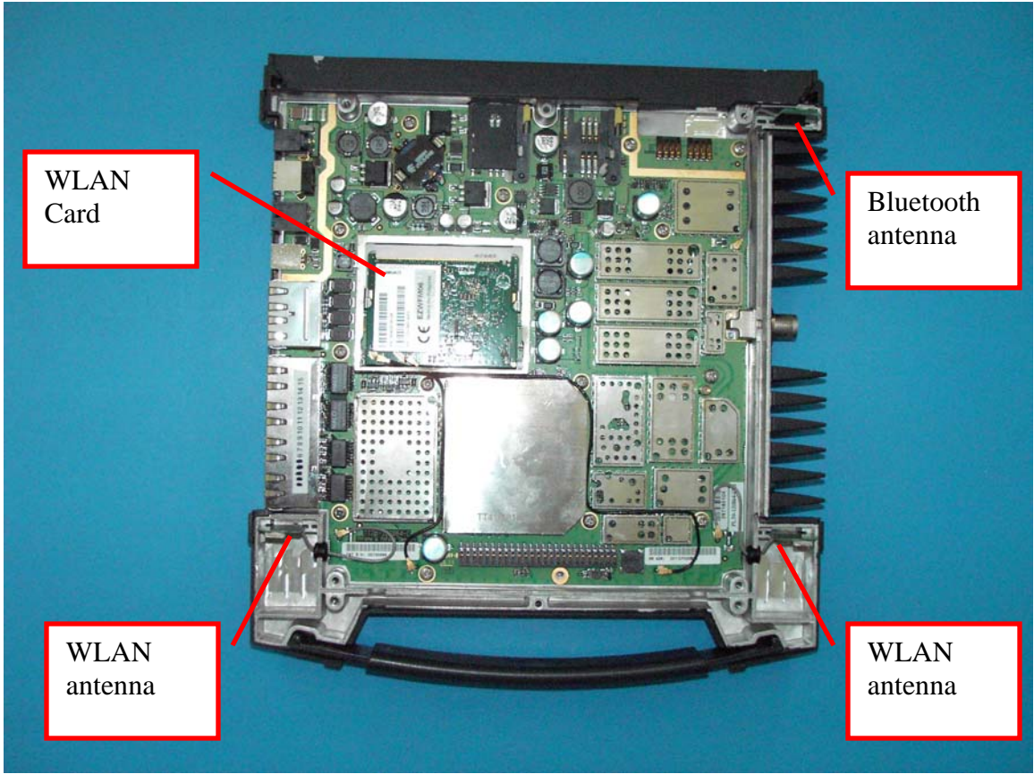
Figure 12 Transceiver and WLAN boards in the Transceiver Unit
