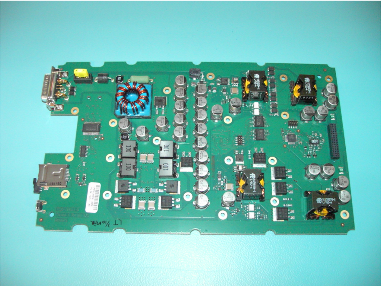
Figur 1 PSM board
