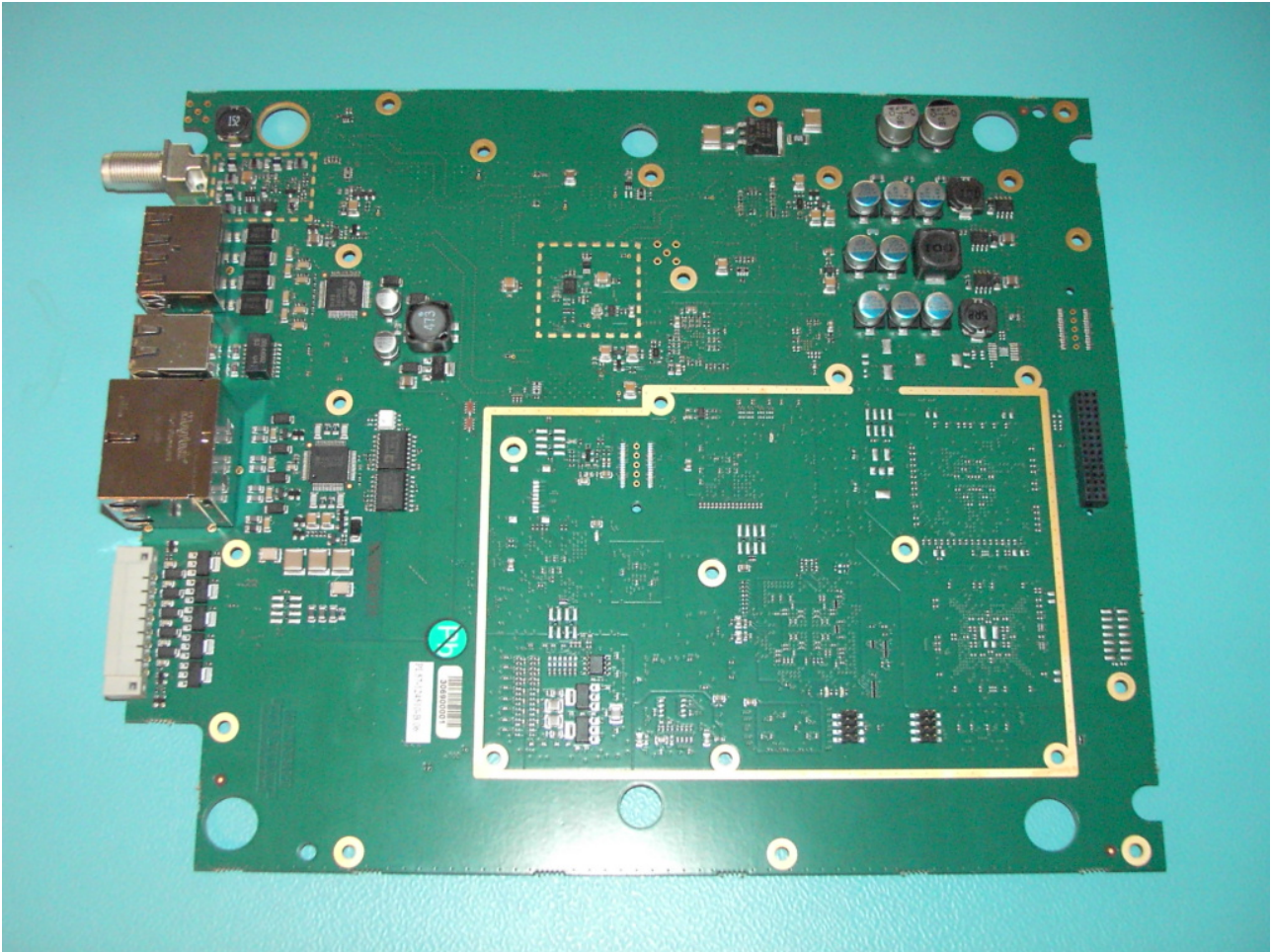
Figur 3 MainBoard
